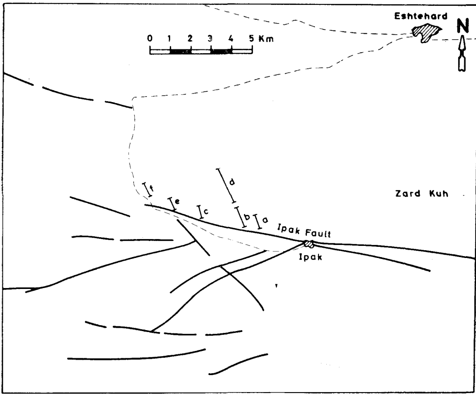
Fig. 4. Position of structural sections near Ipak (faults after Soder, 1958).
