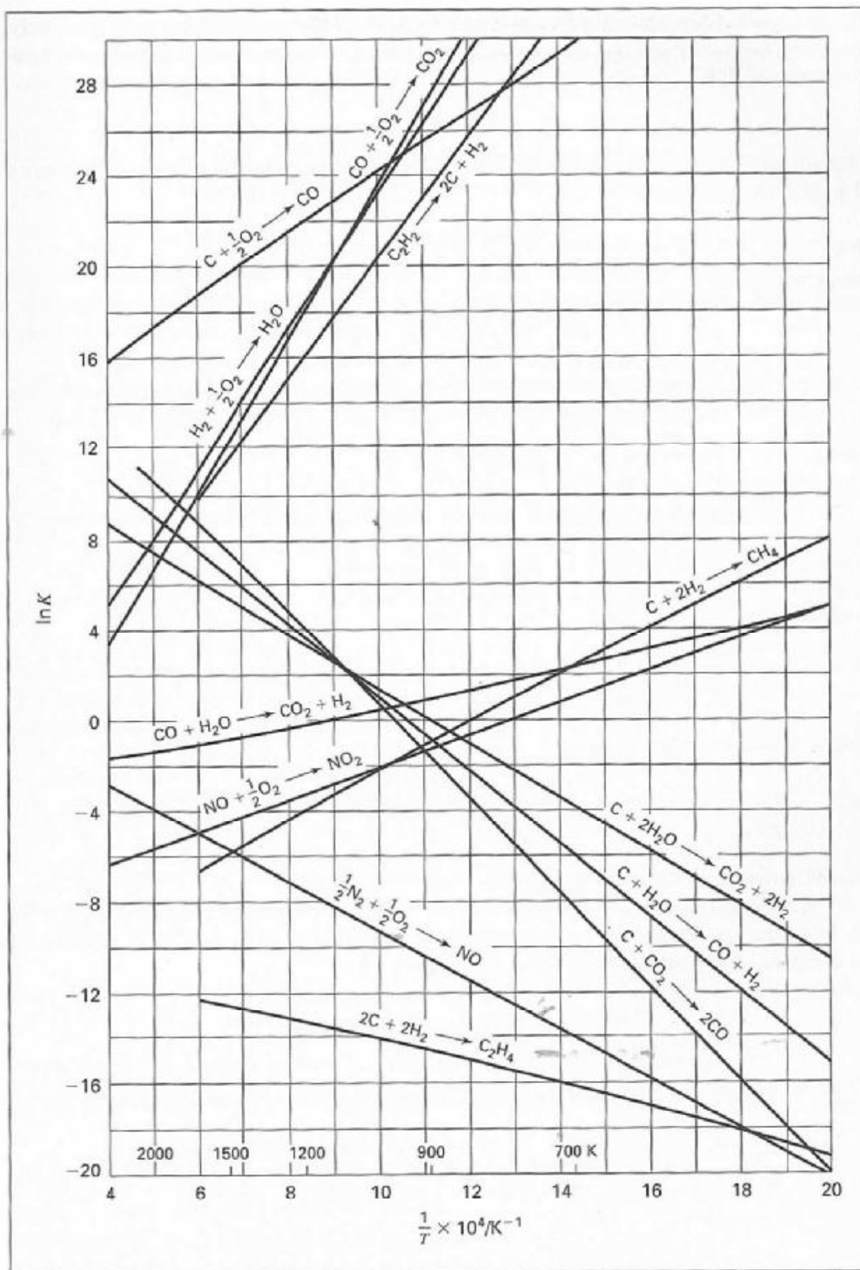
Figure 13.2: Equilibrium constants as a function of temperature.
