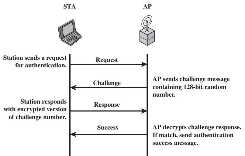
Figure 6.23 WEP Authentication
