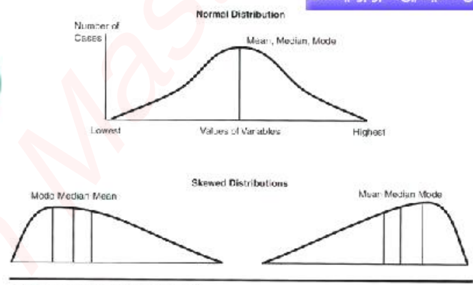
FIGURE 12.5 Measures of Central Tendency
