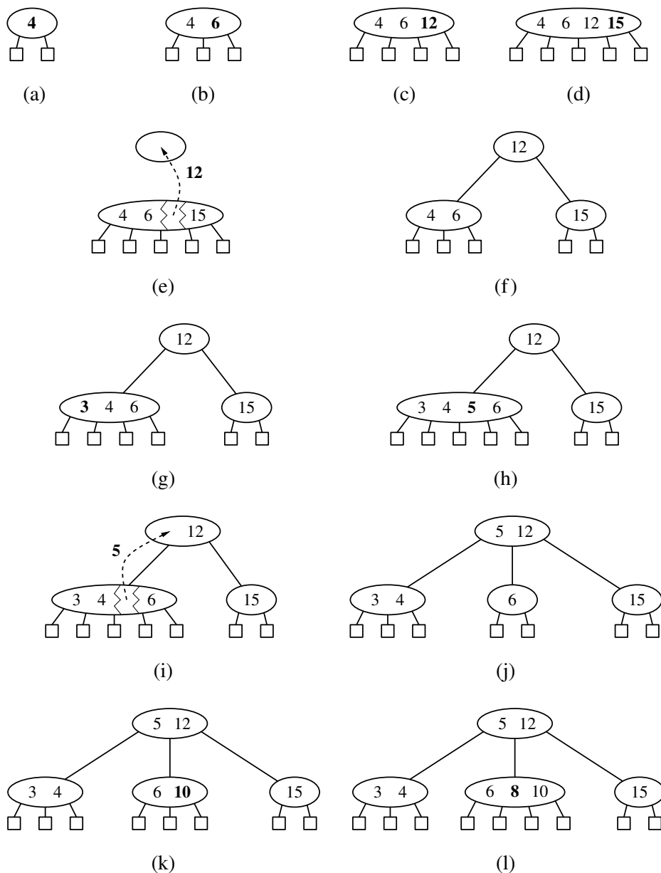
Figure 11.27: A sequence of insertions into a (2,4) tree: (a) initial tree with one item; (b) insertion of 6; (c) insertion of 12; (d) insertion of 15, which causes an overflow; (e) split, which causes the creation of a new root node; (f) after the split; (g) insertion of 3; (h) insertion of 5, which causes an overflow; (i) split; (j) after the split; (k) insertion of 10; (l) insertion of 8.
