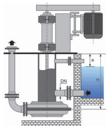
Dry Installation V330
