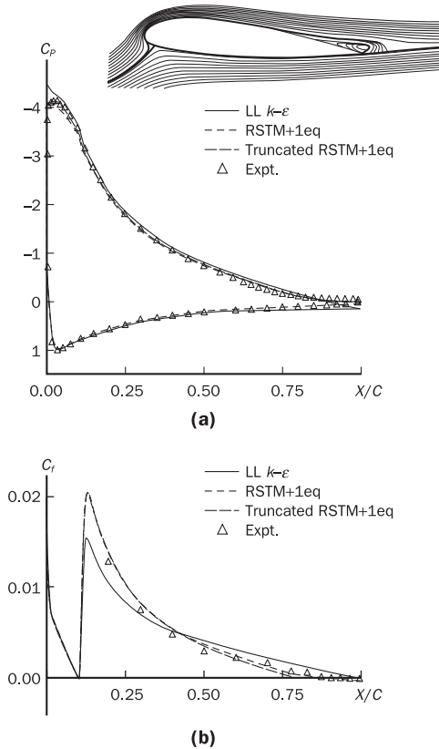
Figure 3.16 Comparison of predictions of RSM and standard k - \varepsilon model with measurements on a high-lift Aérospatiale aerofoil: (a) pressure coefficient; (b) skin friction coefficient Source: Leschziner, in Peyret and Krause (2000)
