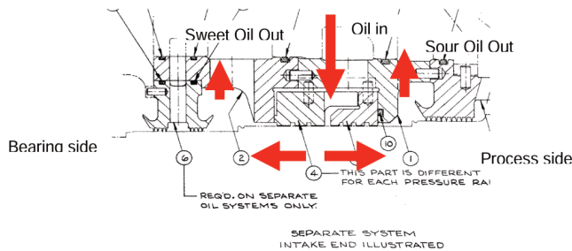
Figure 17. Oil Film Seal.
