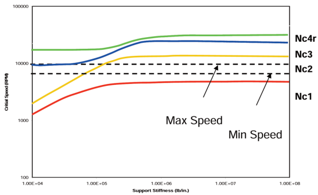
Figure 12. Critical Speed Map.
