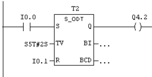
Network 1: On delay timer
