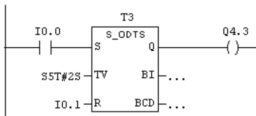
Network 1: Retentive On delay timer
