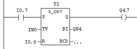
Network 1: on-delay timer with time value in memory word
