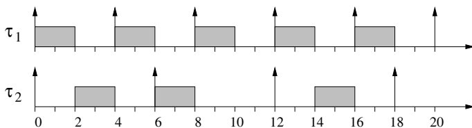
Figure 4.1 A task set with U_{ub} = 5/6 .
