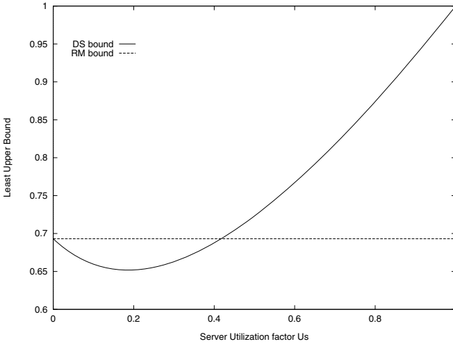
Figure 5.11 Schedulability bound for periodic tasks and DS as a function of the server utilization factor U_s .
