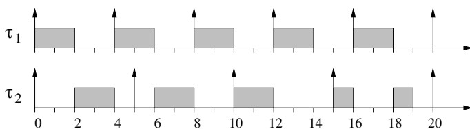
Figure 4.2 A task set with U_{ub} = 0.9 .
