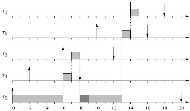
Figure 8.2 Fully preemptive scheduling can generate several preemptions (a) although only a few of them are really necessary to guarantee the schedulability of the task set (b).
