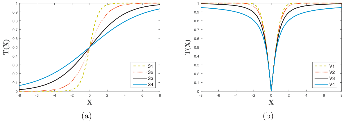
Fig. 2. Transfer functions families (a) S-shaped and (b) V-shaped.
