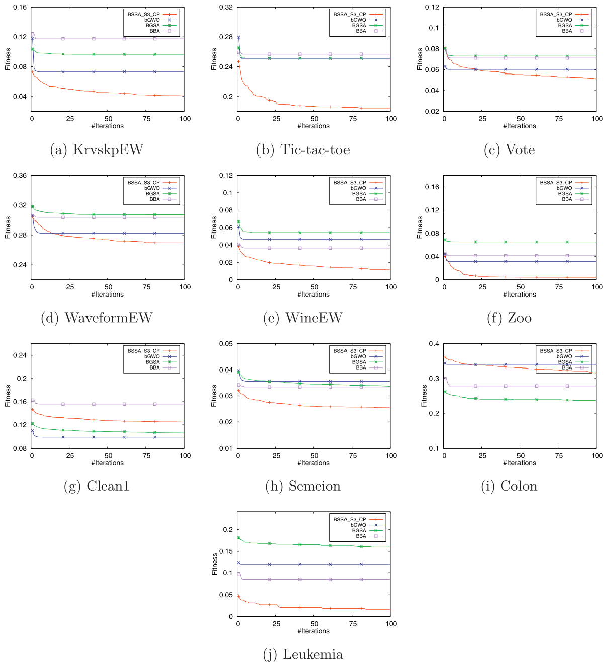
Fig. 6. Convergence curves for BSSA_S3_CP and other state-of-art methods for KrvspkEW, Tic-tac-toe, Vote, WaveformEW, WineEW, Zoo, Clean1, Semeion, Colon, and Leukemia datasets.
