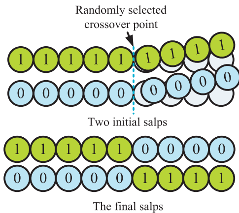
Fig. 4. The crossover process.
