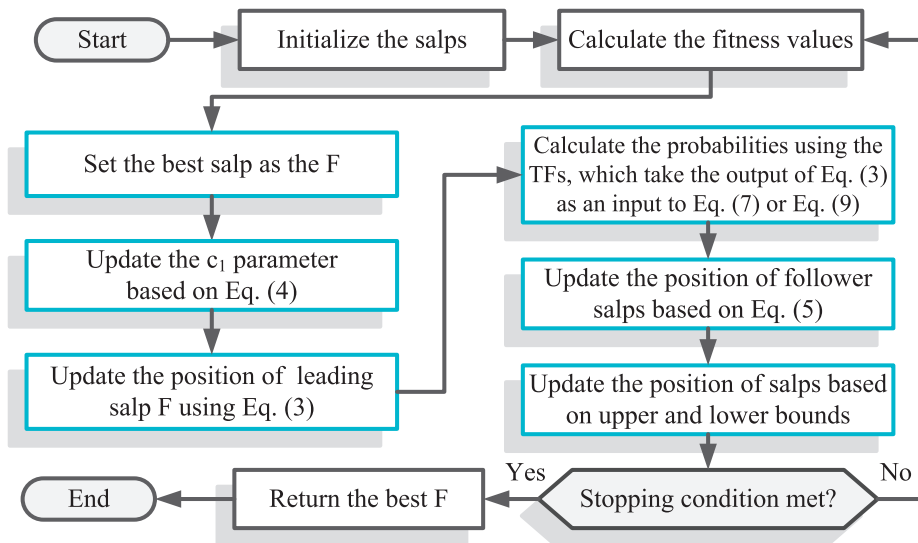
Fig. 3. The flowchart of the SSA algorithm with transfer functions.
