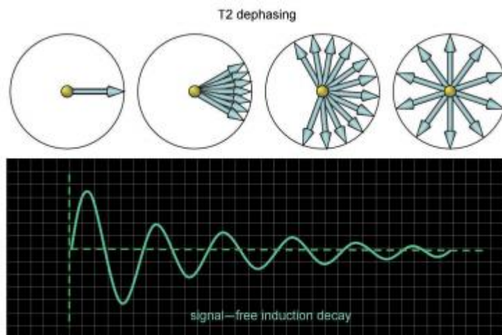
i Dephasing and free induction decay (FID).
