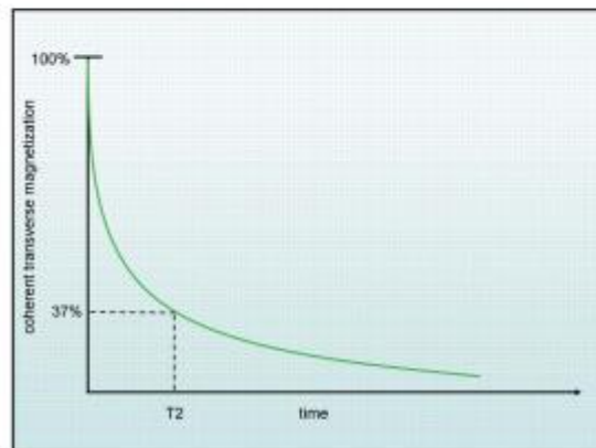
The T 2 decay curve.
