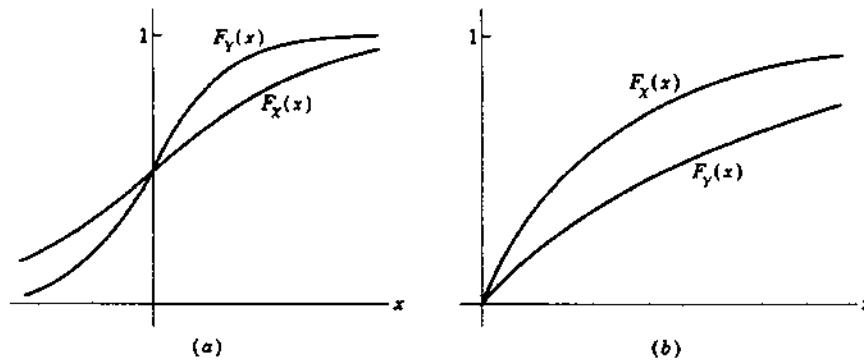
Fig. 1.1 F_Y(x) = F_X(\theta x) . (a) F_X normal, \theta > 1 ; (b) F_X exponential, \theta < 1 .
