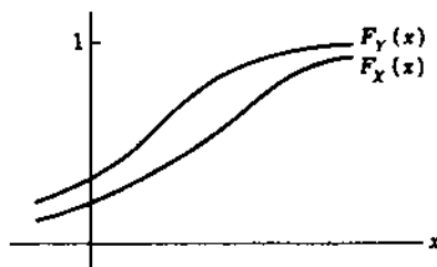
Fig. 1.2 X is stochastically larger than Y .
