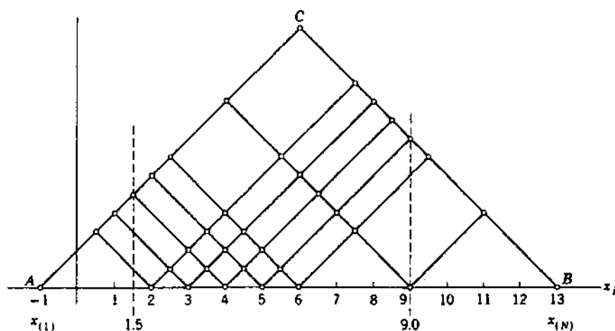
Fig. 7.2 Graphical determination of confidence interval.
