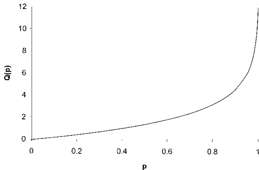
Fig. 2.2 The exponential quantile function with \beta = 2 .
