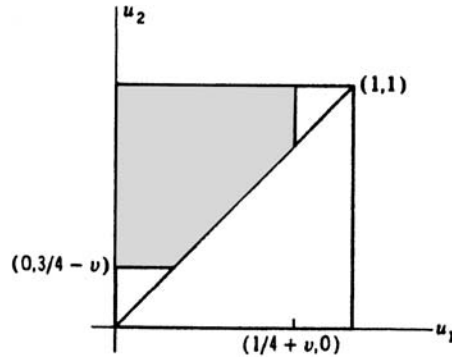
Fig. 3.1 Shaded area is region of integration for n = 2 .
