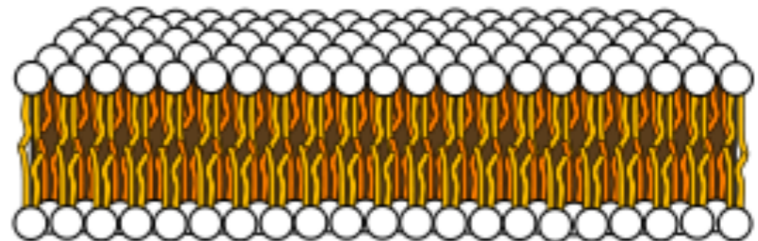
Bilayer sheet
