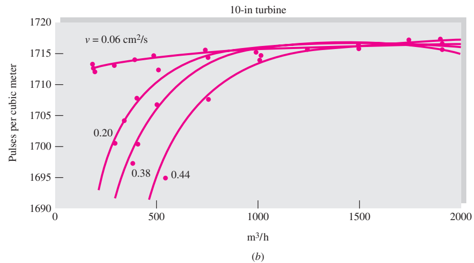
Fig. 6.32 The turbine meter widely used in the oil, gas, and water supply industries: (a) basic design; (b) typical calibration curve for a range of crude oils. ( Daniel Industries, Houston, TX. )
