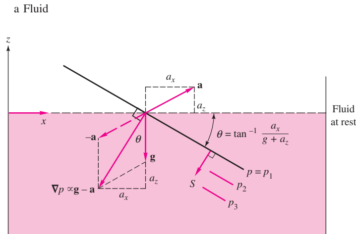
Fig. 2.21 Tilting of constant-pressure surfaces in a tank of liquid in rigid-body acceleration.
