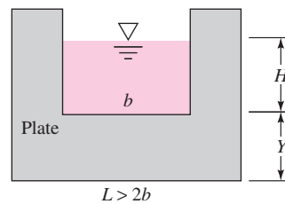
(b) Rectangle with side contractions.
