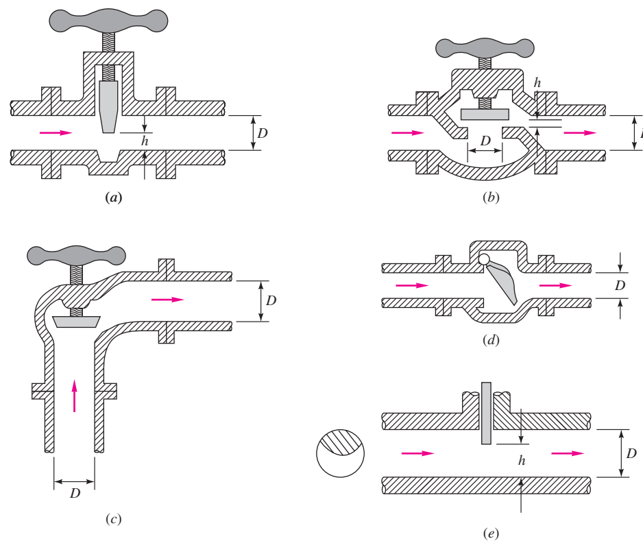
Fig. 6.17 Typical commercial valve geometries: (a) gate valve; (b) globe valve; (c) angle valve; (d) swing-check valve; (e) disk-type gate valve.
