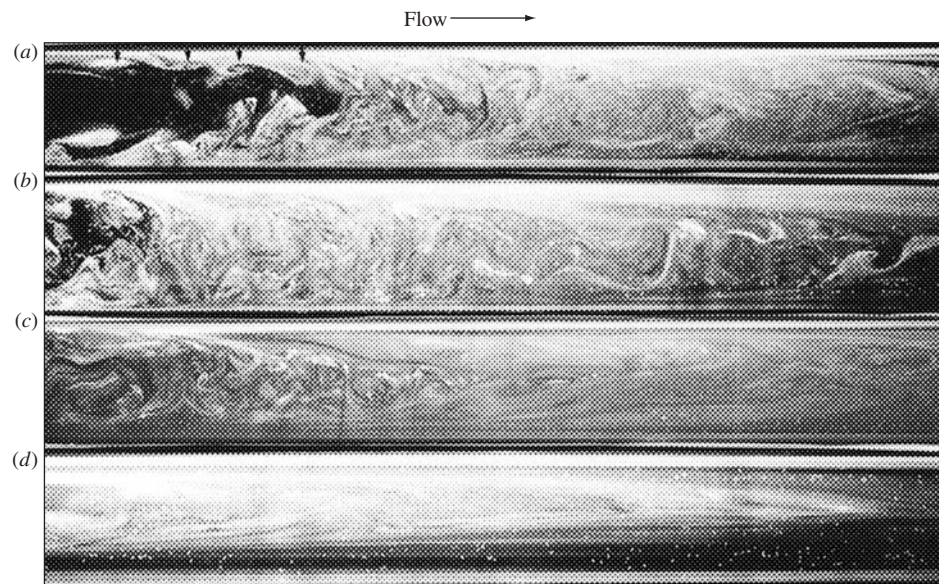
Fig. 6.3 Formation of a turbulent puff in pipe flow: (a) and (b) near the entrance; (c) somewhat downstream; (d) far downstream. (Courtesy of Cambridge University Press. P. R. Bandyopadhyay, "Aspects of the Equilibrium Puff in Transitional Pipe Flow," Journal of Fluid Mechanics , vol. 163, 1986, pp. 439-458.)
