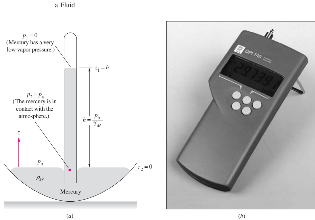
Fig. 2.6 A barometer measures local absolute atmospheric pressure: (a) the height of a mercury column is proportional to p_{\text{atm}} ; (b) a modern portable barometer, with digital readout, uses the resonating silicon element of Fig. 2.28c. (Courtesy of Paul Lupke, Druck Inc.)
