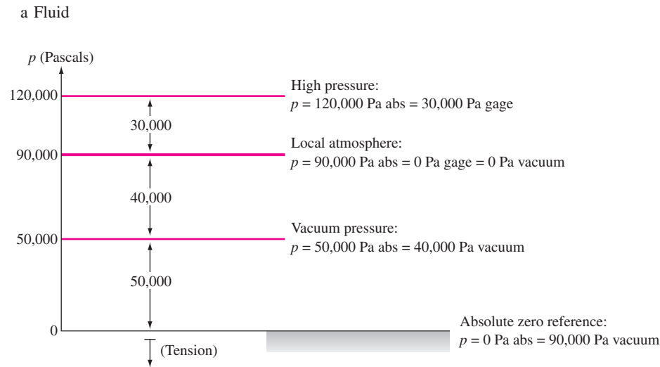
Fig. 2.3 Illustration of absolute, gage, and vacuum pressure readings.
