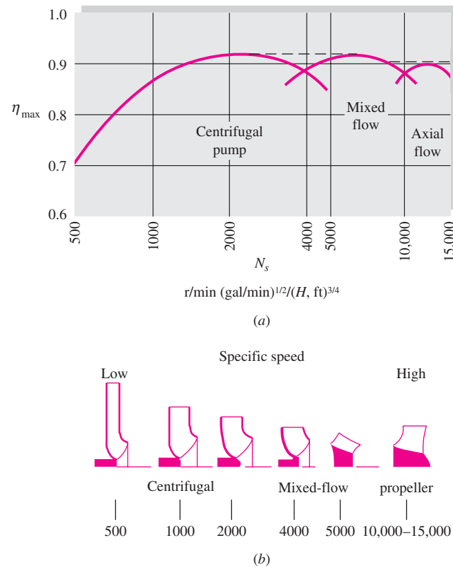
Fig. 11.11 (a) Optimum efficiency and (b) vane design of dynamic pump families as a function of specific speed.
