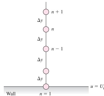
Fig. 8.39 An equally spaced finite difference mesh for one-dimensional viscous flow [Eq. (8.114)].
