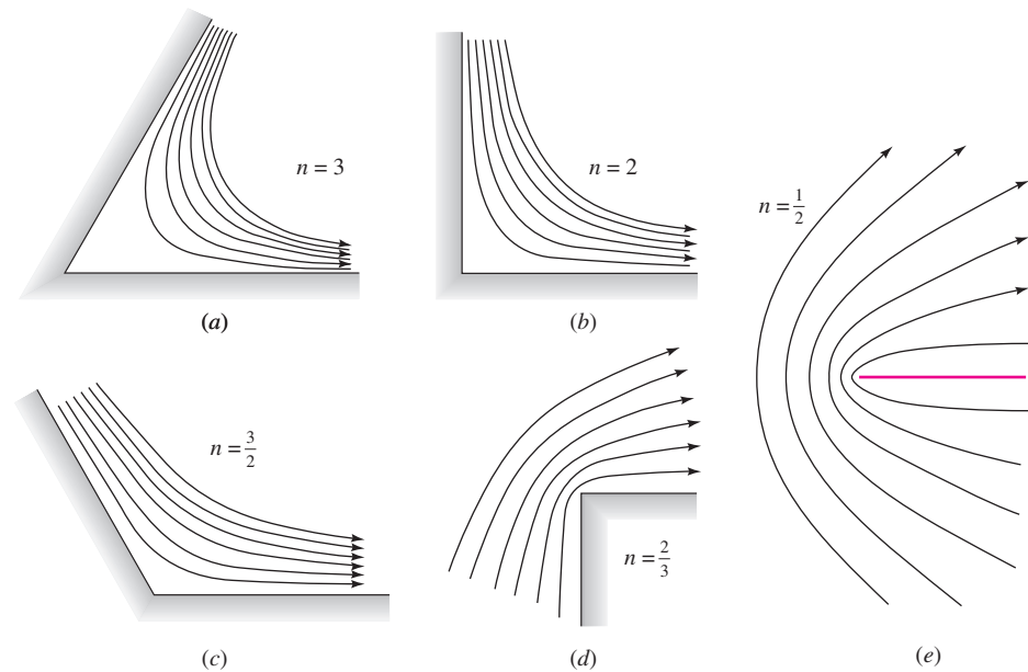
Fig. 8.18 Streamlines for corner flow, Eq. (8.53), for corner angle \beta of (a) 60^\circ , (b) 90^\circ , (c) 120^\circ , (d) 270^\circ , and (e) 360^\circ .
