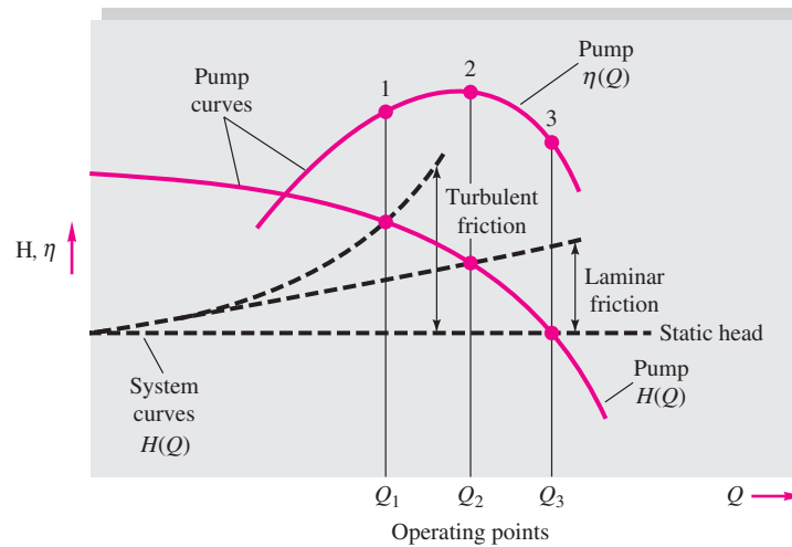
Fig. 11.18 Illustration of pump operating points for three types of system head curves.
