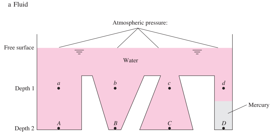
Fig. 2.4 Hydrostatic-pressure distribution. Points a, b, c, and d are at equal depths in water and therefore have identical pressures. Points A, B, and C are also at equal depths in water and have identical pressures higher than a, b, c, and d . Point D has a different pressure from A, B, and C because it is not connected to them by a water path.
