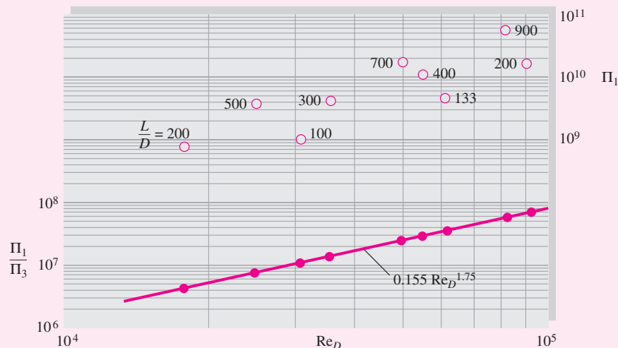
Fig. 5.10 Two different correlations of the data in Example 5.10: Open circles when plotting \rho D^2 \Delta p / \mu^2 versus Re_D , L/D is a parameter; once it is known that \Delta p is proportional to L , a replot (solid circles) of \rho D^3 \Delta p / (L \mu^2) versus Re_D collapses into a single power-law curve.
