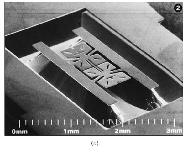
Fig. 2.28 Pressure sensors with electric output: (a) a silicon diaphragm whose deflection changes the cavity capacitance ( Courtesy of Johnson-Yokogawa Inc. ); (b) a silicon strain gage that is stressed by applied pressure; (c) a micromachined silicon element that resonates at a frequency proportional to applied pressure. [(b) and (c) are courtesy of Druck, Inc., Fairfield, CT.]
