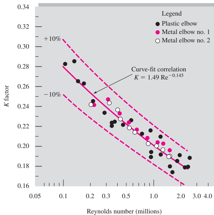
Fig. 6.18a Recent measured loss coefficients for 90° elbows. These values are less than those reported in Table 6.5. (From Ref. 48, courtesy of R. D. Coffald.)
