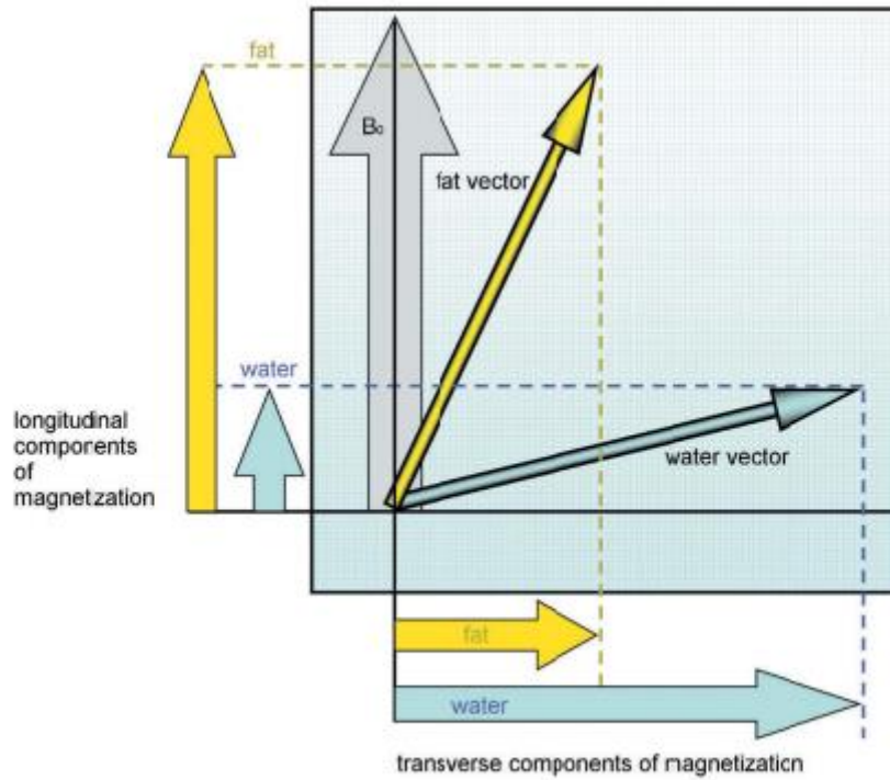
Figure 2.1 The magnitude of transverse magnetization vs amplitude of signal.
