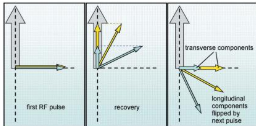
T1 contrast generation.
