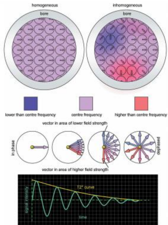
Figure 2.15 T2* decay and field inhomogeneities.
