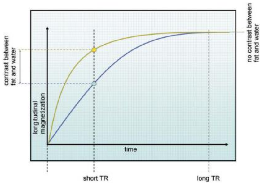
The T 1 differences between fat and water.
