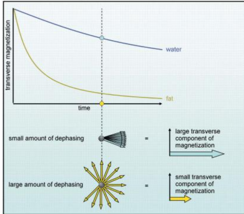
T 2 contrast generation.
