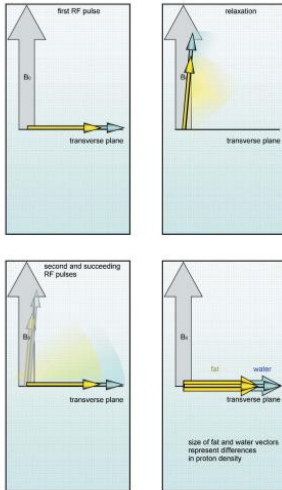
Figure 2.14 No saturation with a long TR.
