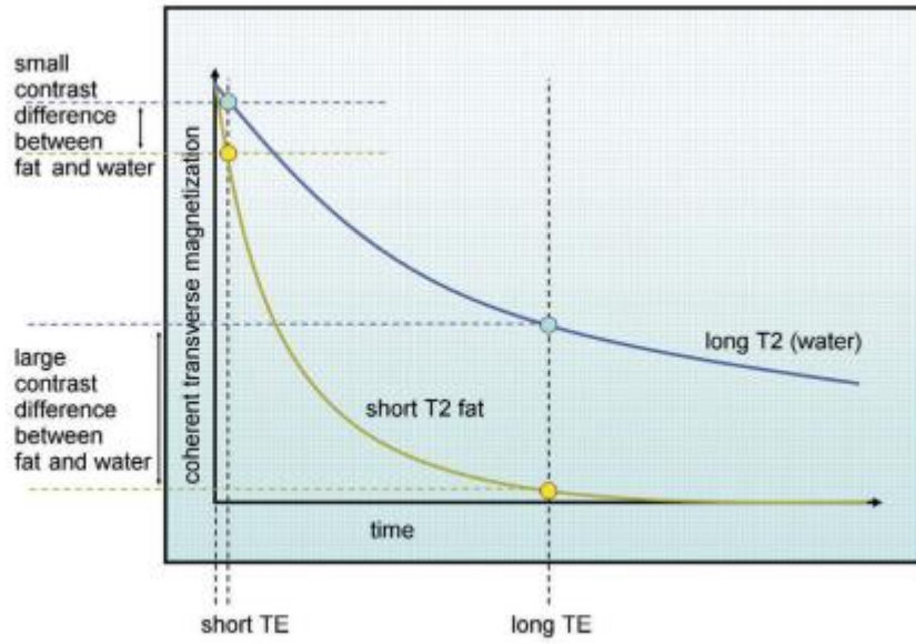
Figure 2.9 The T 2 differences between fat and water.
