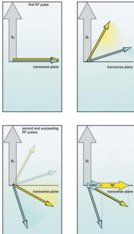
Figure 2.13 Saturation with a short TR.
