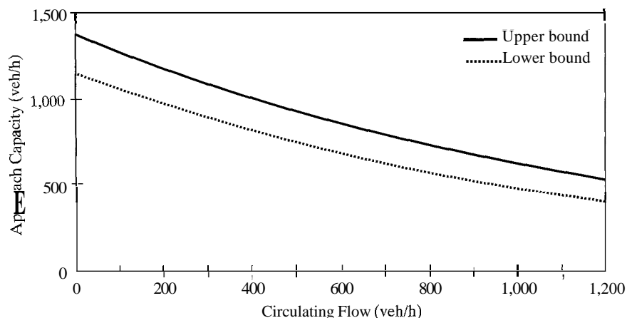
Figure 23.9: Approach Capacity at Roundabouts (Used with permission of Transportation Research Board, National Research Council, Highway Capacity Manual , 4th Edition, Washington DC, 2000, Exhibit 17-38, pg. 17-47.)
