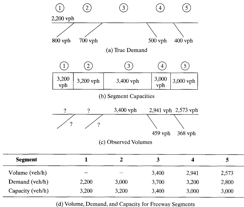
Figure 8.3: Effects of a Bottleneck on Observed Volumes
