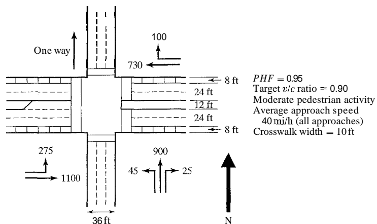
Figure 18.23: Intersection for Problem 18-5
