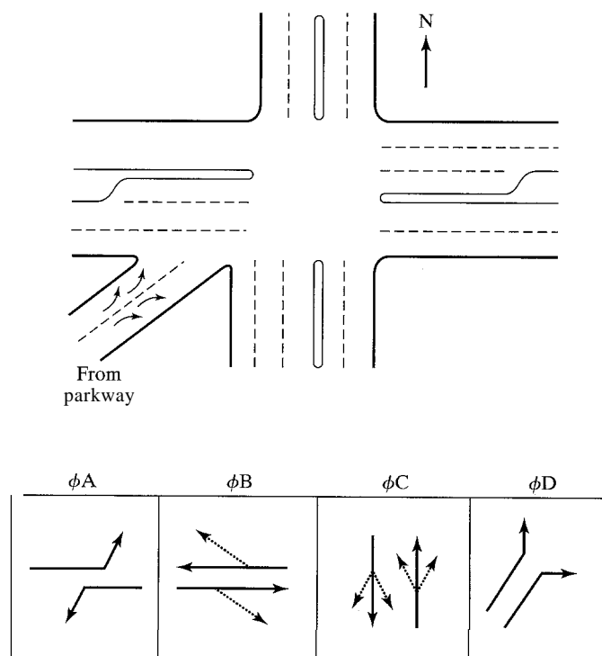
Figure 18.10: A Five-Leg Intersection Illustrated
