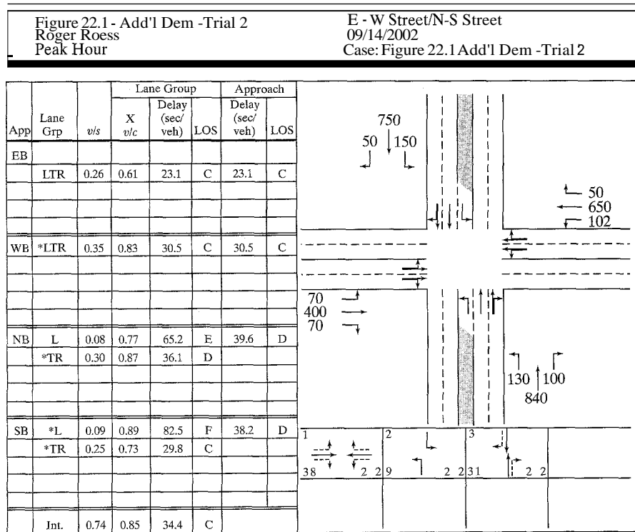
Figure 22.5: HCM-Cinema Results for Additional Demand Scenario—Trial 2 (Used with permission of KLD & Associates and Polytechnic University.)
