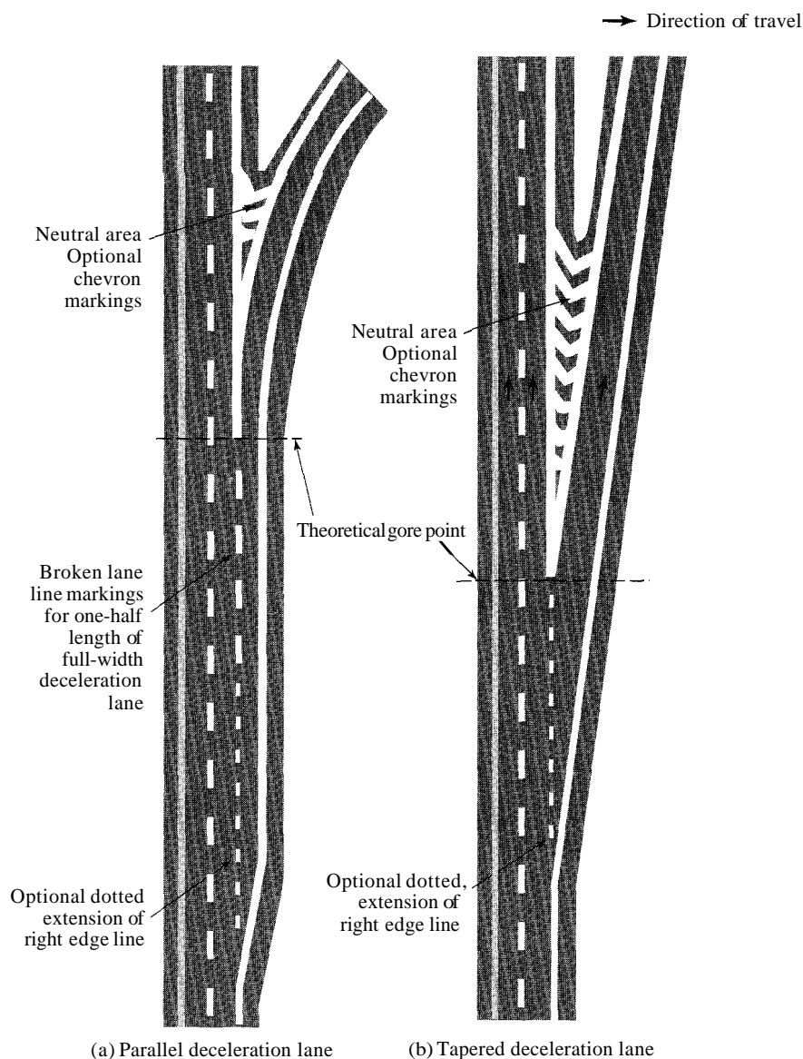
Figure 15.5: Typical Off-Ramp Junction Markings (Used with permission of Federal Highway Administration, Manual on Uniform Traffic Control Devices , Millennium Edition, Washington DC, 2000, Figure 3B-8a,b, pg. 3B-16.)
