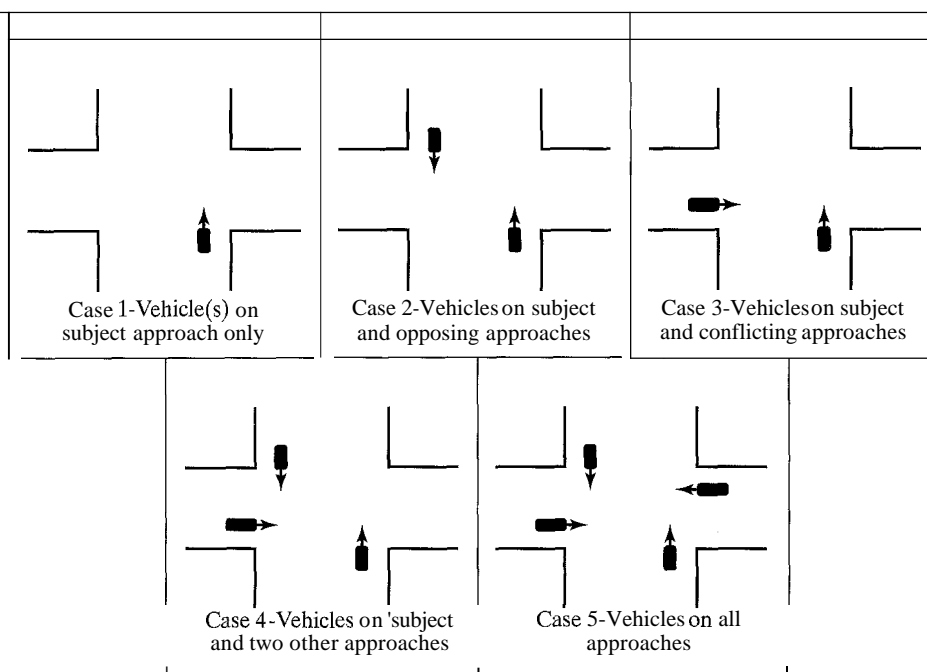
Figure 23.10: Potential Situations at AWSC Intersections (Used with permission of Transportation Research Board, National Research Council, Highway Capacity Manual , 4th Edition, Washington DC, 2000, Exhibit 10-25, pg. 10-30.)
