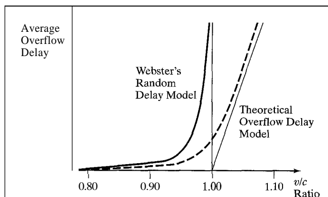
Figure 17.17: Random and Overflow Delay Models Compared (Adapted with permission of Transportation Research Board, National Research Council, Washington DC, from Hurdle, VF. “Signalized Intersection Delay Model: A Primer for the Uninitiated, Transportation Research Record 971, pg. 101, 1984.)
