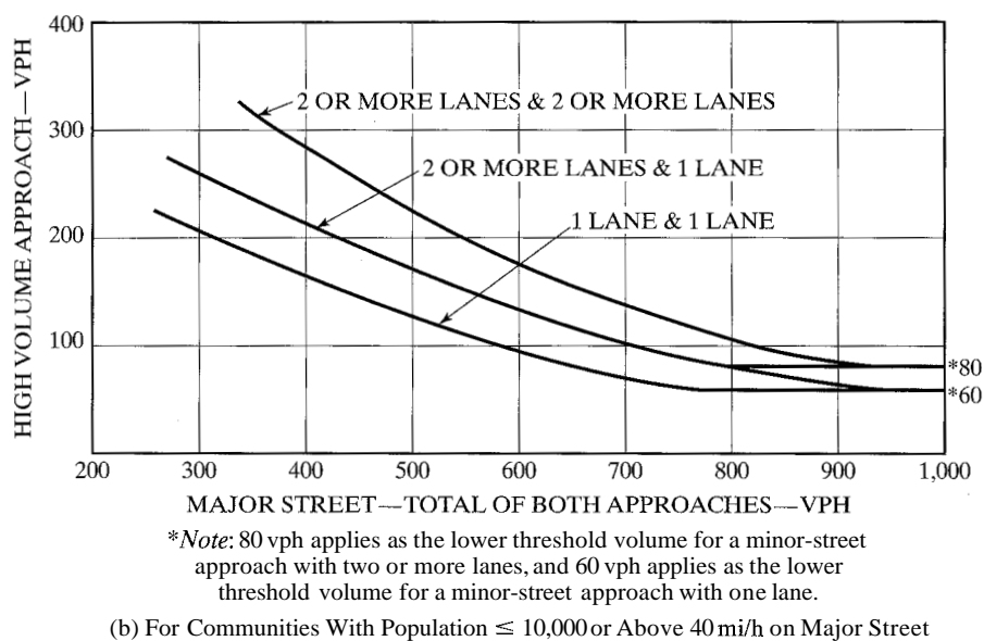
Figure 16.5: Warrant 2: Four-Hour Vehicular Volume Warrant (Used with permission of Federal Highway Administration, U.S. Department of Transportation, Manual on Uniform Traffic Control Devices , Millennium Edition, Washington DC, 2000, Figures 4C-1, 4C-2, pg. 4C-7.)
