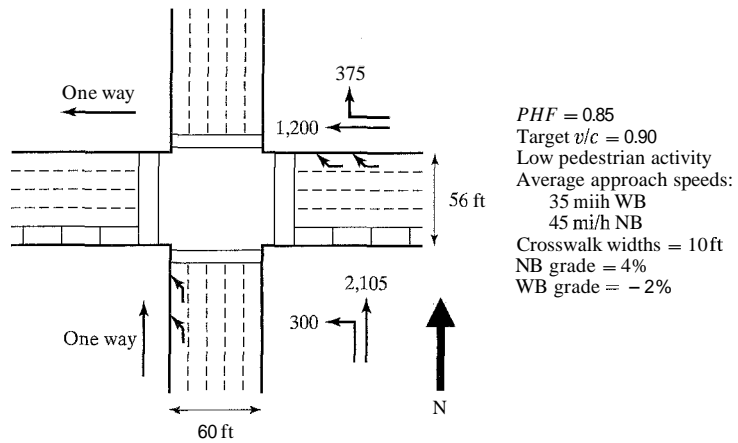
Figure 18.21: Intersection for Problem 18-3
