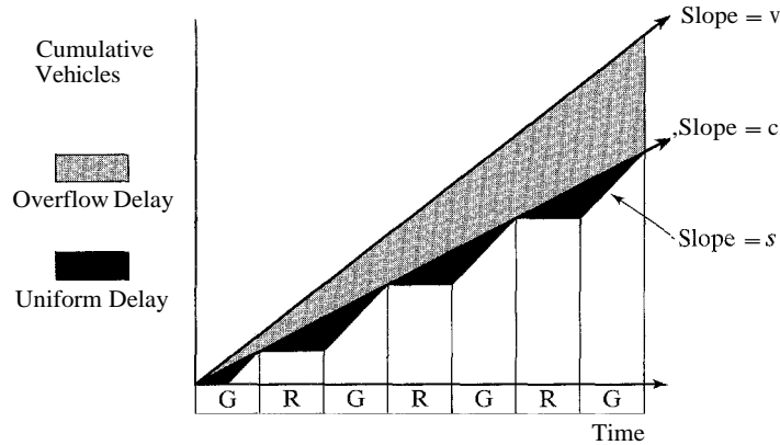
Figure 17.14: An Oversaturated Period Illustrated
