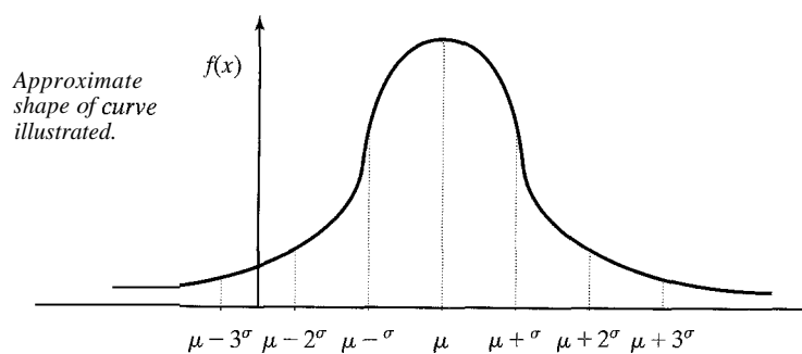
Figure 7.1: Shape of the Normal Distribution Function
