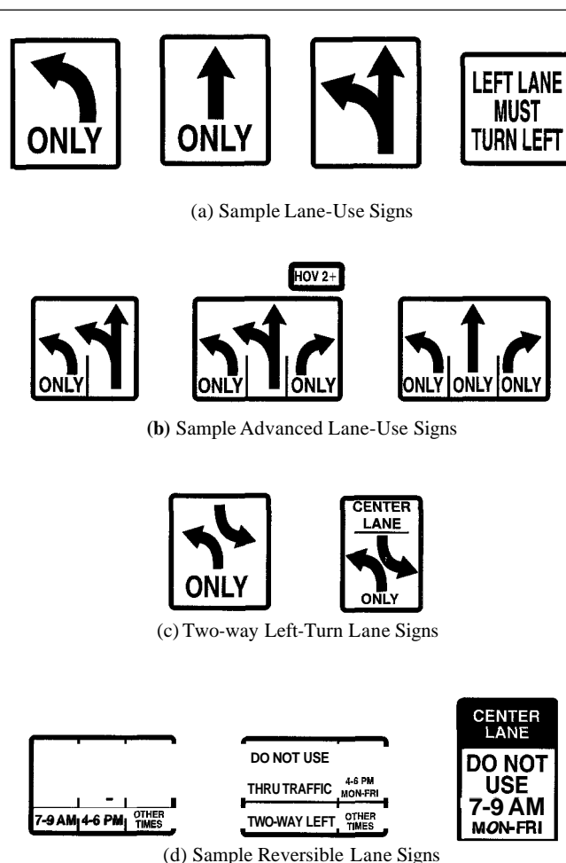
Figure 4.10: Lane-Use Control Signs (Used with permission of Federal Highway Administration, U.S. Department of Transportation, Manual on Uniform Traffic Control Devices , Millennium Edition, pgs. 2B-19 and 2B-22, Washington DC, 2000.)
