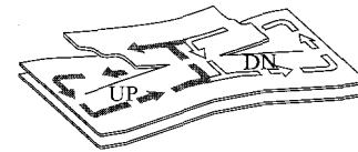
(l) Double sloping-floor system with midpoint crossover.
