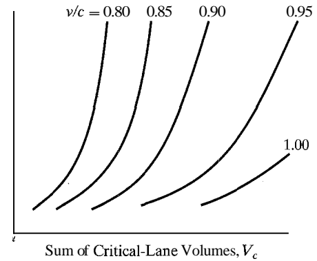
Figure 17.4: Desirable Cycle Length vs. Sum of Critical-Lane Volumes
