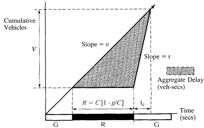
Figure 17.13: Webster's Uniform Delay Model Illustrated
