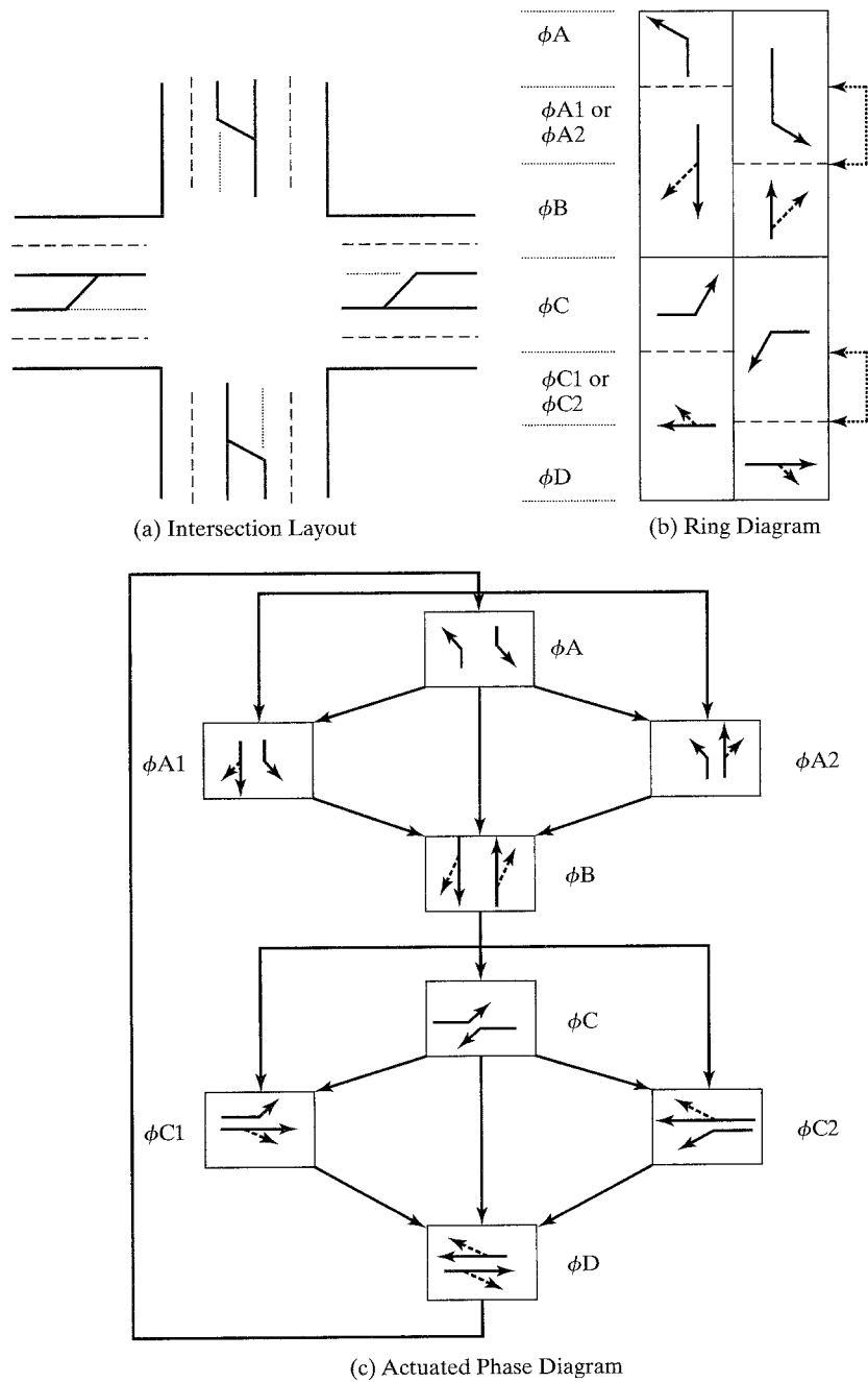
Figure 18.7: Eight-Phase Actuated Control Illustrated
