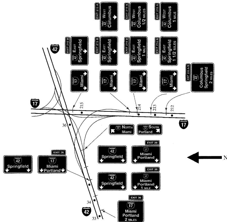
Figure 15.17: A Complex Interchange Between Two Interstate Facilities (Used with permission of Federal Highway Administration, Manual on Uniform Traffic Control Devices , Millennium Edition, Washington DC, Figure 2E-25, pg. 2E-58.)
