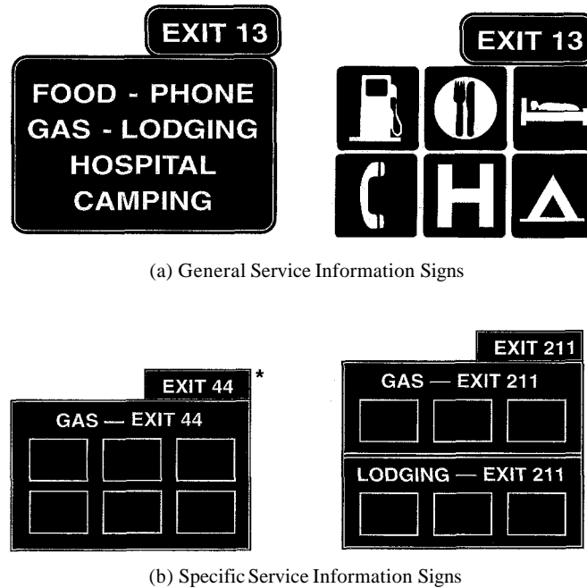
Figure 4.16: Service Information Signs (Used with permission of Federal Highway Administration, U.S. Department of Transportation, Manual on Uniform Traffic Control Devices , Millennium Edition, Figure 2E-34, pg. 2E-72, pg. 2F-4, Washington DC, 2000.) * Exit number panel is optional.
