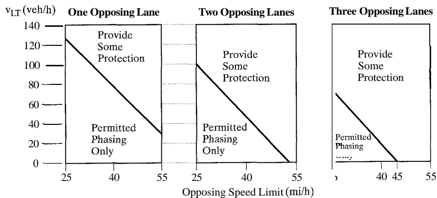
Figure 18.1: Recommended Selection Criteria for Left-Turn Protection (Used with permission of Transportation Research Board, National Research Council, Asante, S., Ardekani, S., and Williams, J., "Selection Criteria for Left-Turn Phasing and Indication Sequence," Transportation Research Record 1421 , Washington DC, 1993, pg. 11.)
