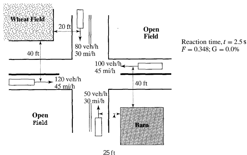
Figure 16.11: Intersection for Problem 16-1
