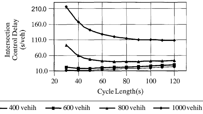
Figure 22.9: Cycle Length versus Delay for Various Demand Levels
