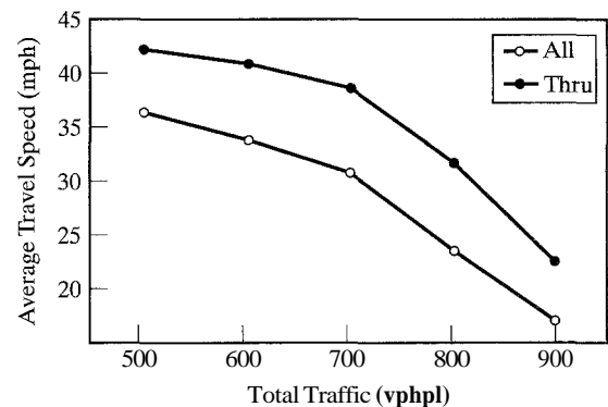
Figure 25.7: Speed of Through Vehicles versus All Vehicles on an Arterial Link (From W. McShane, et al. , “Insights into Access Management Details Using TRAF-NETSIM,” presented at the Second National Conference on Access Management, 1996.)
