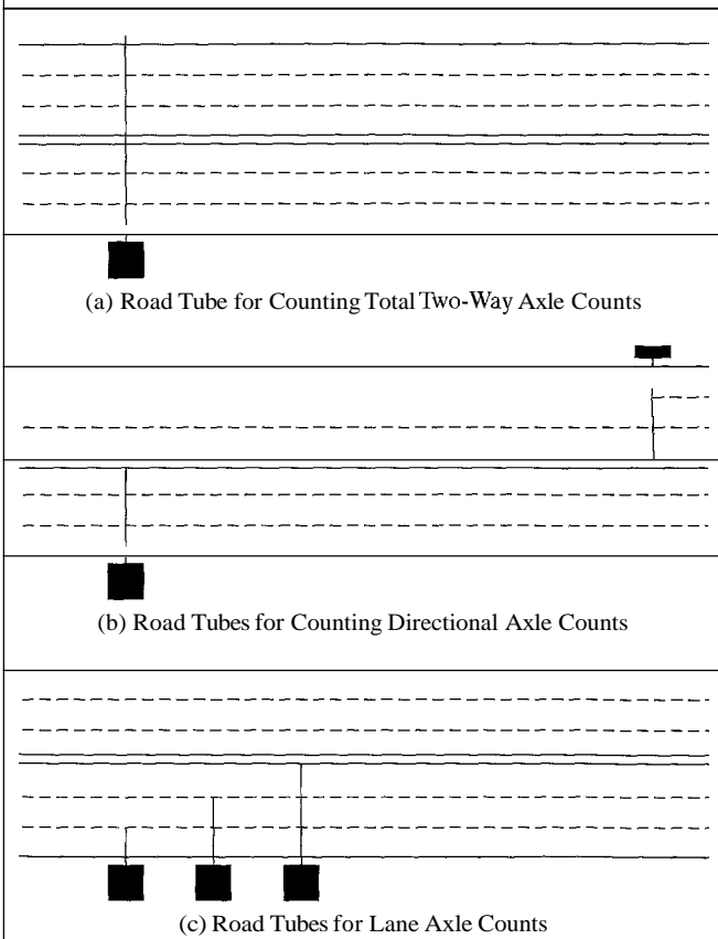
Figure 8.12: Alternative Field Set Ups for Road Tubes
