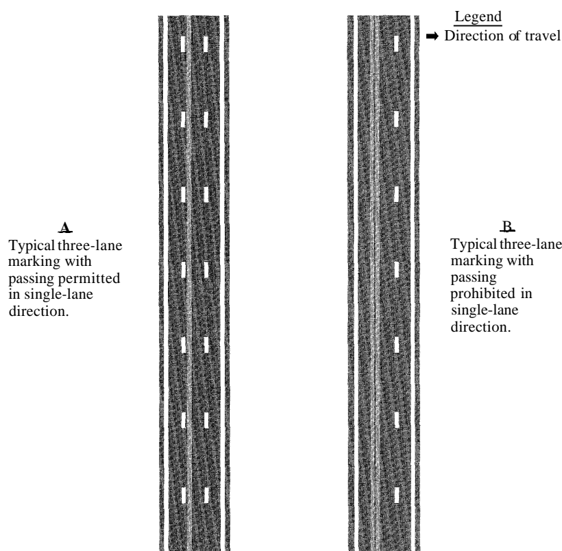
Figure 15.3: Typical Markings on Three-Lane Rural Highways (Used with permission of Federal Highway Administration, Manual on Uniform Traffic Control Devices , Millennium Edition, Washington DC, 2000, Figure 3B-3, pg. 3B-5.)
