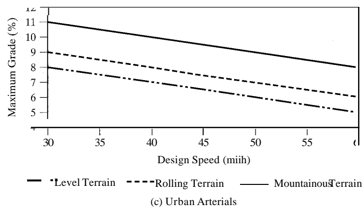
Figure 3.16: General Criteria for Maximum Grades
