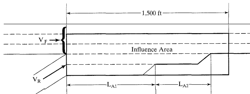
Figure 13.A.II.1: Typical Two-Lane On-Ramp (Used with permission of Transportation Research Board, National Research Council, Highway Capacity Manual , 2000, Exhibit 25-8, pg. 25-9.)
