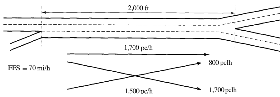
Figure 13.12: Weaving Area for Example 13-2
