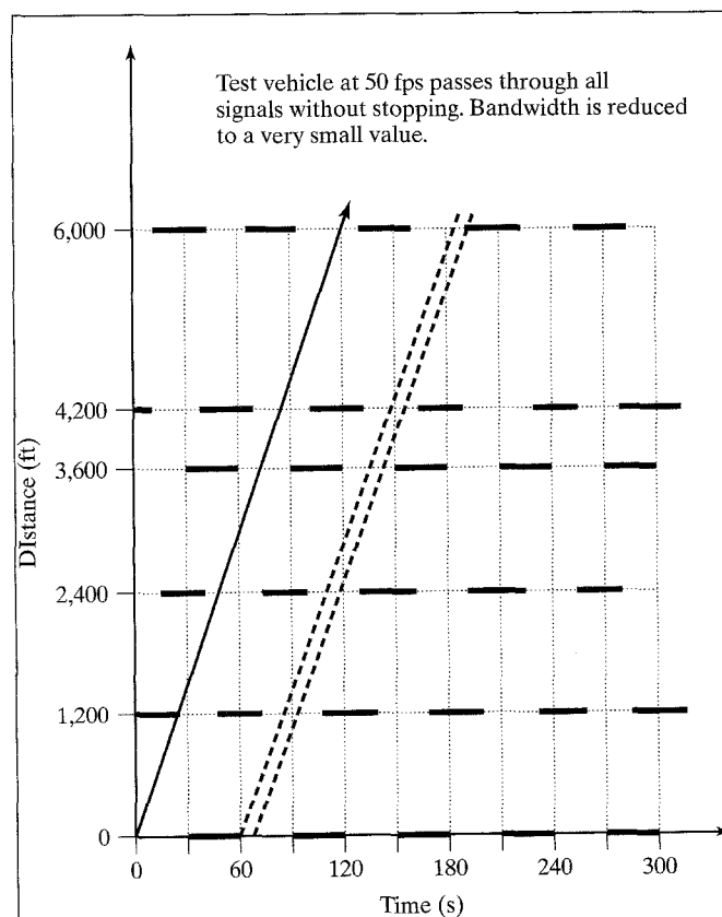
Figure 24.6: The Effect of a 50-ft/s Platoon Speed on Progression
