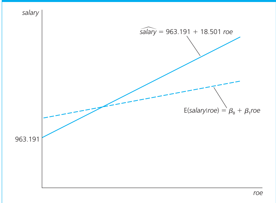
FIGURE 2.5 The OLS regression line \widehat{salary} = 963.191 + 18.501 roe and the (unknown) population regression function.
