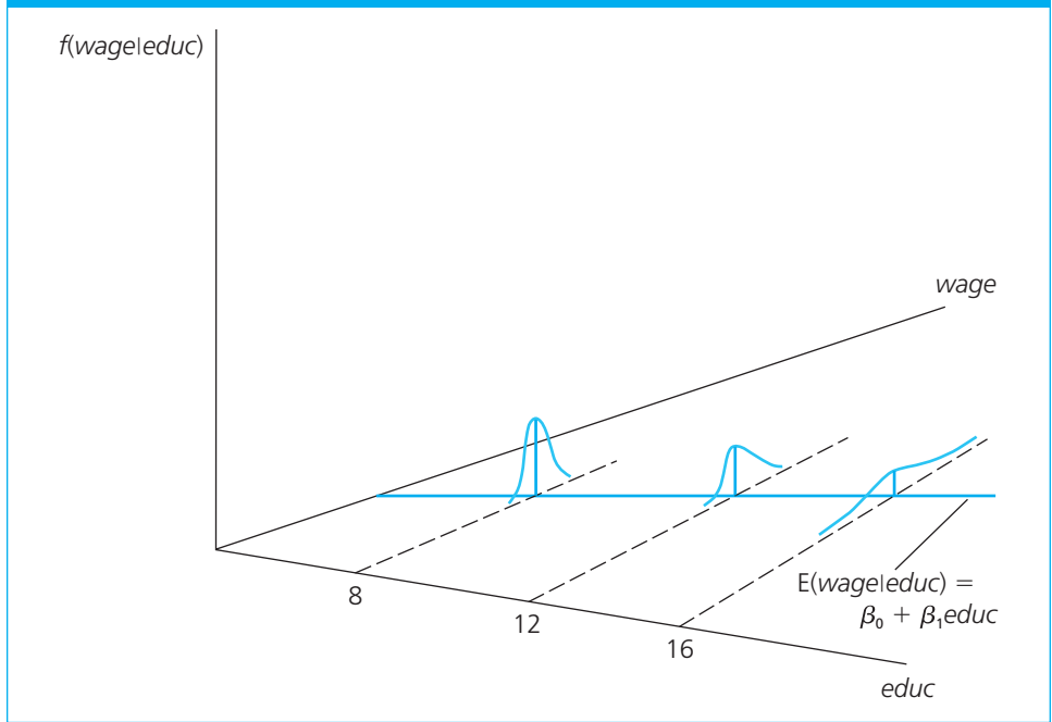
FIGURE 2.9 \text{Var}(\text{wage}|\text{educ}) increasing with \text{educ} .
