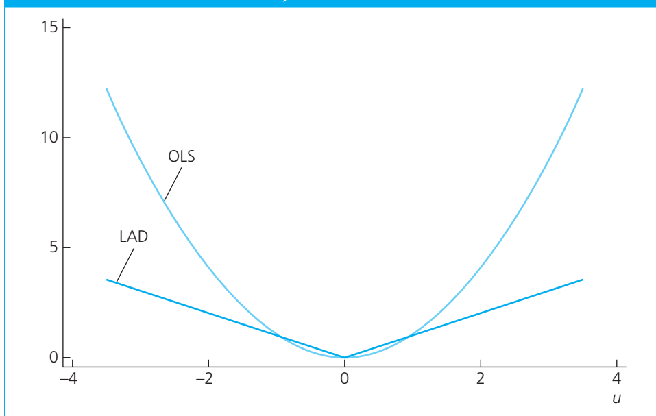
FIGURE 9.2 The OLS and LAD objective functions.
