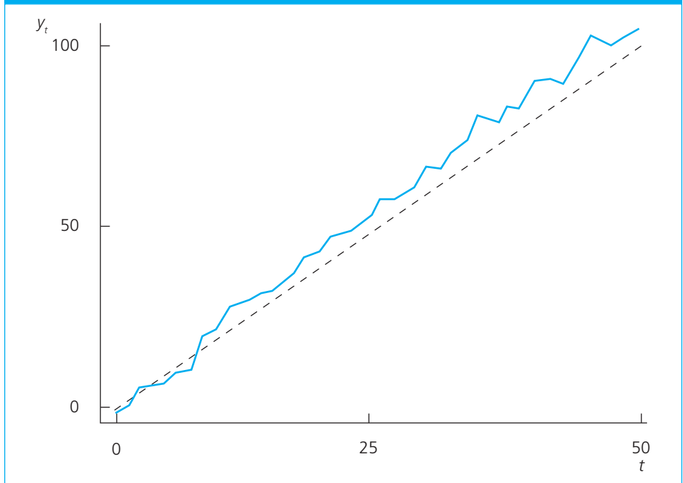
FIGURE 11.3 A realization of the random walk with drift, y_t = 2 + y_{t-1} + e_t , with y_0 = 0 , e_t s Normal(0, 9), and n = 50 . The dashed line is the expected value of y_t , E(y_t) = 2t .
