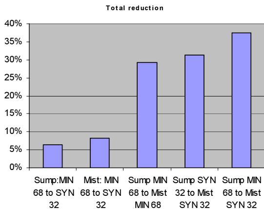
Figure 14. Frictional Power Loss Relationships for Synthetic Lubricants and Different Lube Oil Application Methods.
