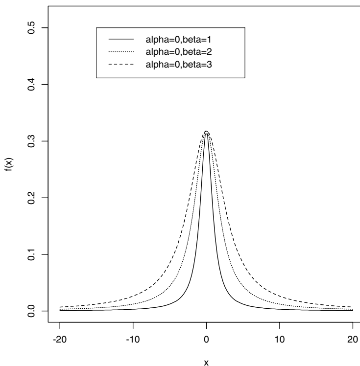
Fig. 83 Laplace distributions for \alpha = 0 ; \beta = 1, 2, 3 .
