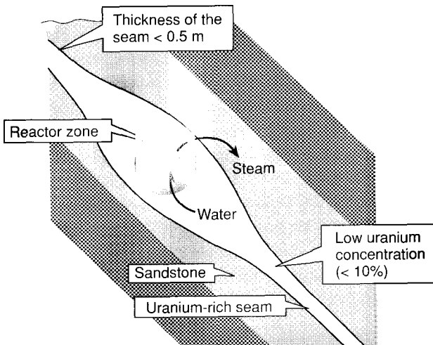
Fig. 6.12 The geological structure of the site of the Oklo natural reactor. A uranium-rich seam lies within a layer of sandstone lying on another layer of granite. The tilt of the granite and sandstone layers led to localized concentrations of uranium and water. When they exceed 10 per cent chain reactions can begin. The uranium layer must be thick enough to prevent the neutrons escaping, and be free from contamination by other heavy elements that would absorb all the neutrons. The nuclear reactions were self-regulated by the moderating presence of the water, which turned into steam when the reactions went faster, so slowing them down, but condensed when the reactions slowed down, so reducing the absorption of neutrons and speeding up the reactions gain.
