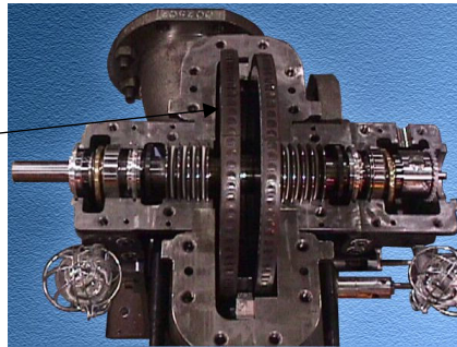
Figure 7. Photo of Small Turbine with Cover Removed Showing Rotor.
