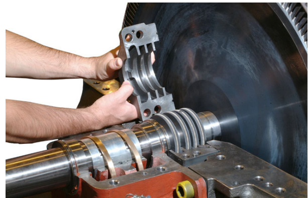
Figure 10. Carbon Ring Seal Arrangement.
