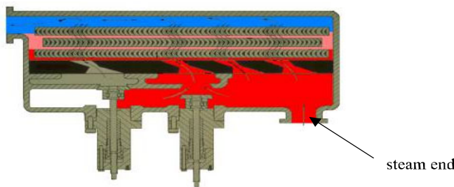
Figure 4. Illustration of Turbine Steam End and Hand Valve Ports.
