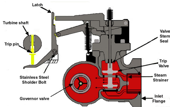
Figure 3. Illustration of Typical Steam Chest.
