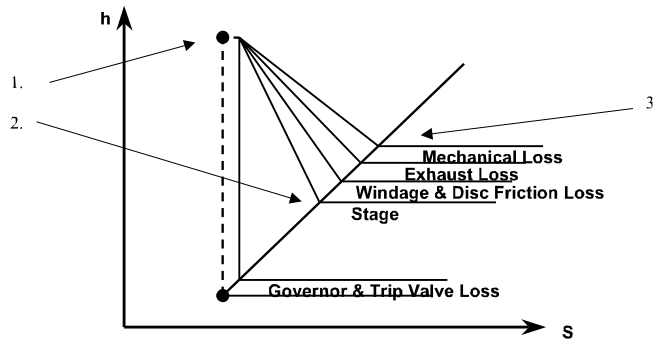
Figure 13. Mollier Chart Illustration.
