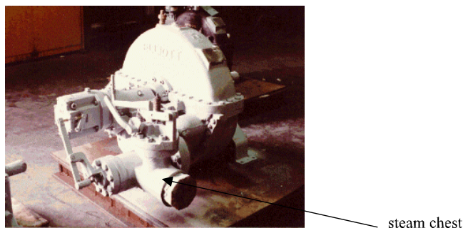
Figure 2. View from Inlet Side of Turbine.
