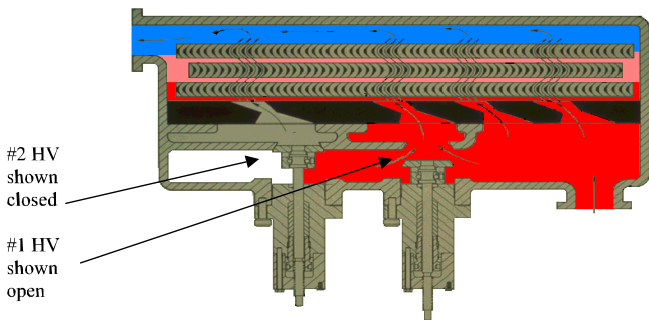
Figure 14. Hand Valve Illustration.
