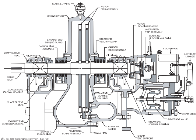
Figure 1. Cross Section of Typical Single-Stage Steam Turbine.
