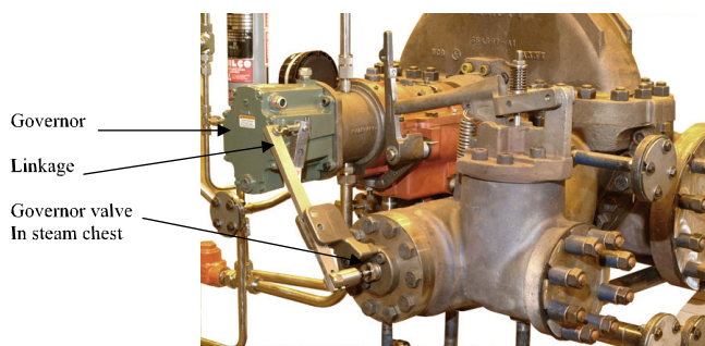
Figure 11. Turbine Controls.
