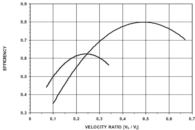
Figure B-1. Typical Efficiency Curves for Turbine Staging.
