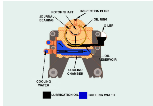
Figure 9. Ring-Oiled Lubrication.
