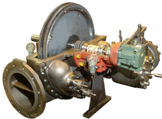
Figure 8. Turbine with Cover Removed.
