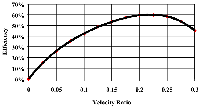
Figure 12. Typical Efficiency Curve for Single-Stage Turbine.
