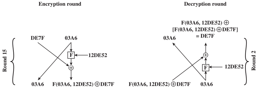
Figure 3.4 Feistel Example
