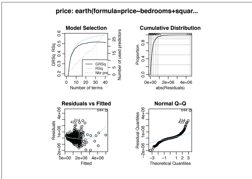
Figure 20-7. Output of plot.earth
