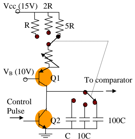
Figure C.15 Symbolic circuit diagram of the sweep generator
