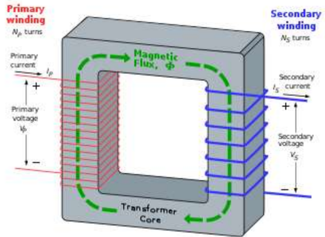
Figure 2. 46 A trnsformer
