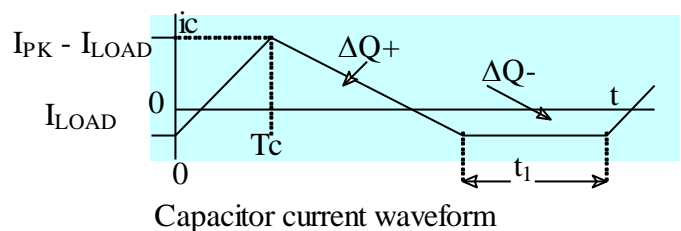
Figure 6.27 Inductor and capacitor waveform
