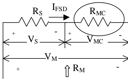
Figure 4. 14 Basic DC voltmeter
