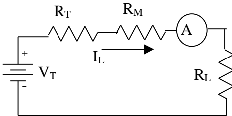
Figure 4.19 Ammeter loading
