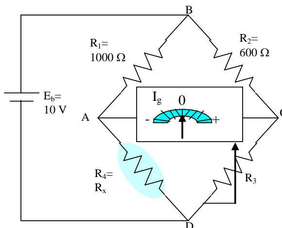
Figure 8.20 Circuit for null-mode
