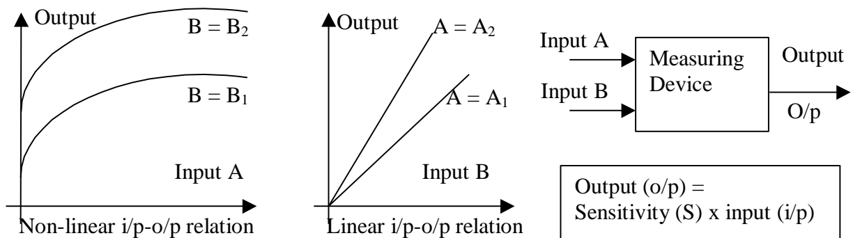
Figure 3.1 Static calibration curves for a multi-input single-output system
