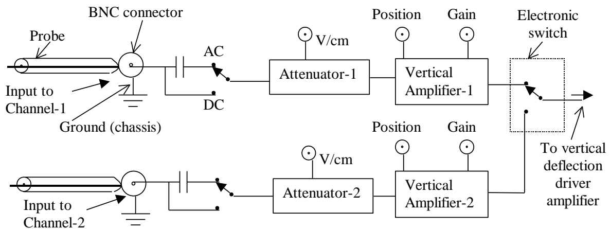
Figure 5.18 Multi-trace operation using an electronic switch
