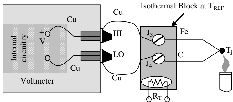
Figure 7.25 External reference junction without ice bath
