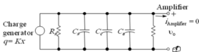
Figure 8.7 Model of the piezoelectric crystal
