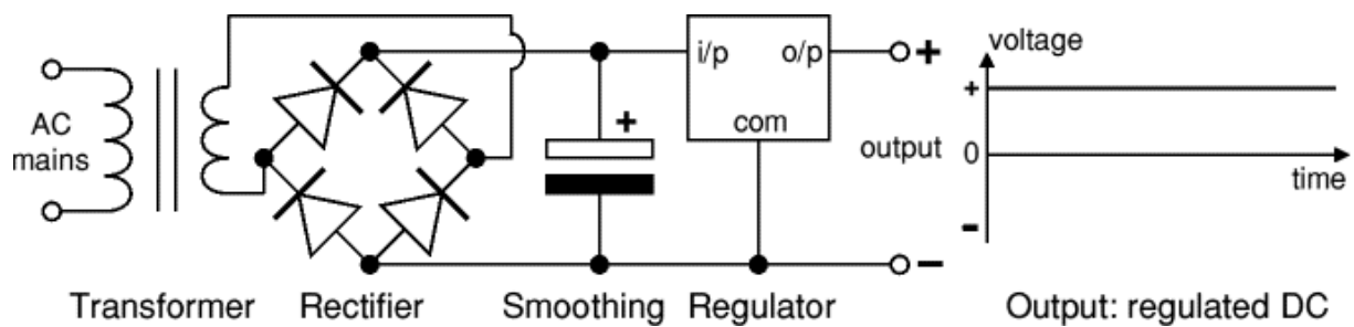
Figure 6.17 Simplified diagram of a regulated power supply
