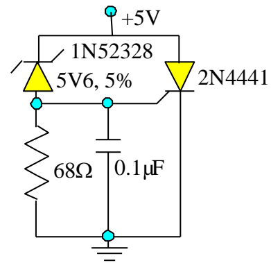
Figure 6.20 Over-voltage crowbar
