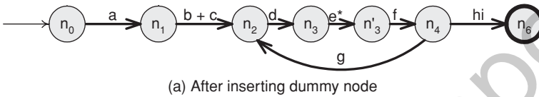
Figure 2.48. After step 2 in path expression reduction.
