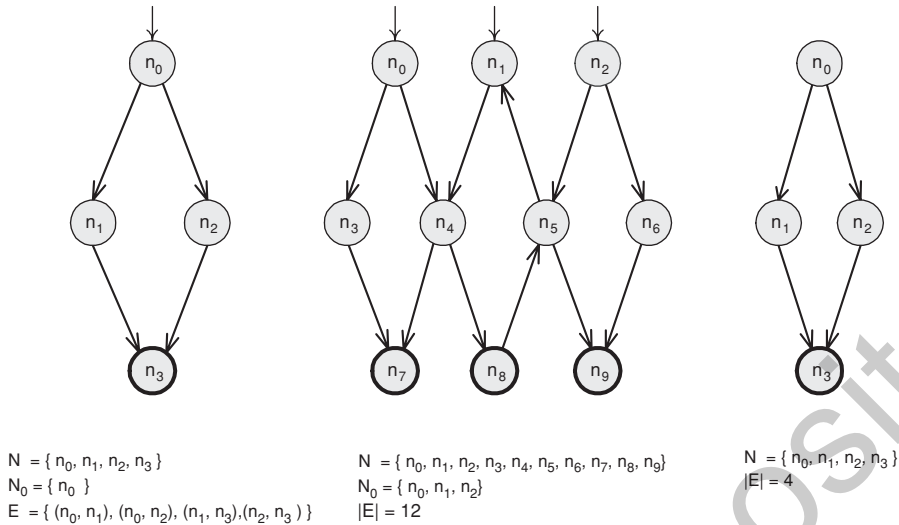
(a) A graph with a single initial node (b) A graph with multiple initial nodes (c) A graph with no initial node
