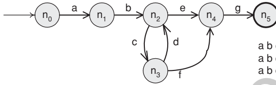
(b) A graph with a loop
