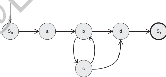
Figure 2.8. Graph with a loop.
