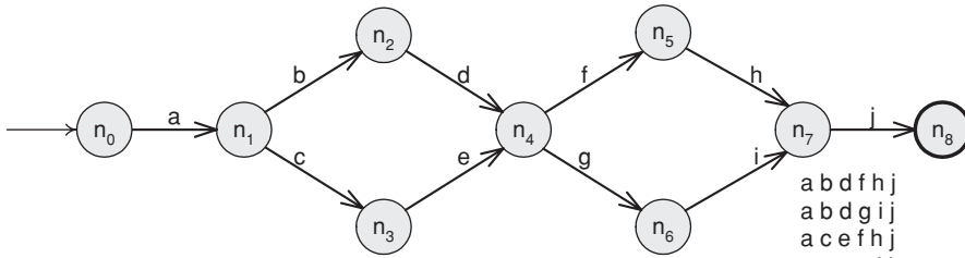
(a) A double diamond graph with edge labels
