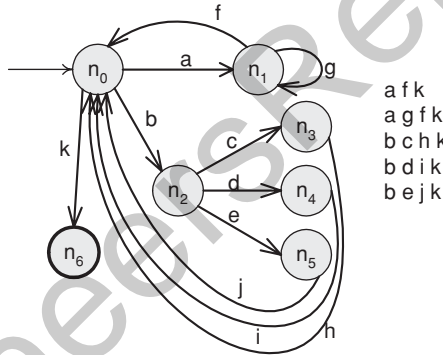
(c) The first FSM for stutter
