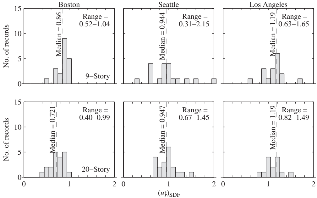
Figure 23.2.2 Histograms of ratio (u_r^*)_{\text{SDF}} for SAC buildings: Boston, Seattle, and Los Angeles 9- and 20-story. The range of values and the median value of this ratio are noted.
