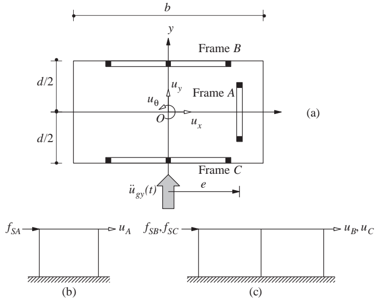
Figure 9.5.1 One-story system considered: (a) plan; (b) frame A; (c) frames B and C.
