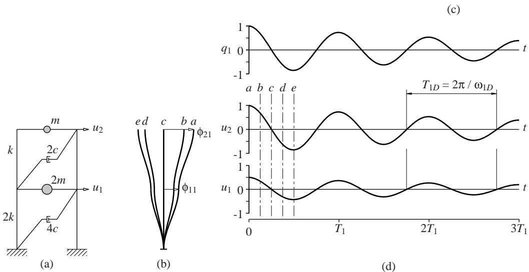
Figure E10.12.1 Free vibration of a classically damped system in the first natural mode of vibration: (a) two-story frame; (b) deflected shapes at time instants a , b , c , d , and e ; (c) modal coordinate q_1(t) ; (d) displacement history.
