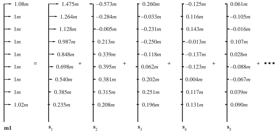
Figure 20.5.2 Modal expansion of the distribution \mathbf{s} = \mathbf{m}\mathbf{u} of effective earthquake forces.
