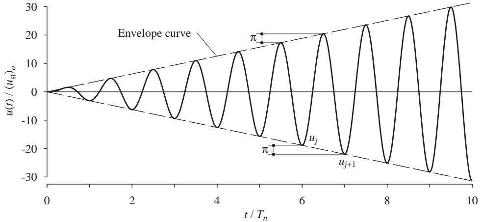
Figure 3.1.4 Response of undamped system to sinusoidal force of frequency \omega = \omega_n ; u(0) = \dot{u}(0) = 0 .
