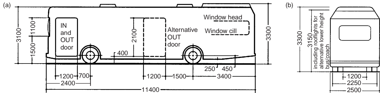
▲ 8.1 Single-decker bus.
