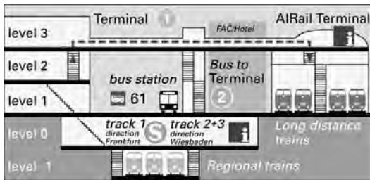
▲ 6.39 Cross-section showing regional rail station and national rail station/AIRail (Courtesy of airport website).
