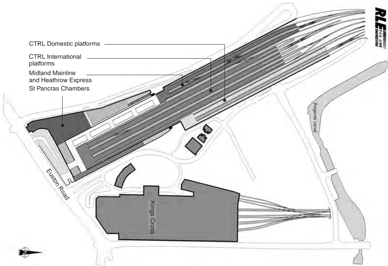
▲ 6.141 St Pancras Station, London: diagram, platform level (Courtesy of CTRL Press Office).
