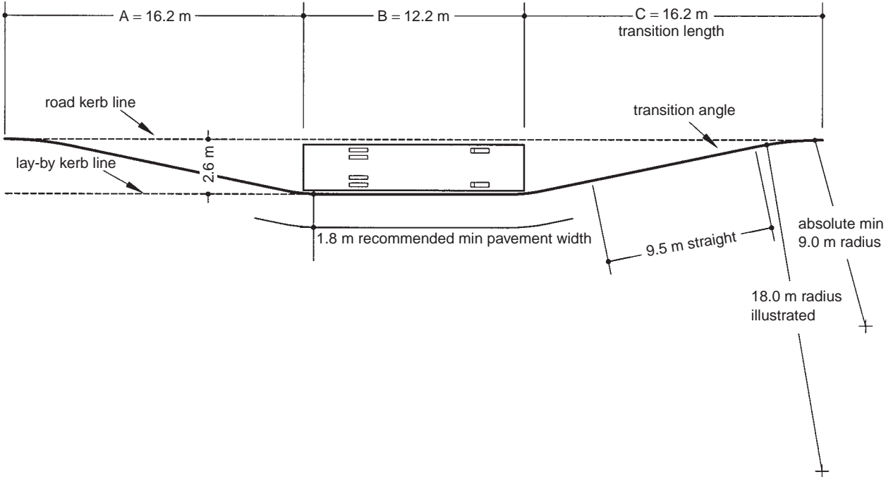
▲ 8.7 A lay-by with one bus stop, assuming normal urban speed of approach. The transition length of 16.2m is the minimum for a 12-m rigid vehicle. Three bus stops is the desirable maximum in a lay-by, the maximum comfortable distance for a pedestrian to walk. Overall length is A + nB + C , where n is the number of buses to be accommodated.
