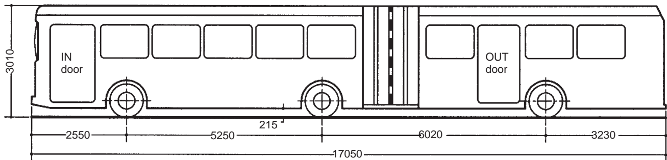
▲ 8.2 Articulated bus.
