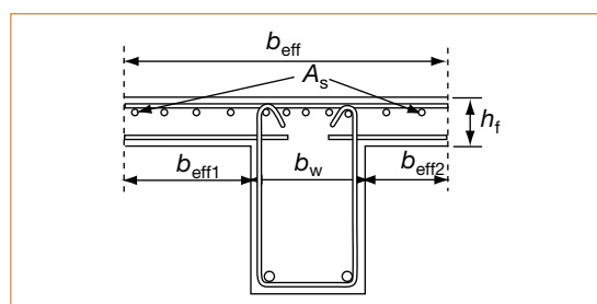
Figure 6.16 Placing of tension reinforcement in a flange cross-section
