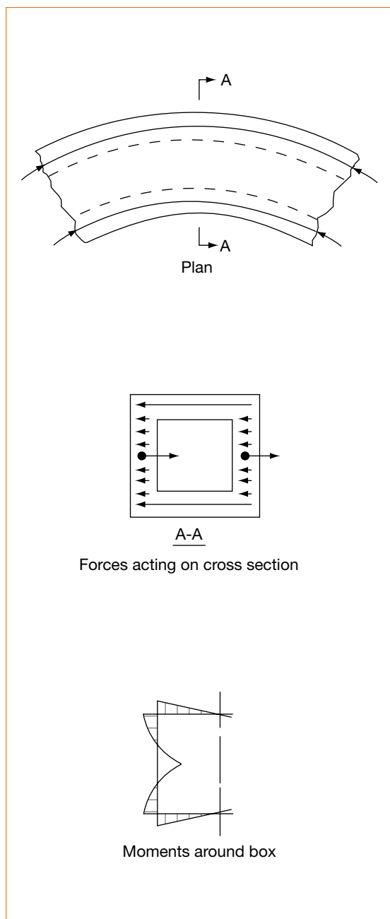
Figure 7.20 Forces in box girder in plan
