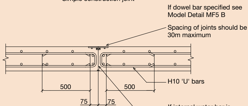
DETAIL 'A' Simple construction joint
