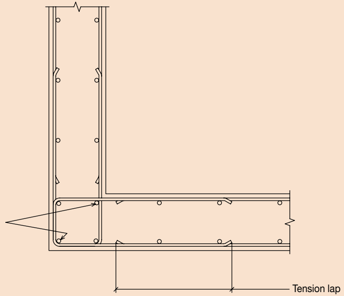
DETAIL 'A'
