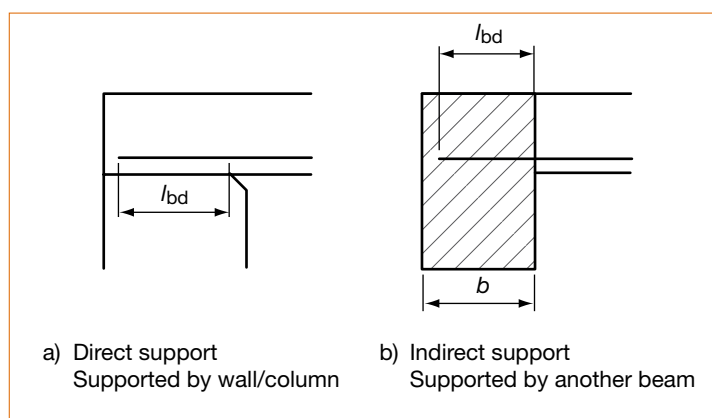
Figure 6.1 Anchorage of bottom reinforcement at end supports
