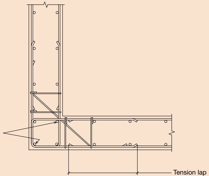
DETAIL 'A'
