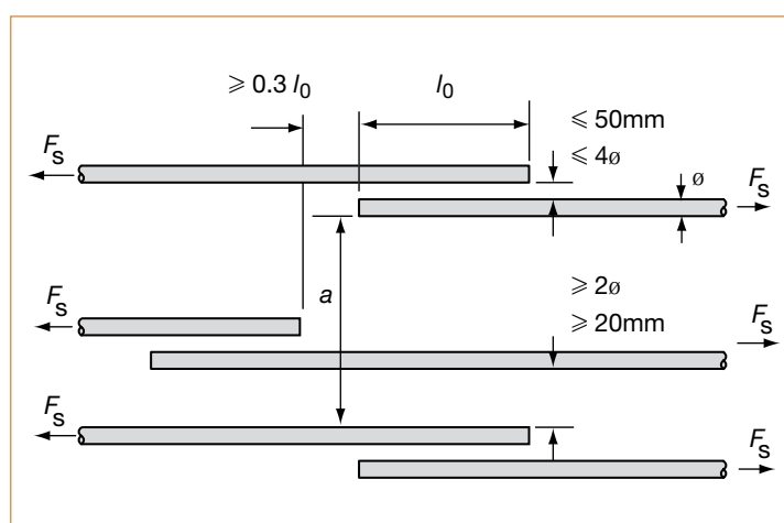
Figure 6.2 Adjacent laps
