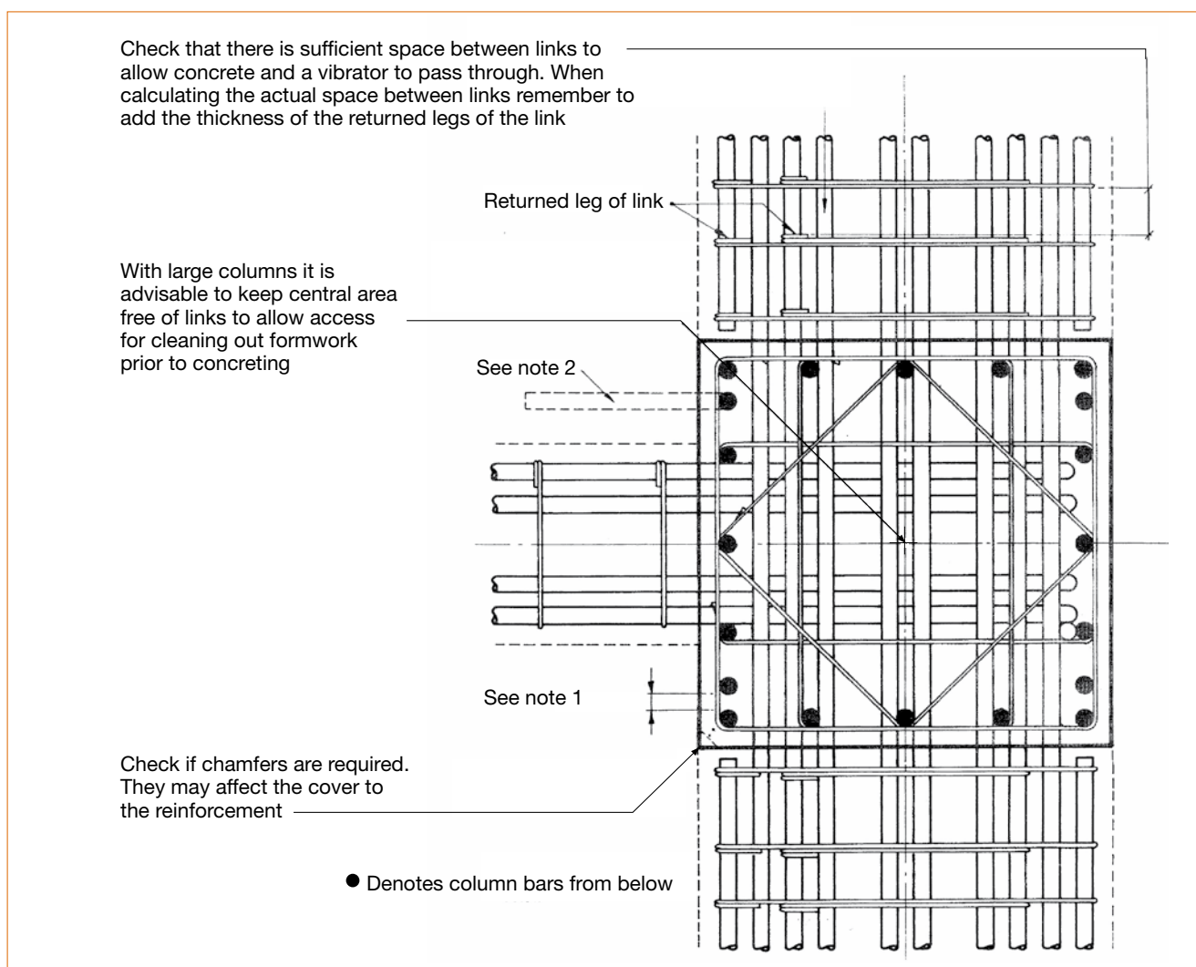
Figure 4.4 Plan of reinforcement at beam/column intersection
