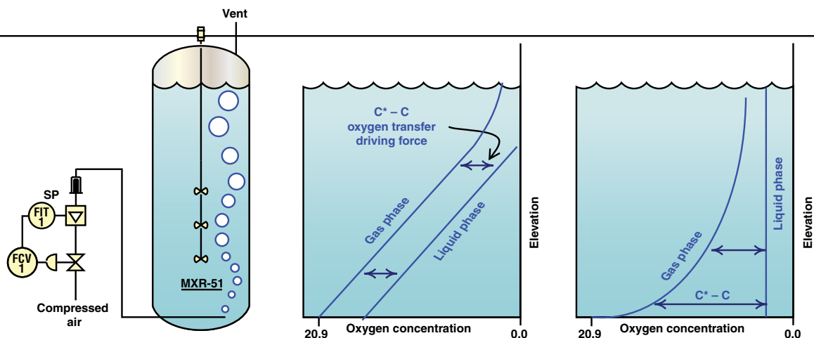
FIGURE 3. The oxygen transfer rates and the amount of dissolved oxygen in the liquid are strongly affected by mixing in a fermenter
