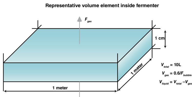
FIGURE 1. A representative volume element of the fermenter is depicted in this sketch, where V is volume and F is the gas flowrate
