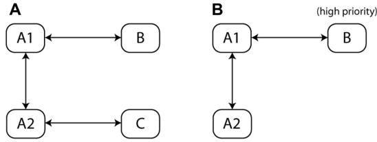
Fig. 1. Double-headed arrows indicate that the connected pairs are compatible for exchange; i.e., the patient in one pair is compatible with the donor in the other. Pairs A1 and A2 are both from transplant center A, and pairs B and C are from different transplant centers. Transplant center A, which sees only its own pairs, can conduct an exchange among its pairs A1 and A2 since they are compatible; if it does so, this will be the only exchange, resulting in two transplants. However, if in fig. 1A transplant center A makes its pairs available for exchange with other centers, then the exchanges will be A1 with B and A2 with C, resulting in four transplants. However, in fig. 1B, the suggested exchange might be A1 with B, which would leave the patient in A2 without a transplant. Faced with this possibility (and not knowing if the situation is as in panel A or B), transplant center A might choose to transplant A1 and A2 by itself, without informing the central exchange.
