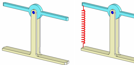
FIGURE 15: THE SWING ARM ON THE LEFT CAN MOVE WITHOUT DEFORMATION; THUS IT'S A MECHANISM. ANY MOVEMENT IN THE ARM ON THE RIGHT IS ACCOMPANIED BY DEFORMATION OF THE SPRING; THIS MEANS IT'S A STRUCTURE.
