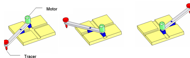
FIGURE 1: VARIOUS POSITIONS OF ELLIPTIC TRAMMEL SIMULATED USING CAD ANIMATOR
