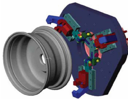
FIGURE 25: WARD MACHINE TOOL OF FOWLerville, MICHIGAN DESIGNED AND SIMULATED THE LATHE CHUCK.
