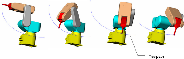
FIGURE 11: SIMULATED MOVEMENT OF AN INDUSTRIAL ROBOT THROUGH SEVERAL POSITIONS MAKES IT POSSIBLE TO CREATE A TOOLPATH WITHOUT ANY PHYSICAL TESTS.
