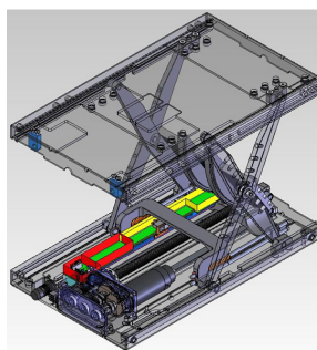
FIGURE 26: THIS LIFTING PLATFORM WAS DESIGNED BY SYNCRONESS, OF WESTMINSTER, COLORADO USING SOLIDWORKS, SOLIDWORKS MOTION, AND SOLIDWORKS SIMULATION AS DESIGN TOOLS.
