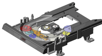
FIGURE 8: A CD DRIVE IS A COMPLEX MECHANISM, YET EASILY ANALYZED BY MOTION SIMULATION.
