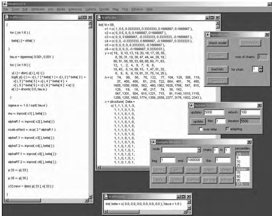
Fig. 2.6 WinBUGS fitting of a regression reformulation of model (2.5) to the Berkeley traffic data in Section 2.1.1.
