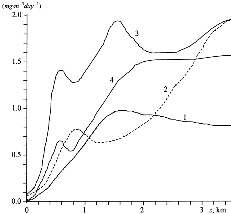
Figure 8.13. Average production of H_2S ( mg\ m^{-3}\ day^{-1} ) in the oceans: 1 – the Arctic Ocean; 2 – the Pacific Ocean; 3 – the Indian Ocean; 4 – the Atlantic Ocean.
