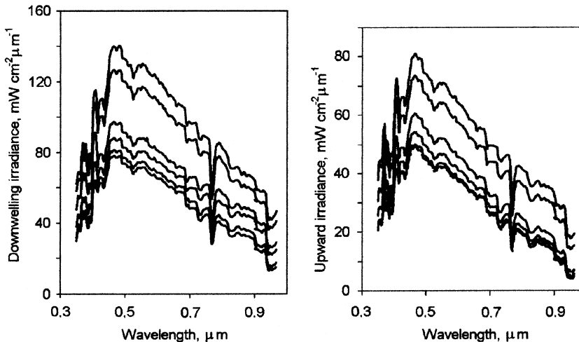
Figure 6.2. The results of airborne sounding under overcast sky conditions.
