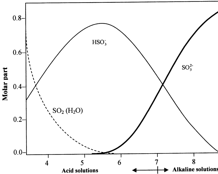
Figure 8.8. Relationship between molar parts of sulphite, bisulphate, and dissolved sulphur dioxide in the formation of pH level.
