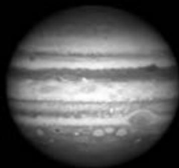
Jupiter 139,822 km
