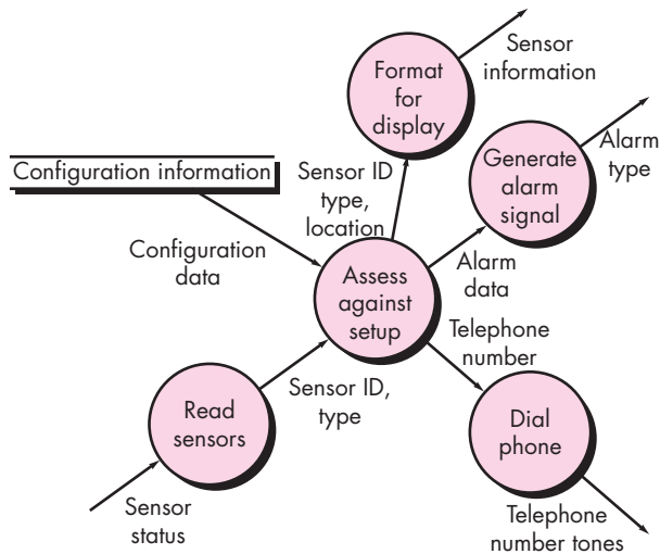
FIGURE 9.13 Level 3 DFD for monitor sensors with flow boundaries
