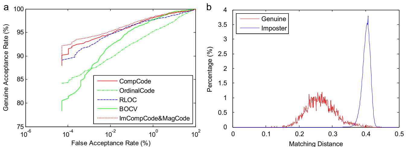
Fig. 8. (a) ROC curves obtained by five recognition methods in experiment 1 and (b) distance distributions of genuine matchings and imposter matchings with the proposed scheme in experiment 1.
