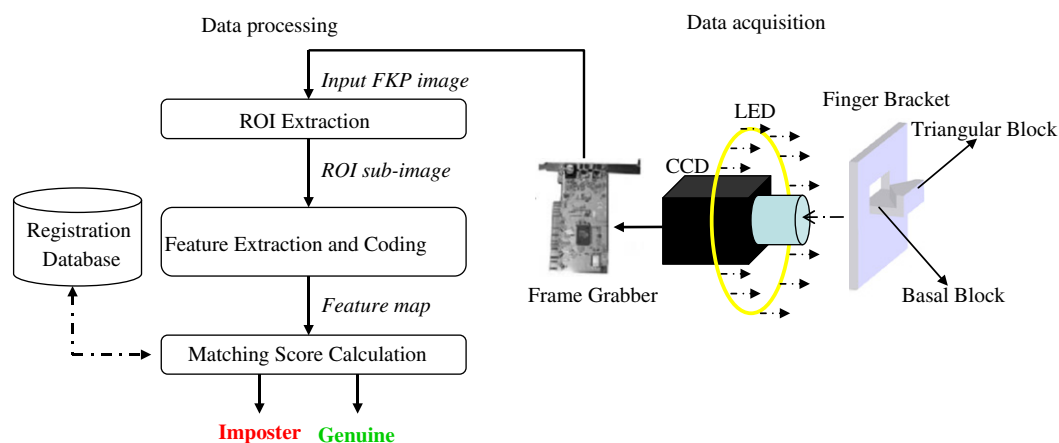
Fig. 1. Structure of the proposed FKP-based personal authentication system. The whole system is composed of a data acquisition module and a data processing module.
