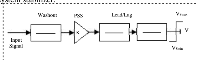
Fig.3. Power System Stabilizer
