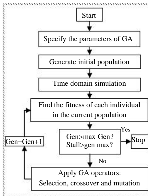
Fig.4. Flowchart of the GAs procedure
