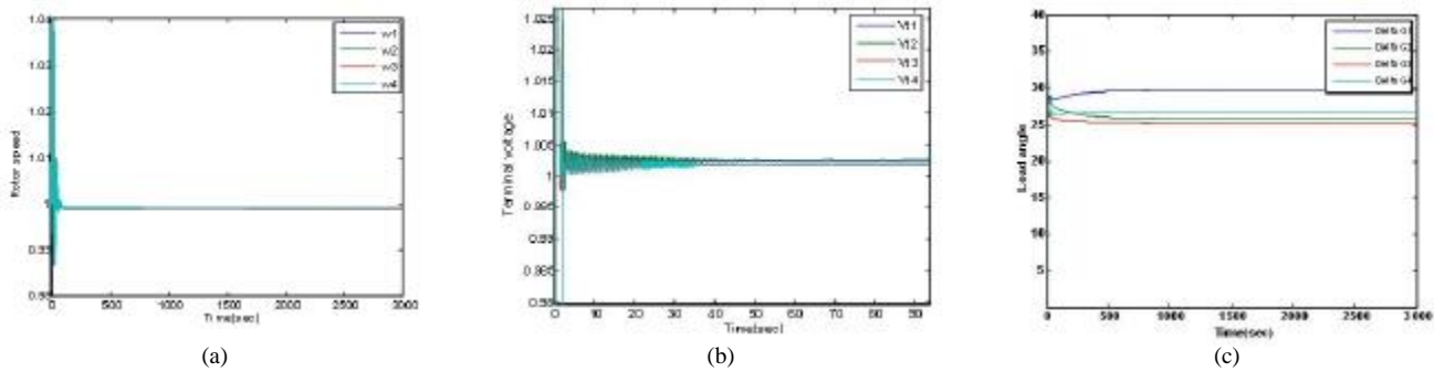
Fig.11. Generators rotor speed (a), terminal voltage (b) and Load angle (c) oscillations in LFO condition without PSS and with SVC optimization by PSO
