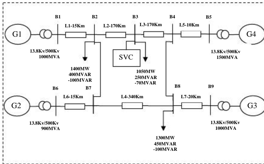
Fig.6. Schematic Model of Power System
