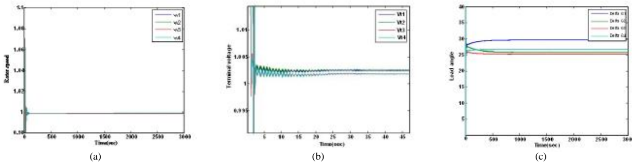
Fig.10. Generators rotor speed (a), terminal voltage (b) and Load angle (c) oscillations in LFO condition without PSS and with SVC optimization by GA
