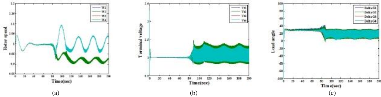
Fig.7. Generators rotor speed (a), terminal voltage (b) and Load angle (c) oscillations in LFO condition without compensating
