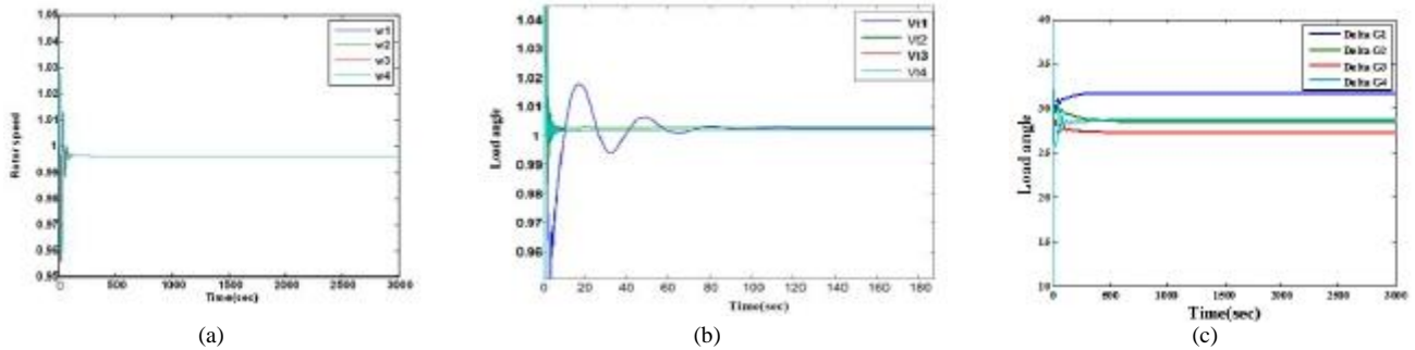
Fig.8. Generators rotor speed (a), terminal voltage (b) and Load angle (c) oscillations in LFO condition with PSS and without SVC optimization by GA
