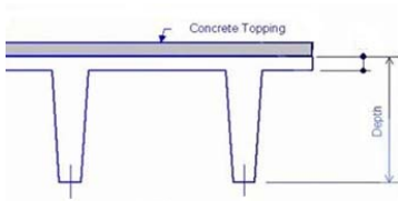
Typical Precast Double Tee Beam
