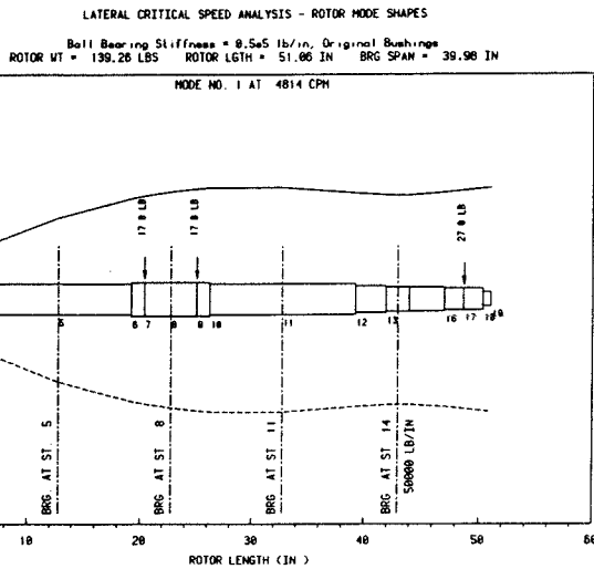
Figure 11. Pump Rotor Model and Vibration Mode Shape.
