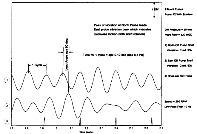
Figure 26. Illustration of Forward Whirl.
