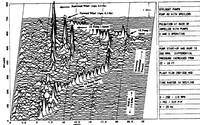
Figure 27. Pulsation Measured Behind Impeller with Spoilers Installed.
