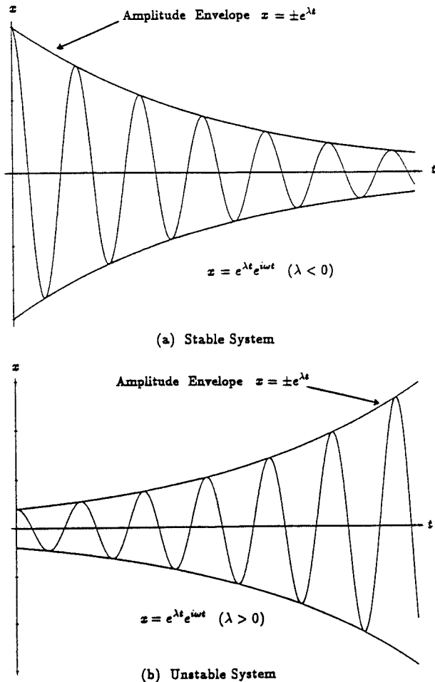
Figure 10. Comparison of Stable and Unstable Systems.
