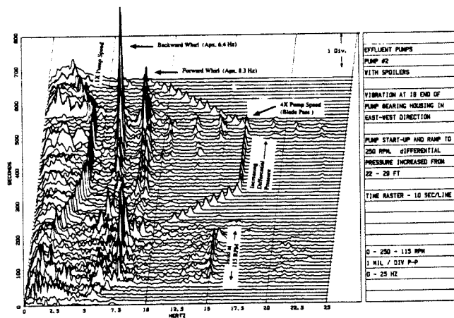
Figure 23. Shaft Instability Vibration with Spoilers Installed.
