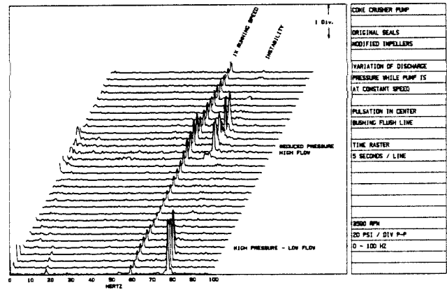
Figure 9. Frequency Spectra of Pulsation in Center Bushing Flush Line vs Pump Discharge Pressure with Original Bushings.
