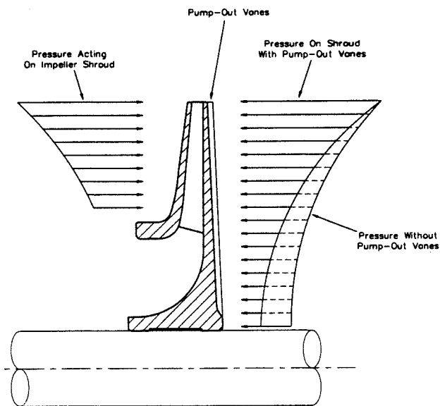
Figure 1. Pumpout Vanes used in a Single-Suction Impeller to Reduce Axial Thrust.
