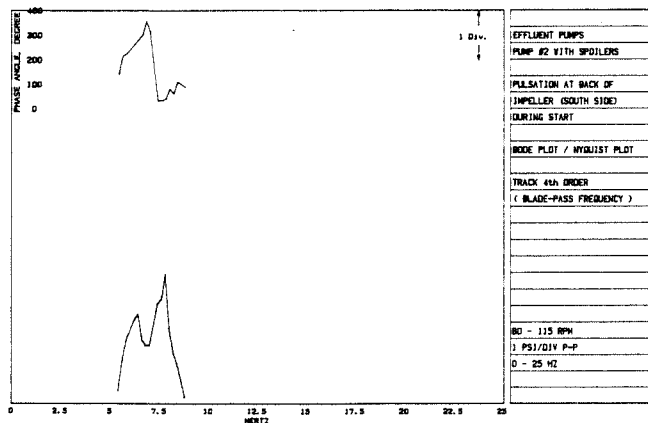
Figure 33. Bode Plot of Pulsation at Blade-Pass Frequency During Startup.
