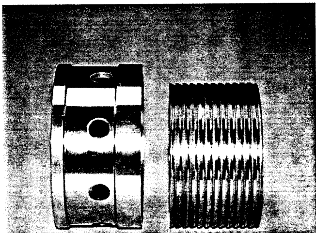
Figure 13. Original Center Bushing.
