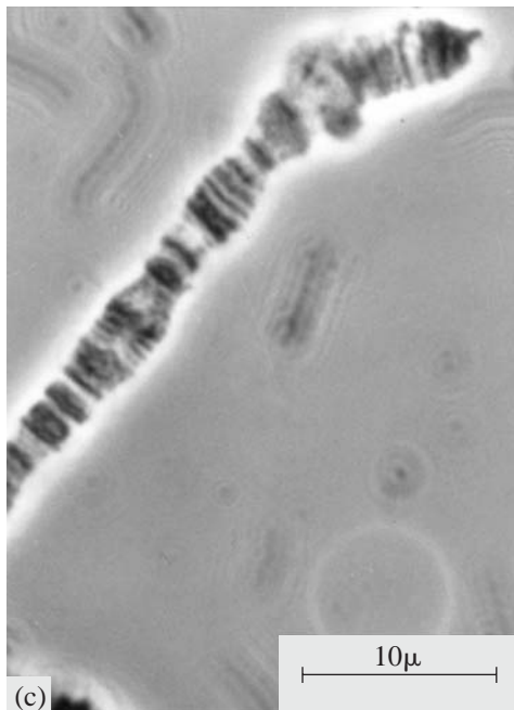
Figure 1.4 Polytene chromosomes from the salivary gland of a fruit fly, as seen in the electron microscope. Length scales: 100 000 Å or 10 \mu m. Courtesy of Ron Hill and Margaret Mott.
