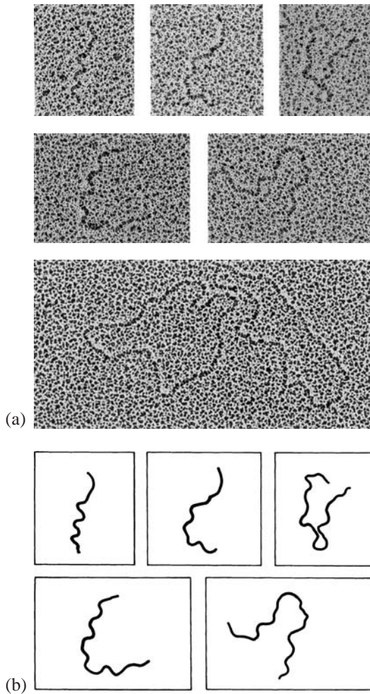
Figure 5.5 Electron micrographs of repeating-sequence DNA. The first five frames in (a) show an assortment of pictures of repeating-sequence, curved DNA of size about 1000 base-pairs. The last frame in (a) shows two DNA plasmid or ring molecules of size 3000 base-pairs, that have been included as controls. In (b), approximate tracings of the curved DNA molecules from (a) are presented. Courtesy of Margaret Mott.
