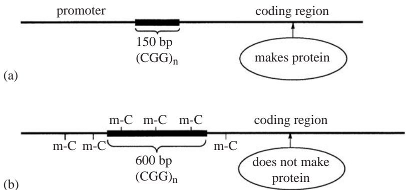
Figure 10.8 (a) When the FMR1 gene contains a repeat of (CGG)_n less than 150 base-pairs long, that DNA still works normally to make RNA and protein. (b) But when the FMR1 gene contains a repeat of (CGG)_n more than 600 base-pairs long, the expanded repeat somehow triggers methylation of nearby promoter DNA (i.e. conversion of cytosine to methyl-cytosine) by cellular methylase enzymes; and so the gene no longer works to make RNA or protein in the normal amounts.
