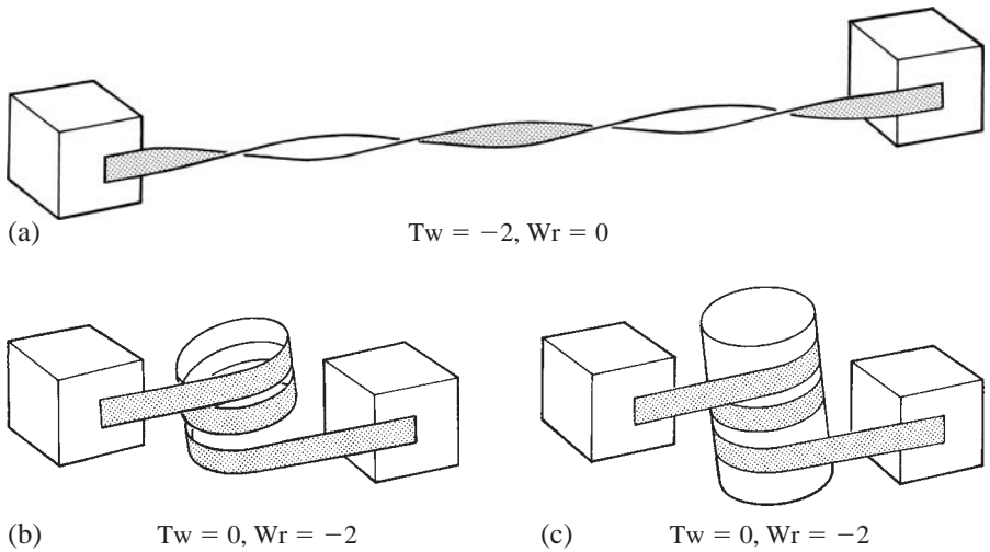
Figure 6.6 A highly twisted ribbon will collapse spontaneously into part of a toroidal supercoil. In (a), the two ends of the ribbon are held apart by their attachment to blocks, so that Tw = -2 . In (b), the blocks move together so that the ribbon can collapse to Wr = -2 . In (c), a cork or protein spool stabilizes the shape of the ribbon shown in (b).
