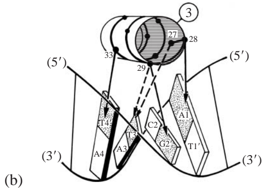
Figure 8.3 (a) A DNA base sequence which is recognized specifically by the 434 repressor protein. The four base-pairs on either end of this 14-base-pair sequence are shown in bold letters: they correspond to the four shaded base-pairs on each end of the DNA shown in Fig. 8.2(a), which are contacted directly by amino acids from \alpha -helix '3'. (b) A more detailed view of how amino acids 27, 28, 29, and 33 from \alpha -helix '3' contact different base-pairs within the major groove, at the sequence ACAA or TGTT shown in bold in (a). Hydrogen bonds between amino acids and base-pairs are drawn as continuous arrows, while hydrophobic contacts are drawn as dashed arrows.
