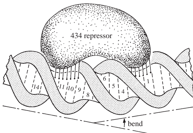
Figure 4.11 Schematic view of the binding of 434 repressor to DNA. This protein probes for the identities of base-pairs in positions 1 to 4 and 11 to 14 of its binding site, and also docks to the overall DNA conformation by testing the ease of curvature in positions 5 to 10. (More detail is shown in Fig. 8.2(a).)
