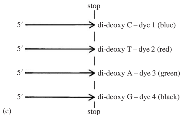
Figure 10.3 Key concepts from the di-deoxy, four-colour method of DNA sequencing: (a) comparison of three forms of nucleotide on an atomic scale; (b) comparison of chain extension by 2'-deoxy cytosine versus 2',3'-di-deoxy cytosine under the action of DNA polymerase; the chain extends normally if 2'-deoxy-C is added (and pairs with the guanine on the template), but stops or terminates if 2',3'-di-deoxy-C is added; (c) fluorescent dyes of four different colours can be attached to the four different di-deoxy nucleotides C, T, A and G, so that any particular product of chain termination will show just one color by capillary electrophoresis.
