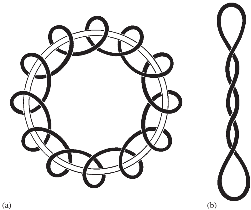
Figure 6.2 Two general varieties of DNA supercoil. In (a), the DNA coils into a series of spirals about an imaginary toroid or ring (shown here by open lines); and so this kind of wrapping is known as ‘toroidal’. In (b), the DNA crosses over and under itself repeatedly; and so this kind of wrapping is known as ‘interwound’.
