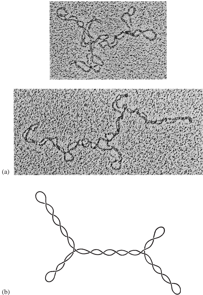
Figure 6.7 (a) Electron micrographs of negatively supercoiled, interwound DNA as prepared in pure form from E. coli bacteria. Each DNA plasmid or ring is 7000 base-pairs long, and has a mean Lk = -40 . Courtesy of Christian Boles, Nick Cozzarelli, and James White; and from Journal of Molecular Biology (1990) 213 , 931–51. (b) Branched path of the interwound DNA shown in (a), in schematic form. Such branching has little effect on the parameters Lk , Tw , and Wr .
