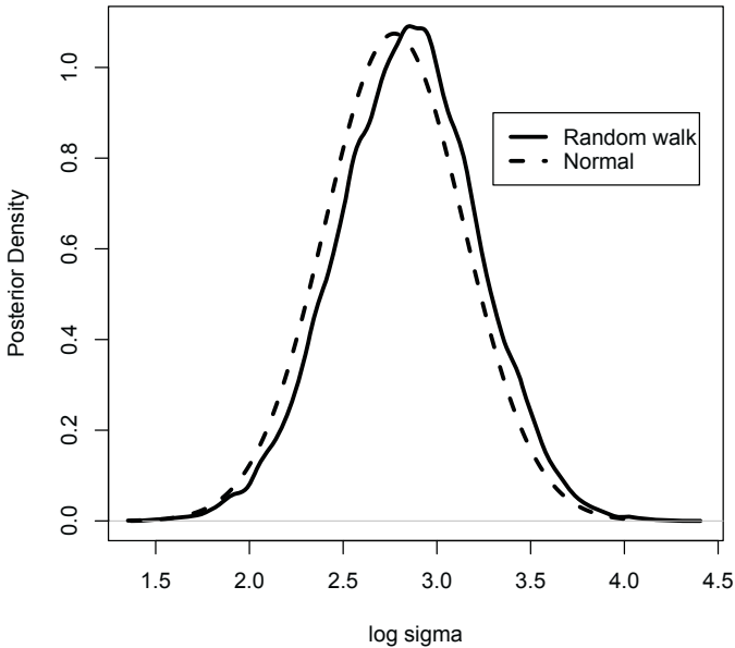
Fig. 6.10. Posterior density of \log \sigma using the normal approximation and simulated draws from the Metropolis random walk chain.
