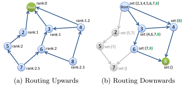
Figure 1: ORPL routes packets using multiple forwarders opportunistically. Routing upwards is done along a gradient. Routing downwards is done by going away from the root along nodes that have the destination in their routing set (either a bitmap or a Bloom filter).
