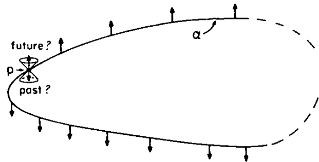
Fig. X.1 (Non-temporally orientable space-time)
