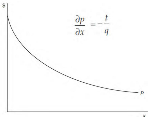
Figure 2.3 Housing-price curve.
