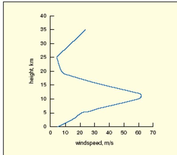
Figure 1. Typical Jet-Stream wind profile v/s altitude [1]
