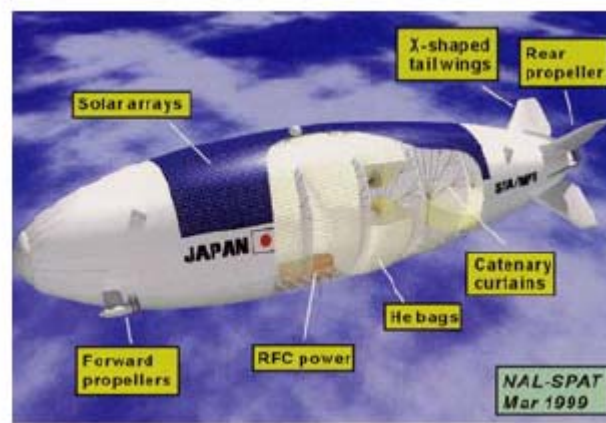
Figure 3: Artist's rendering of Japanese Stratospheric Platform System [7]
