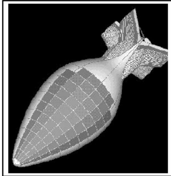
Figure 2. Solar cells placed on the HALE Airship platform envelope [5]
