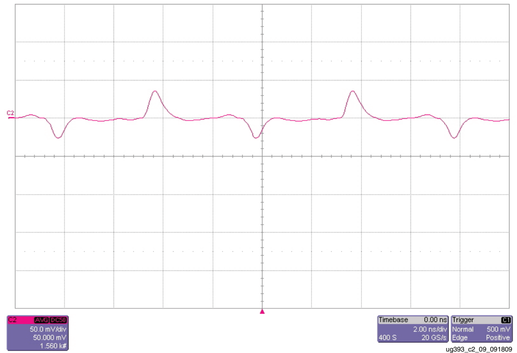
Figure 2-9: Averaged Measurement of V_{CC0} Supply with Multiple I/O Sending Patterns at 250 Mb/s
