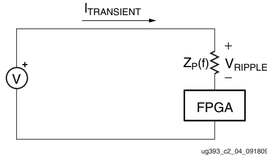
Figure 2-4: Further Simplified PDS Circuit
