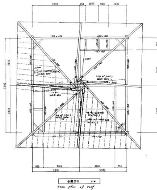
▲ 8.13 Roof plan. (Drawing: Yoichi Kan.)
