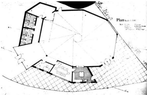
▲ 3.5 Community hall design – plan view.
