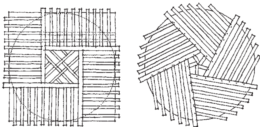
▲ 2.16 Example of a grillage structure (a) over a square plan and (b) over a circular plan. (Sketches by A. E. Piroozfar.)
