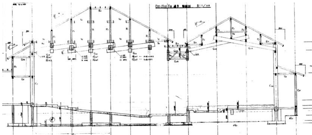
▲ 7.48 Section through the auditorium and stage. (Drawing: Tadashi Hamauzu.)
