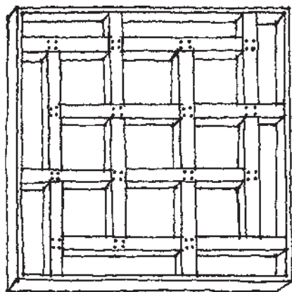
▲ 2.13 Serlio's solution for a 15-foot ceiling. (Sketch by A. E. Piroozfar.)
