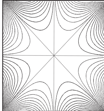
(Displacement Contours, a/b = 1.0 )
