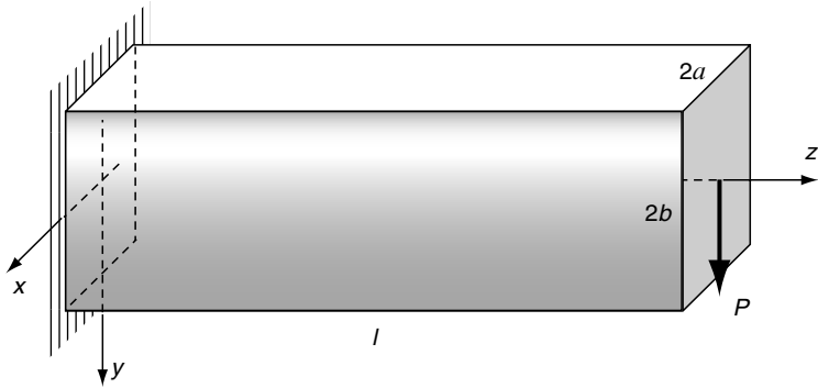
Figure 9-21 Flexure of a beam of rectangular section.
