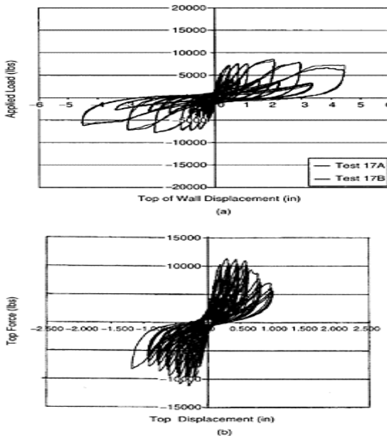
FIGURE 18.26 Variability in shear wall component test results, (a) Pardoen et al. Test 17
