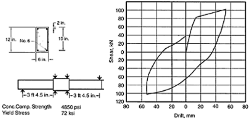
FIGURE 13.5 Load-deflection curve for a reinforced concrete beam with moment constantly changing along its span
