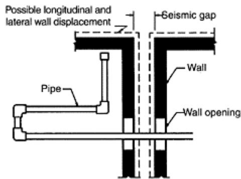
FIGURE 19.26 Detail (plan view) to provide for pipe crossing seismic gap. (Adapted from Sabol, T.A. (1989). Design of nonstructural systems and components, in Seismic Design Handbook , Naeim, F., Ed., Van Nostrand Reinhold, New York, chap. 12. With permission.)
