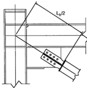
FIGURE 16.42 Unbraced length of gusset connection. (Tsai, K.C., Hwang, Y.C. and Weng, C.S. (2004). Subassembly testing and analysis of buckling restrained brace for seismic resistance, Structural Engineering , 18 (in Chinese).)
