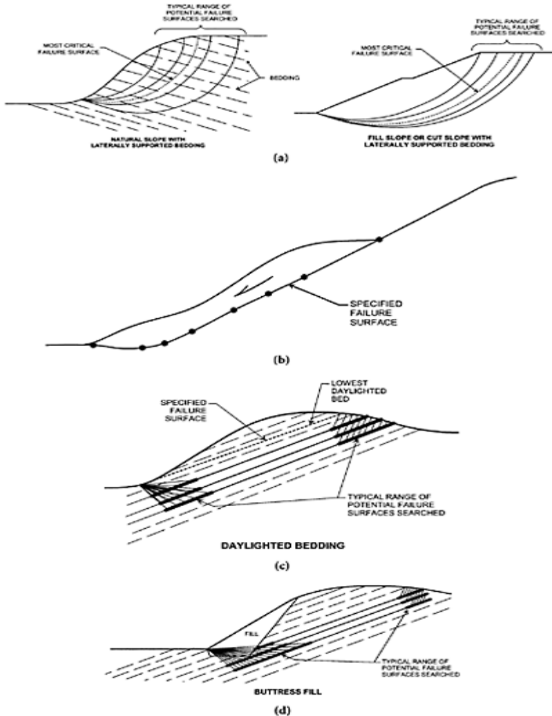
FIGURE 4.39 (a) Examples of use of circular failure surface geometry, (b) Example of use of specified failure
