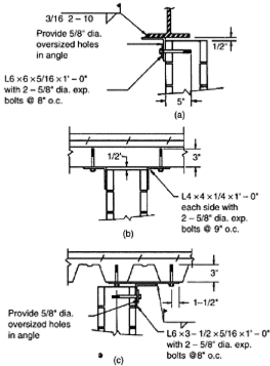
FIGURE 19.20 Details to separate nonbearing masonry wall from structure: (a) under steel beam; (b) perpendicular to steel deck; (c) parallel to steel deck. (Adapted from Sabol, T.A. (1989).
