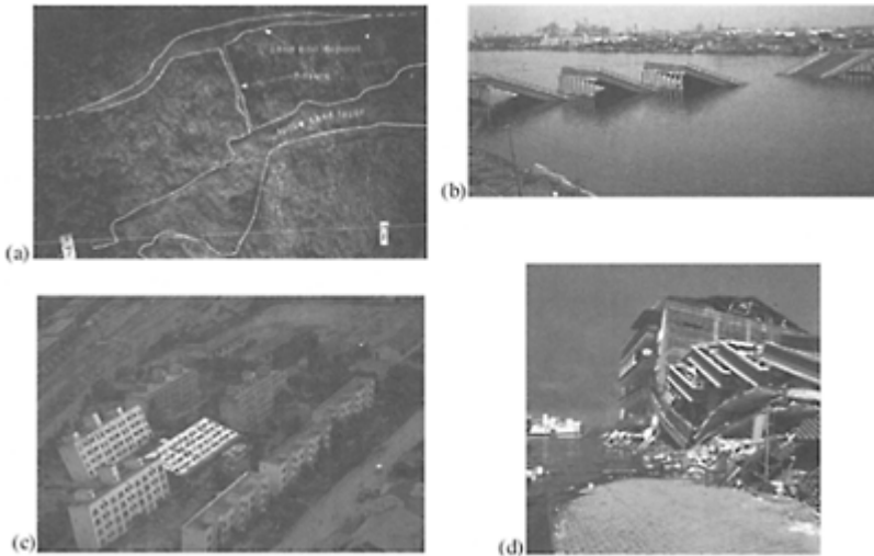
FIGURE 4.26 (a) Paleo-evidence of liquefaction in the form of buried sand boil (photo: U.S. Geological Survey), (b) lateral spreading damage to Showa bridge from 1964 Niigata earthquake (photo: J.Penzi), (c) bearing failure of foundations for Kawagishi-cho apartment buildings in 1964 Niigata earthquake (photo: J.Penzi), (d) subsidence of waterfront area in 1999 Turkey earthquake (photo: K.Elwood).
