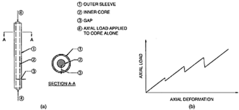
FIGURE 16.22 Concept of sleeved column and typical behavior, (a) Components of sleeved column; (b) typical compression behavior. (Adapted from Prasad, B. (1992). Proc. 33rd AIAA Structures, Structural Dynamics and Materials Conference , Dallas, TX. With permission.)
