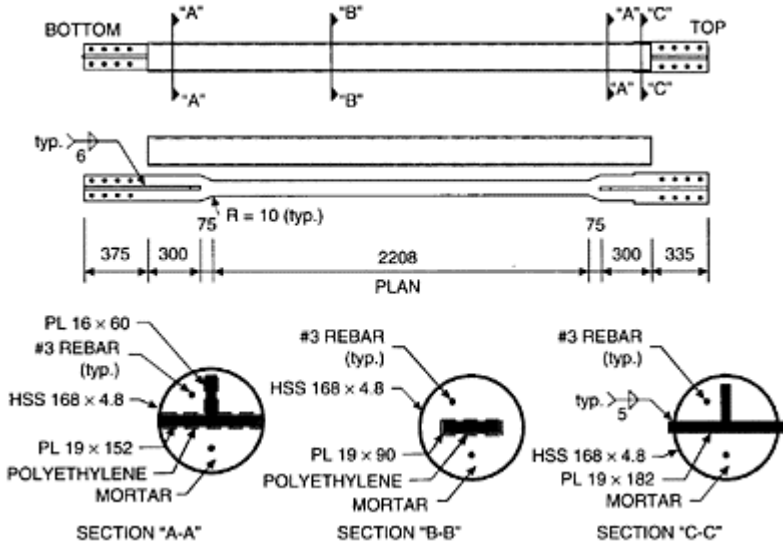
FIGURE 16.38 Details of buckling-restrained brace. (Tremblay, R., Degrange, G. and Blouin, J. (1999). Seismic rehabilitation of a four-story building with a stiffened bracing system, Proc. 8th Canadian Conference on Earthquake Engineering, Vancouver, BC, 549–554.)
