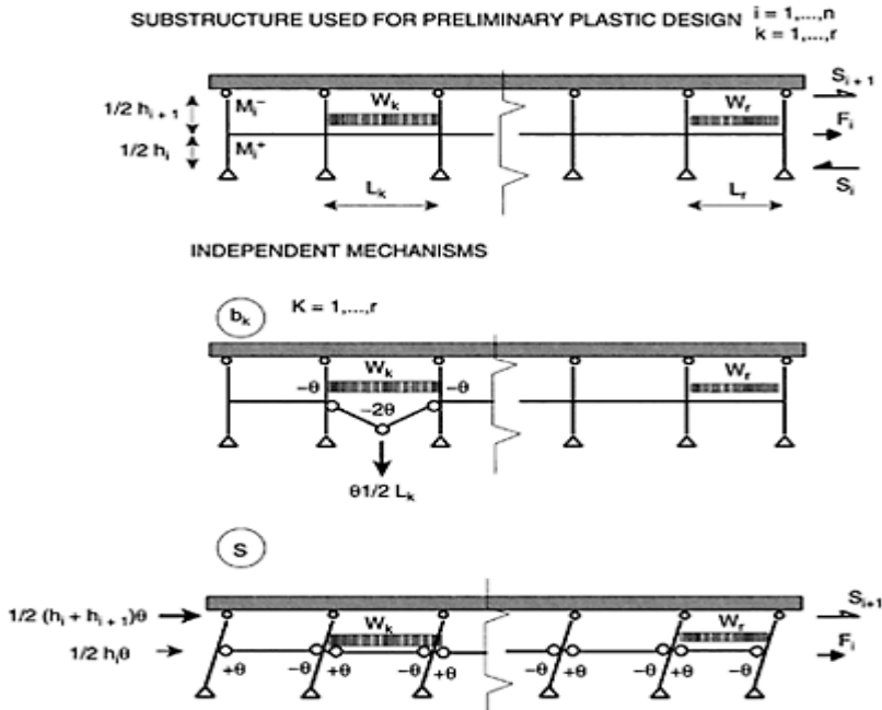
FIGURE 8.9 Substructure used for preliminary plastic design and independent mechanisms.
