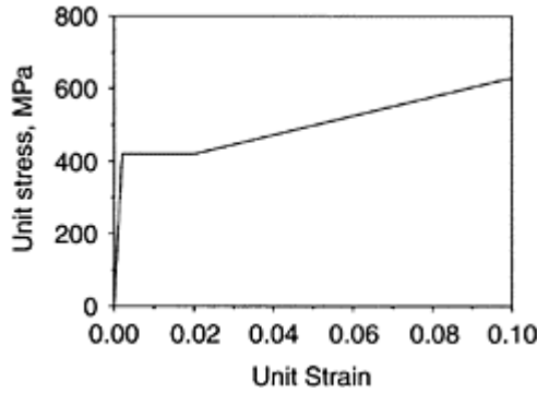
FIGURE 13.9 Representative idealized stress-strain relationship for steel reinforcement.
