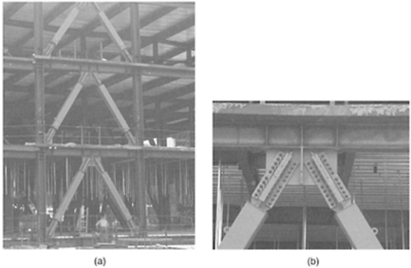
FIGURE 16.8 Buckling-restrained brace frames for new construction, (a) Elevation; (b) connection details (courtesy of SIE, Inc.).
