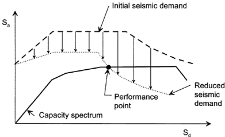
FIGURE 4.25 Use of capacity and demand spectra to define performance point. (Adapted from Comartin, C.D.)
