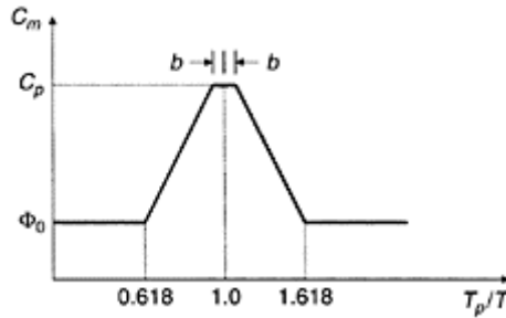
FIGURE 19.15 Variation of modified amplification factor with natural period ratio.
