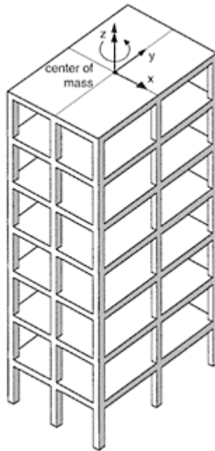
FIGURE 14.12 Three-dimensional model with three degrees of freedom per story.
