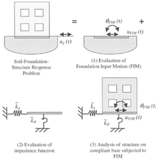
FIGURE 4.15 Substructure approach to analysis of the soil-structure interaction problem.
