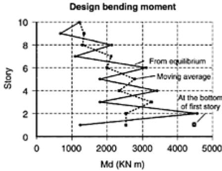
FIGURE 8.28 Design bending moment for exterior column.
