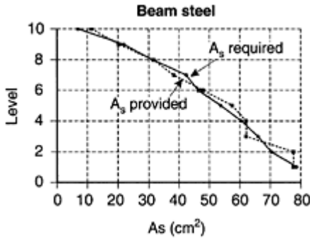
FIGURE 8.24 Required and provided beam reinforcement.
