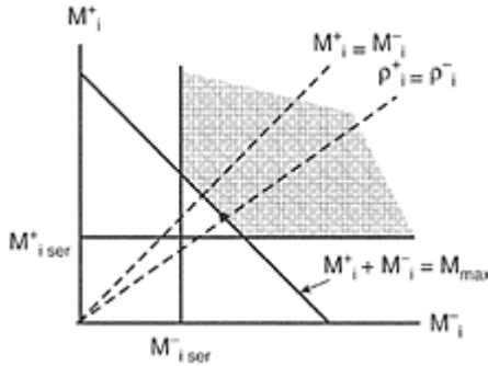
FIGURE 8.23 Optimization problem to design beam reinforcement.
