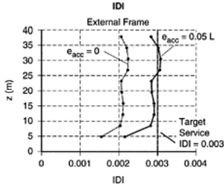
FIGURE 8.39 3D linear elastic response spectrum analysis of external frame IDI.
