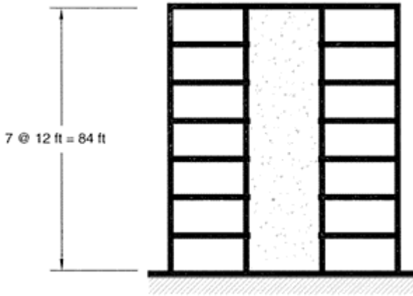
FIGURE 13.3 Frame with dominant wall.
