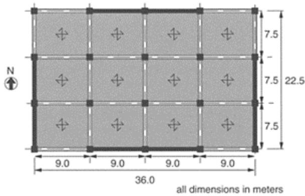
FIGURE 14.47 Two-bay wall scheme studied in (Garcia, 1996).
