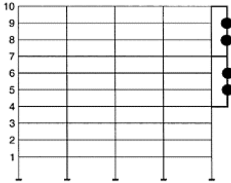
FIGURE 19.14 Example of nonstructural element connected to multiple points of supporting structure.
