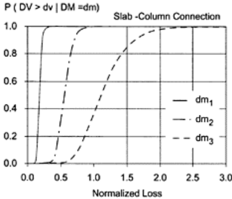
FIGURE 9.38 Probabilities of exceeding a normalized loss in slab-to-column connections conditioned on being in a certain damage state.
