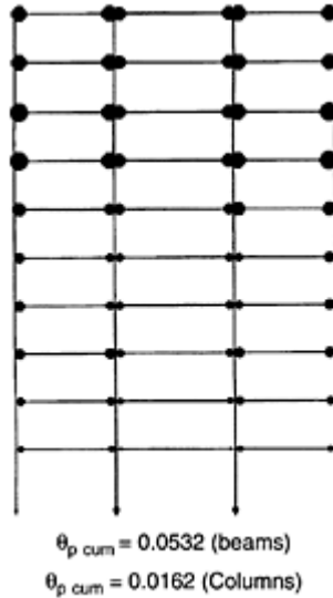
FIGURE 8.56 Time-history analysis: cumulative plastic hinge rotations.
