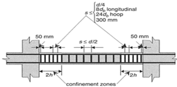
FIGURE 14.28 Hoop spacing in girders.
