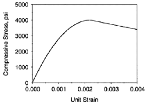
FIGURE 13.8 The Hognestad stress-strain relationship for unconfined concrete in compression.
