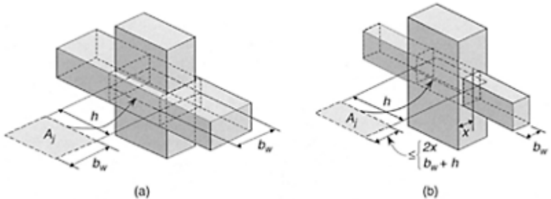
FIGURE 14.36 Definition of A_j for joint shear determination.
