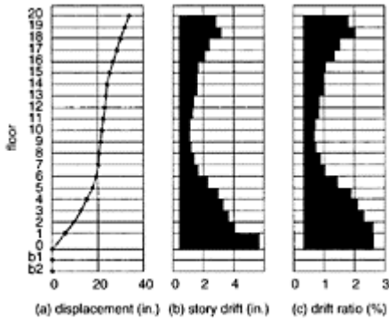
FIGURE 6.30 Envelope of maximum floor displacement and story drift for 20-story building due to horizontal ground motion.
