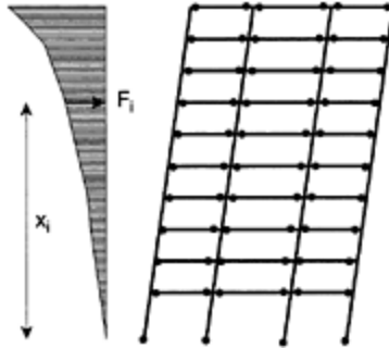
FIGURE 8.50 Estimation of V_{mech} using plastic analysis.
