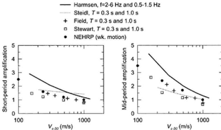
FIGURE 4.10 Averaged median spectral amplification versus V_{s-30} from various investigators (Harmsen, 1997; Field, 2000; Steidl, 2000; Stewart et al,
