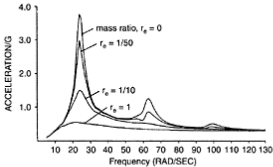
FIGURE 19.10 Floor response spectra for fourth floor of six-story building in Figure 19.11 corresponding to different nonstructural to structural mass ratios. (Adapted from Singh, M.P. and Suárez, L.E., Earthquake Eng. Struct. Dyn. , 15, 871–888, 1987. With permission.)
