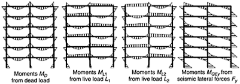
FIGURE 14.15 Moment diagrams obtained from frame analysis due to gravity and lateral loads.
