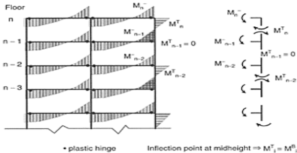
FIGURE 8.14 Zig-zag pattern of design bending moments and shear for columns.
