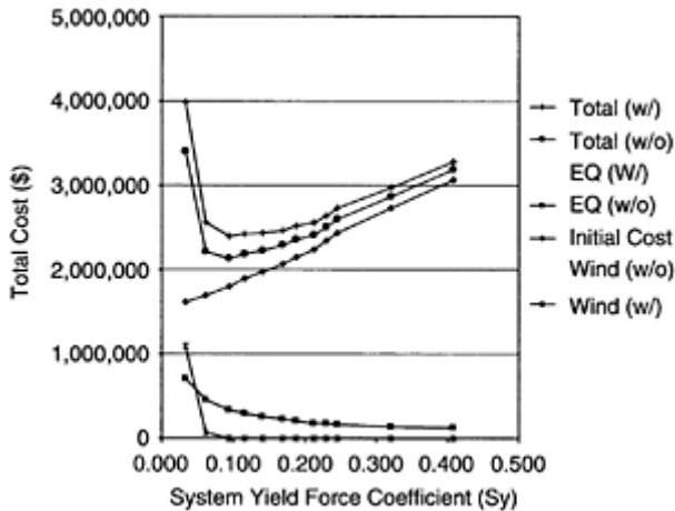
FIGURE 7.9 Life-cycle costs of a nine-story office building as function of system yield force coefficient at Seattle (life=50 year, discount rate=5%, w/ and w/o indicate with and without consideration of costs due to deaths and injuries). (Kang and Wen, Structural Research Series No. 629, University of Illinois at Urbana-Champaign, 2000.)
