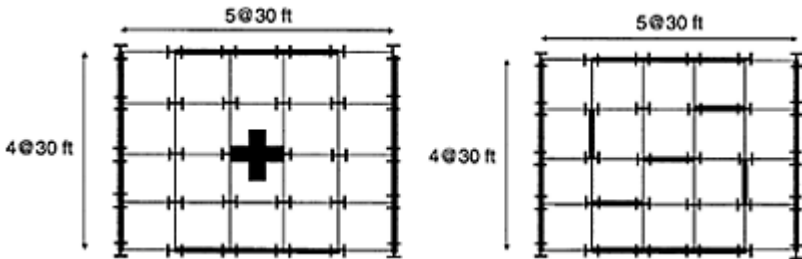
FIGURE 7.12 Plane of five-story two-way dual systems with equal total lateral resistances.
