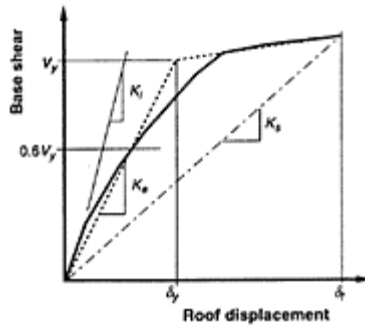
FIGURE 12.12 Calculation of secant stiffness at maximum displacement (FEMA 1997).
