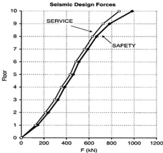
FIGURE 8.22 Distribution of design service and safety earthquake loads for external frames.
