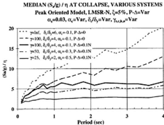
FIGURE 9.29 Effect of combinations of deterioration parameters on median collapse capacity. (Ibarra, L., Medina, R. and Krawinkler, H. (2002). Collapse assessment of deteriorating
