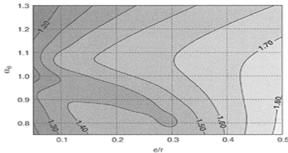
FIGURE 8.18 Maximum displacement ratio between two and one DOFS (hyperbolic spectrum, rectangular plant L=2D ).
