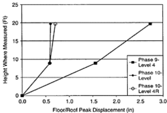
FIGURE 18.21 Vertical distribution of deformation demand in UC San Diego House. (From Cobeen et al., 2003, CUREE Publication W-30, CUREE, Richmond, CA. With permission.)
