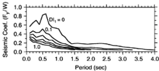
FIGURE 5.23 Strength spectra for constant values of damage index ( DI_1=0, 0.1, 0.2, 0.4, 0.6, 1.0 ) for an elastic-perfectly-plastic SDF system with 5% damping subjected to the El Centre (NS) recording of the 1940 Imperial Valley, California, earthquake. (From Bozorgnia, Y. and Bertero, V.V., 2002. Improved damage parameters for post-earthquake applications. Proc. SMIP02 Seminar on Utilization of Strong-Motion Data , Los Angeles, 61–82.)
