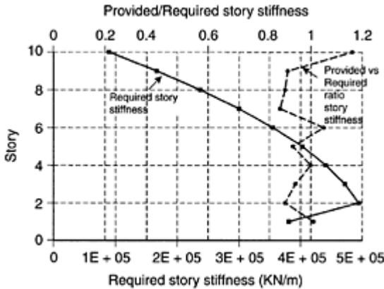
FIGURE 8.19 Required and provided story stiffness.
