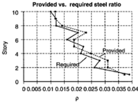
FIGURE 8.30 Provided and required steel ratio for exterior column.
