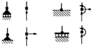
FIGURE 6.2 Typical support symbols for the 2d case.
