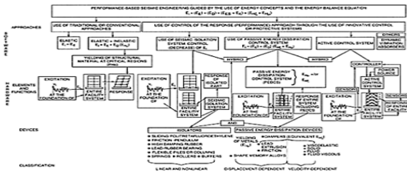
FIGURE 10.3 Flow chart of the conventional and innovative approaches, strategies and techniques for P-BSD. (From Bertero, V.V., 1997,
