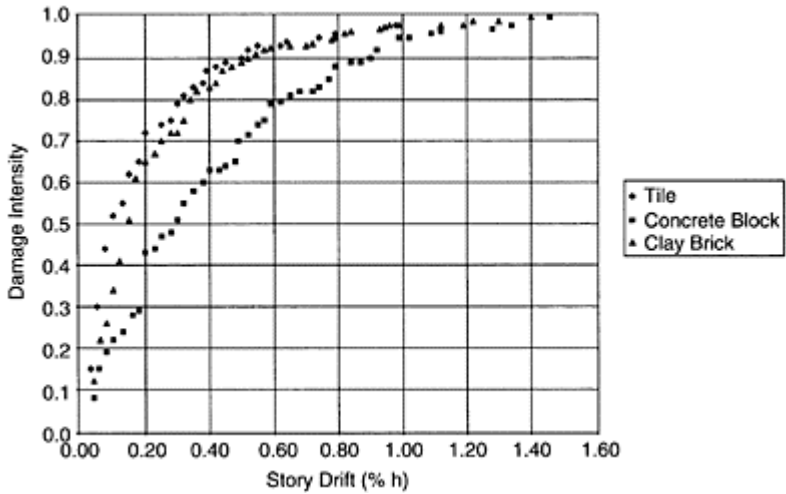
FIGURE 14.19 Damage intensity versus story drift index for masonry partitions.
