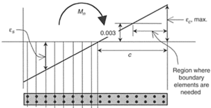
FIGURE 14.39 Strain state at the critical wall section.
