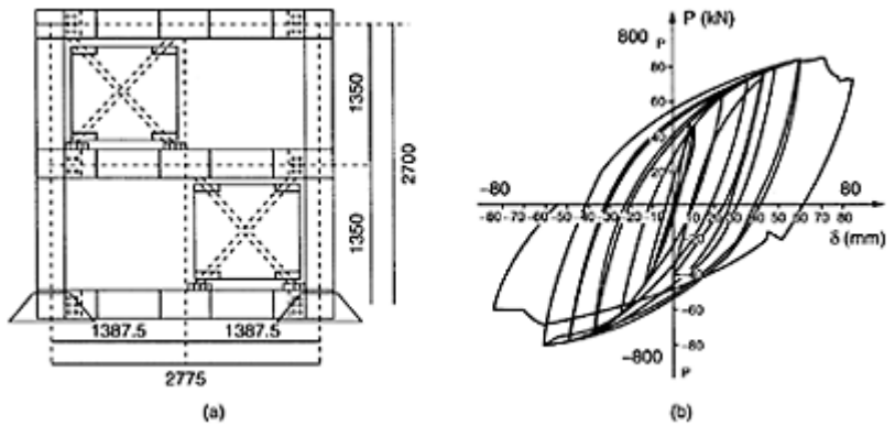
FIGURE 16.16 System test of budding-restrained braces sandwiched between precast concrete panels, (a) Test setup; (b) hysteresis behavior.
