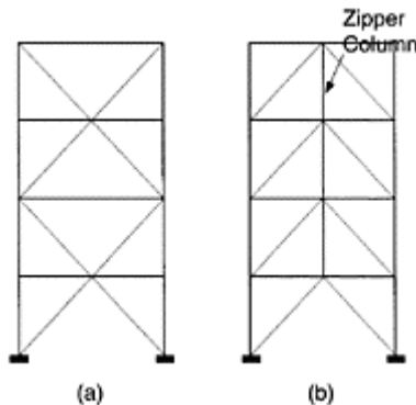
FIGURE 16.2 Configurations that mitigate unbalanced loads in beams (AISC (2002). Seismic Provisions for
