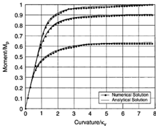
FIGURE 6.22 Moment-curvature relation for rectangular section with elastic-perfectly plastic material; analytical and numerical solution with
