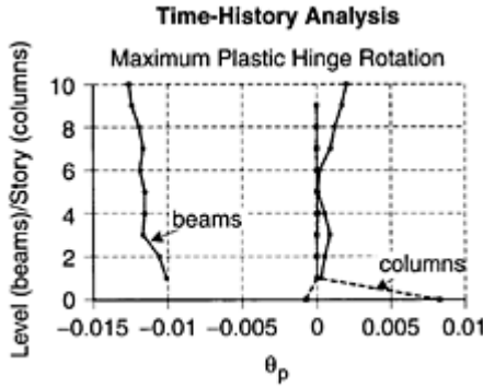
FIGURE 8.53 Maximum plastic hinge rotations for time-history analysis.
