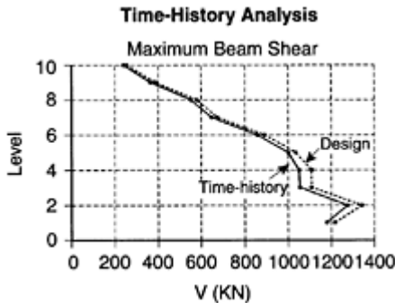
FIGURE 8.58 Time-history and design beam shear.
