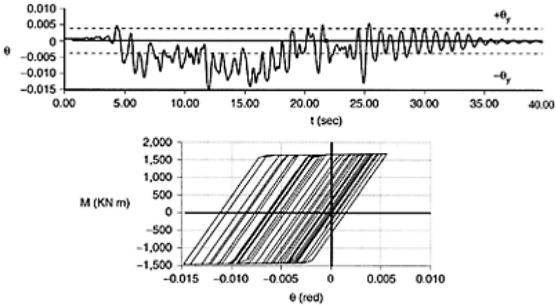
FIGURE 8.63 Moment vs rotation of the end of the beam located at the eighth level and left span.
