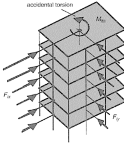
FIGURE 14.13 Six-story building subjected to seismic forces Q_E along the principal axes plus accidental torsion.
