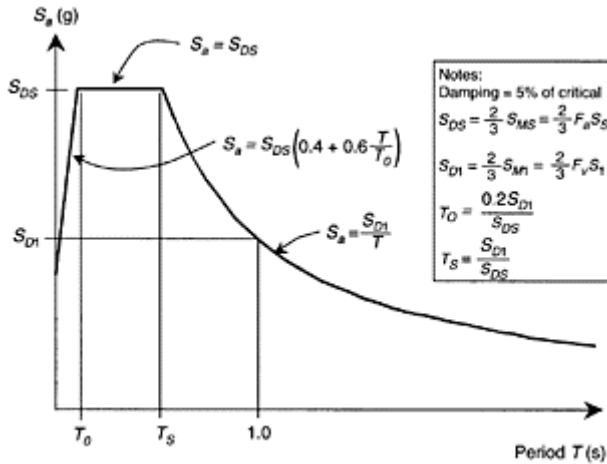
FIGURE 14.9 Design acceleration response spectrum.
