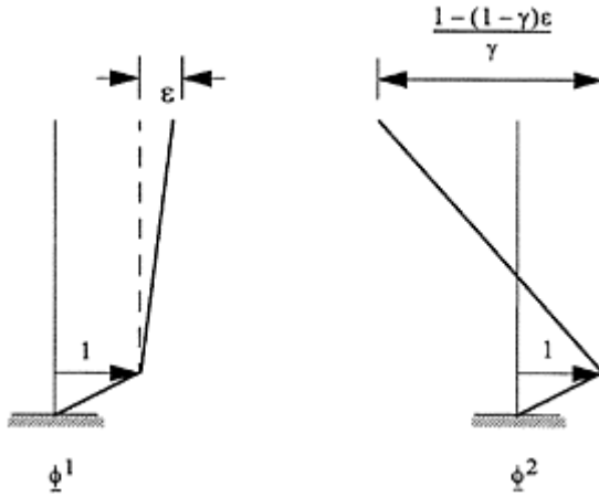
FIGURE 11.7 Mode shapes of two-degree-of-freedom isolation system model.
