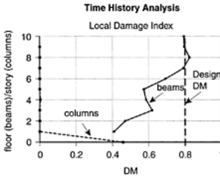
FIGURE 8.62 Maximum damage index at each level from time-history analysis.
