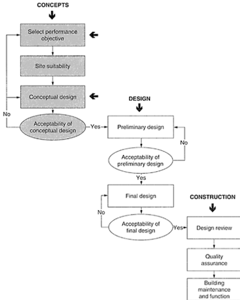
FIGURE 10.1 Conceptual framework for P-BSE. (Adapted from SEAOC Vision 2000 Committee (1995). Performance-based seismic engineering of buildings. Report, Structural Engineers Association of California, Sacramento, CA.)
