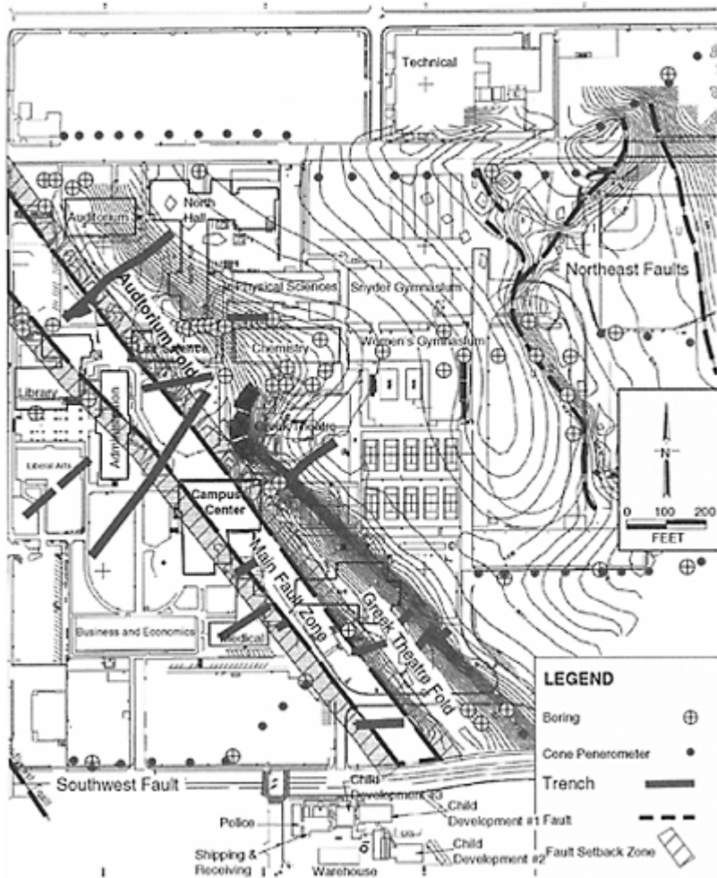
FIGURE 3.6 Map of part of campus of San Bernardino Valley College, crossed by the San Jacinto active fault, locating trenches, borings and cone penetrometer sites, recommended setbacks and location of secondary faults as of the beginning of 1999. Contours are on a stream terrace surface 10,000 years old; contour interval 1 foot. See also color insert
