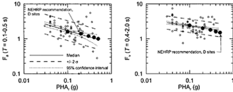
FIGURE 4.9 Averaged spectral amplification versus reference motion peak acceleration ( PHA_r ) for Northridge earthquake recordings at D sites (Borcherdt, 2002), as compared to NEHRP site factors (BSSC, 2001). Note: Reference motions for NEHRP factors modified from published values according to PHA_r = S_s / 2.5 (for F_a ) and PHA_r = S_1 (for F_v ).
