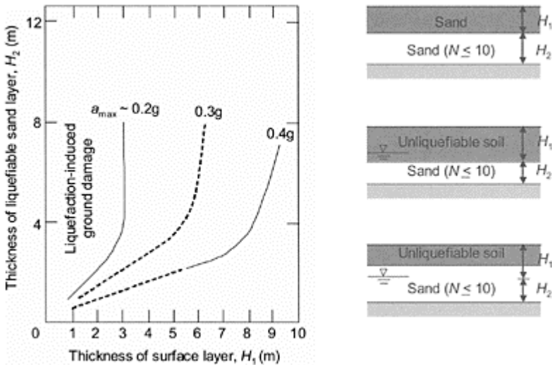
FIGURE 4.33 Empirical relationships for estimating conditions under which surficial evidence of liquefaction can be expected. Surficial evidence can be expected for H_1-H_2 pairs that plot above each of the indicated curves. (From Ishihara, K., Proceedings, Eleventh International Conference on Soil Mechanics and Foundation Engineering , 1, 321–376, 1985. With permission.)
