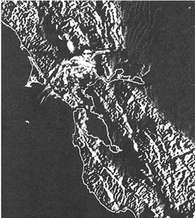
FIGURE 2.8 Computed ground motions generated by constant velocity rupture northward of the Hayward fault (red line). Wave intensities defined by color intensities. See also color insert following page 2–30. (courtesy of D.Dreger).
