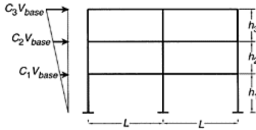
FIGURE 13.13 Story-force distribution assumed for a planar three-story frame.
