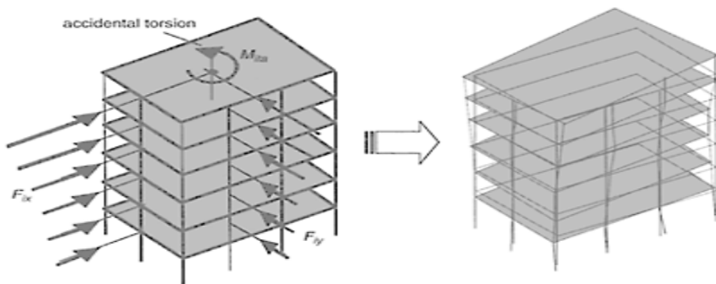
FIGURE 14.17 Lateral deflections of a building due to orthogonal and torsional effects.
