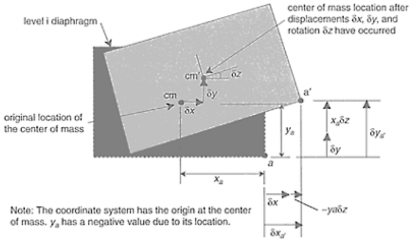
FIGURE 14.18 Location of a point within the diaphragm after lateral deflection have occurred.
