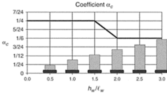
FIGURE 14.37 Coefficient \alpha_c for wall shear design.
