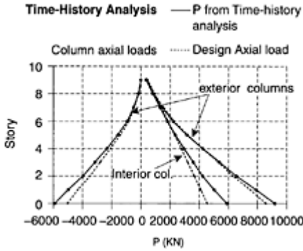
FIGURE 8.60 Time-history and design column axial loads.
