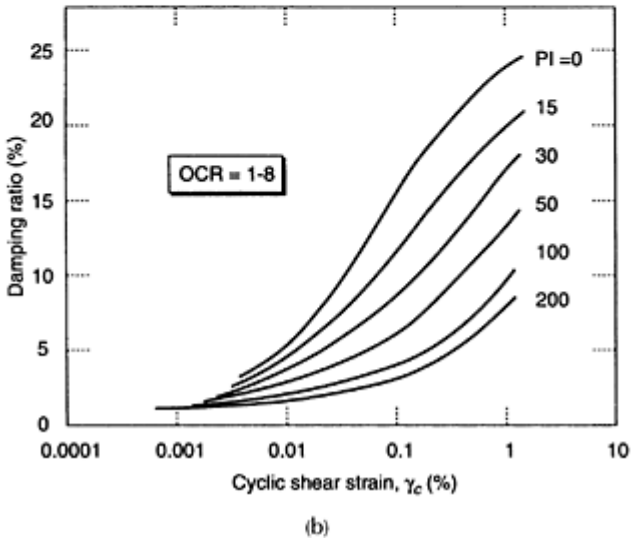
FIGURE 4.5 Vucetic-Dobry model: (a) modulus reduction curves and (b) damping curves. (From Vucetic, M. and Dobry, R. J. Geotech. Engrg. , ASCE, 117, 89–107, 1991. With permission.)
