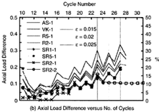
FIGURE 16.34 Duckling-restrained brace effect of unbending materials on axial load difference. (Tsai, K.C. and Lai, J.W. (2002). A study of buckling restrained seismic braced frame, Structural Engineering , 17(2), (in Chinese).)
