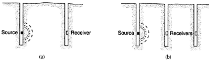
FIGURE 4.2 Configurations for cross-hole seismic test: (a) single receiver, and (b) multiple receivers.
