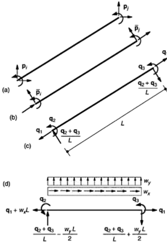
FIGURE 6.4 Element forces in global, local and basic reference systems.
