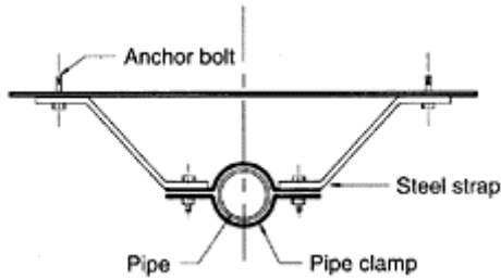
FIGURE 19.27 Pipe clamp and sway bracing. (Adapted from Sabol, T.A., Design of nonstructural systems and components, in Seismic Design Handbook , Naeim, F., Ed., Van Nostrand Reinhold, New York, 1989. With permission.)
