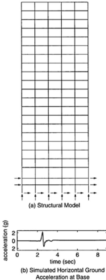
FIGURE 6.27 Model for 20-story moment-resisting frame (Gupta and Krawinkler, 1999) and ground motion for simulations.
