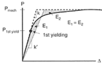
FIGURE 8.7 Stiffness of an equivalent SDOF system.
