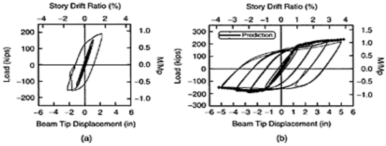
FIGURE 15.14 Load versus beam tip deflection relationships of the composite specimens (Yu, Q.-S., Noel, S. and Uang, C.-M. (1997).
