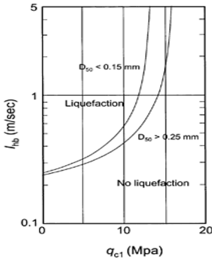
FIGURE 4.32 Variation of Arias intensity required to trigger liquefaction with corrected cone penetration resistance, q_{c1} . (Modified
