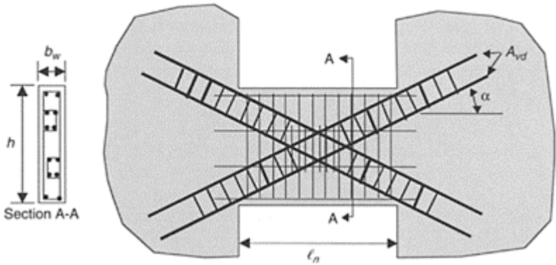
FIGURE 14.40 Wall coupling beam with diagonal reinforcement.
