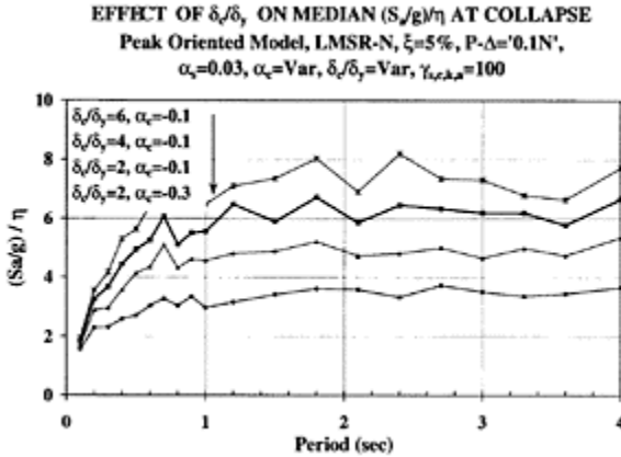
FIGURE 9.27 Effect of \delta_c/\delta_y ratio on median collapse capacity. (Ibarra, L., Medina, R. and Krawinkler, H. (2002). Collapse assessment of deteriorating SDOF systems. Proc. 12th European Conference on Earthquake Engineering , London, Paper Reference 665. With permission.)
