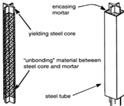
FIGURE 16.10 Concept of a type of buckling-restrained brace (Adapted from Clark, P., et al. (1999). Proc. 69th Annual SEAOC Convention , Sacramento, CA. With permission.)
