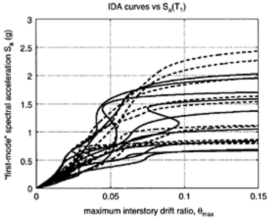
FIGURE 7.7 Results of incremental dynamic analysis of nine-story steel moment-resisting frame with fracturing connection under SAC ground motions (Vamvatsikos and Cornell, J. Earthquake Eng. Struct. Dyn. , 31, 491–514, 2002.).
