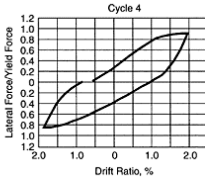
FIGURE 13.19D A force-displacement relationship in a cycle of applied displacement for
