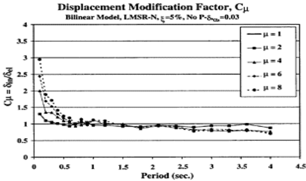
FIGURE 9.9 Ratio of displacements of inelastic to elastic bilinear SDOF systems, for various ductility ratios.
