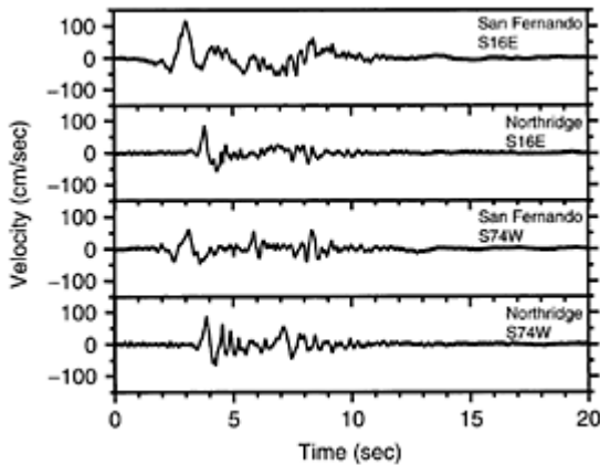
FIGURE 2.10 Ground motion velocity pulses at Pacoima Dam comparing the 1971 San Fernando, California, and 1994 Northridge, California, earthquakes.
