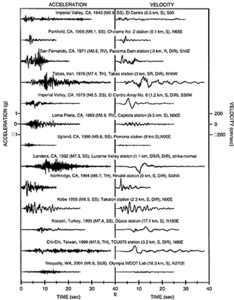
FIGURE 5.1 Selected recorded ground accelerations (plotted at the same scale), and the corresponding ground velocities. SS=strike-slip faulting; RV=reverse faulting; TH=thrust faulting; SUB=subduction intraslab earthquake; S=soil site; R=rock site; SR=soft rock site; DIR=record includes fault rupture directivity effects. Distance measure is
