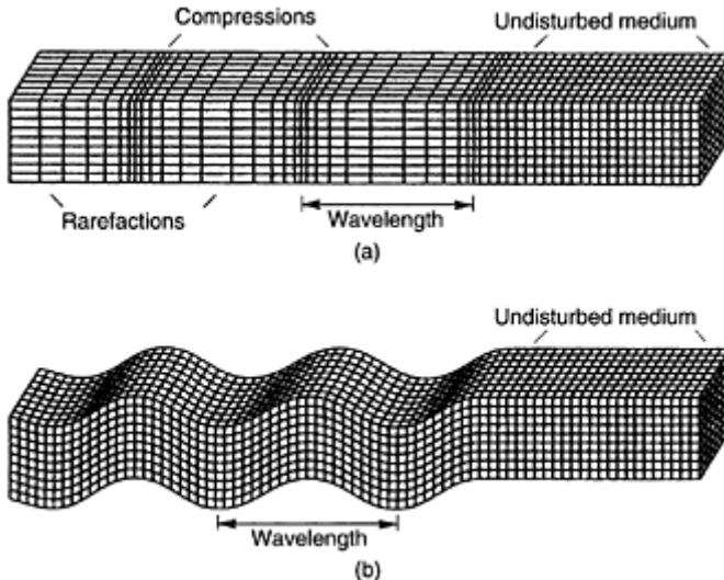
FIGURE 2.4 Deformation produced by body waves (a) P-wave; (b) SV- (vertically polarized) wave (Bolt, B.A., 2003. Earthquakes . 5th ed.,
