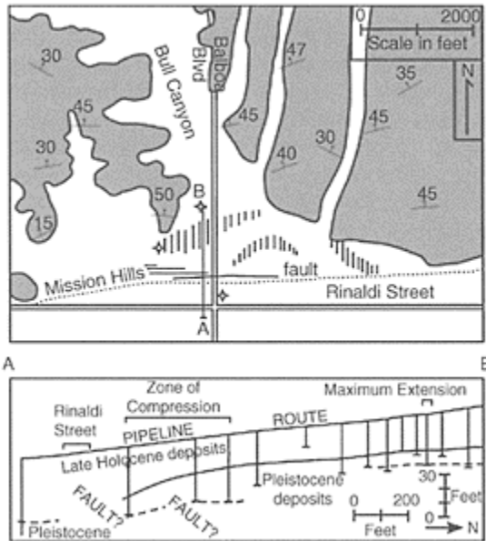
FIGURE 3.9 (Top) Geologic map of Balboa Boulevard, where pipelines ruptured in the 1994 Northridge earthquake. Geology modified from Shields (1977) and Dibblee (1991; 1992). Bedrock is shaded, with arrows in direction of dip of strata. Clear areas covered by late Quaternary alluvial deposits. Open circles with crosses show oil-well control for location of Mission Hills fault. Vertical lines, areas of extension; horizontal lines, areas of compression in 1994 earthquake. A-B locates cross section (bottom) with linear array of CPT and SPT soundings to define shallow geologic units, including boundary between Pleistocene and Holocene alluvial deposits. Modified from Holzer et al. (1999).
