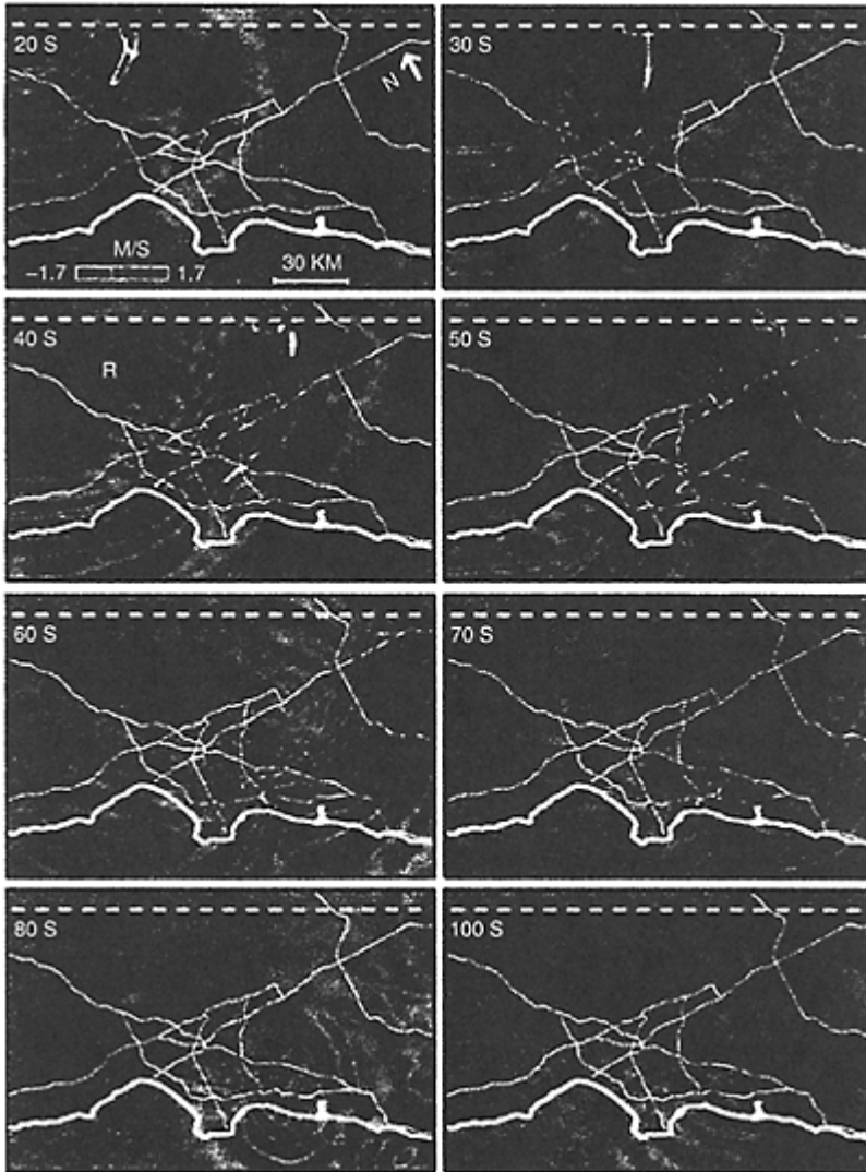
FIGURE 2.13 Snapshots of simulated wave propagation in the Los Angeles area for hypothetical earthquake; the snapshots depict the horizontal particle velocities that represent shaking parallel to the San Andreas fault from 20 sec to 100 sec after the origin time of the rupture. Red depicts large
