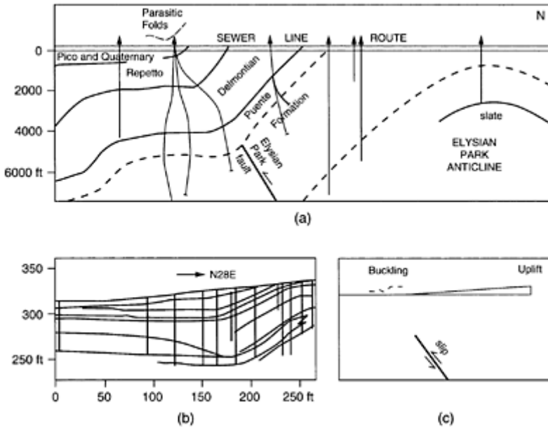
FIGURE 3.8 Diagrammatic cross section along Los Angeles sewer line route following the Los Angeles River. Bedrock formations are based on oil well control (derrick symbol, straight and curved lines). Parasitic folds related to bending moment (Oskin et al., 2000) are found at the boundary between flat-lying strata (left) and the south flank of the Elysian Park anticline (right). Slip on the blind Elysian Park fault would result in an increase in gradient between the crest of the anticline and the flat-lying strata to the left, in addition to buckling of the parasitic folds, (b) Parasitic fold at the Coyote Pass escarpment, with vertical lines showing borehole control, after Oskin et al. (2000). Buckling during an earthquake would be concentrated on parasitic folds like
