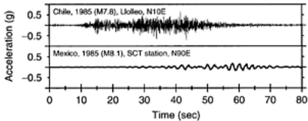
FIGURE 5.2 Ground accelerations recorded during the March 3, 1985 Chile and September 19, 1985 Mexico earthquakes.
