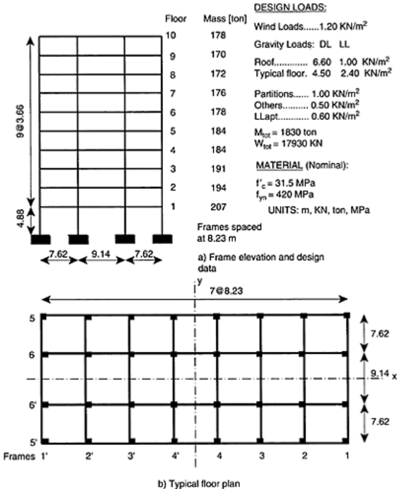
FIGURE 8.15 General configuration and structural lay-out.
