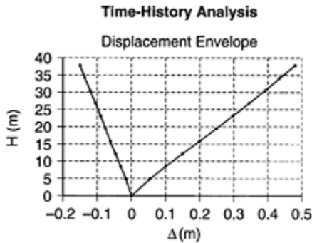
FIGURE 8.51 Displacement envelopes for time-history analysis.
