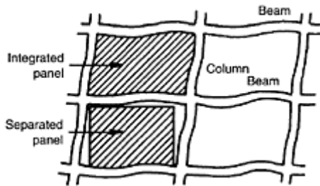
FIGURE 19.18 Separated and integrated infill panels in a framed structure.
