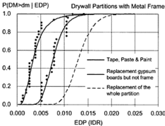
FIGURE 9.41 Fragility functions for three damage states of drywall partitions with metal frames.
