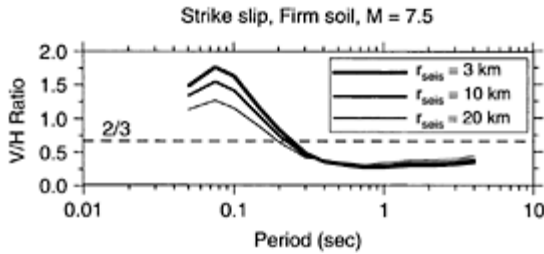
FIGURE 5.35 Vertical-to-horizontal (V/H) spectral ratio for 5% damping and distances from seismic faulting of 3, 10 and 20 km. (Adapted from Campbell, K.W. and Bozorgnia, Y. (2003). Updated near-source ground motion (attenuation) relations for the horizontal and vertical components of PGA and acceleration response spectra. Bulletin of the Seismological Society of America , 93, 314–331.)
