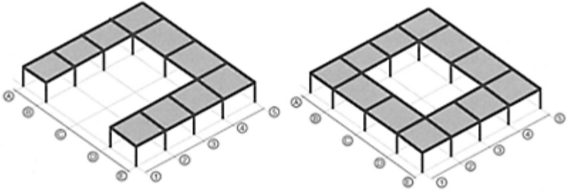
FIGURE 14.24 Examples of diaphragms not appropriate to be modeled as rigid diaphragms.
