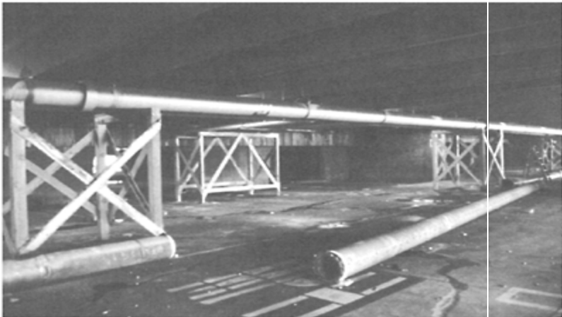
FIGURE 19.2 Collapse of pipe originally suspended from below
