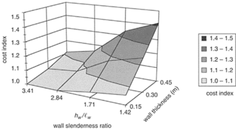
FIGURE 14.49 Wall, beam and column cost index for eight-story building having the plan layouts shown in Figures 14.46 and 14.47 and located in a moderate seismic zone studied in (Garcia, 1996).
