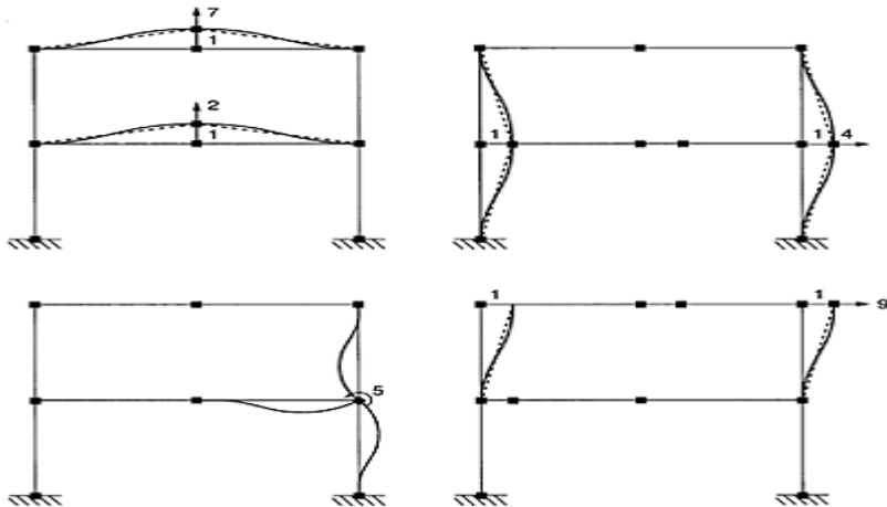
FIGURE 6.11 Typical deformed shapes for global DOFs of two-story frame.
