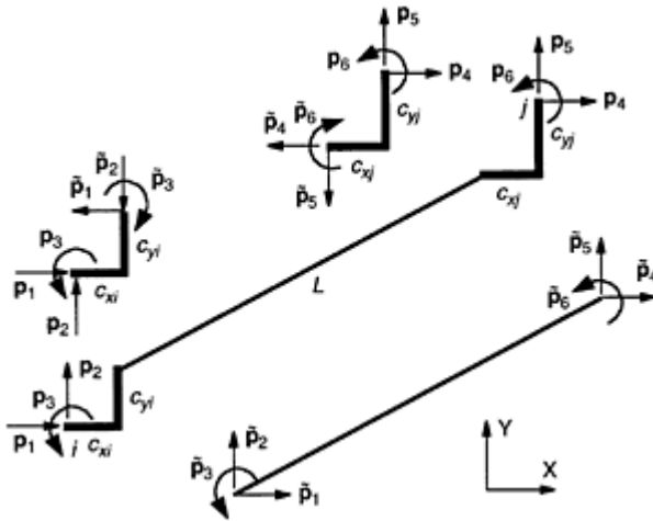
FIGURE 6.5 Force transformation (equilibrium) for rigid-end offsets.
