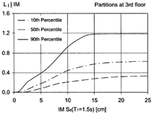
FIGURE 9.45 Variation of normalized losses in interior partition walls in the third story as a function of the level of ground motion intensity.
