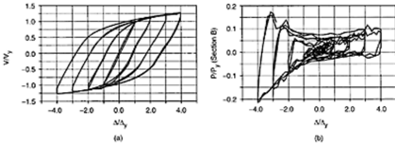
FIGURE 16.39 Measured hysteresis response, (a) Global response; (b) round hollow structural section casing response. (Tremblay, R., Degrange, G. and Blouin, J. (1999). Seismic rehabilitation of a four-story building with a stiffened bracing system, Proc. 8th Canadian Conference on Earthquake Engineering, Vancouver, BC , 549–554.)
