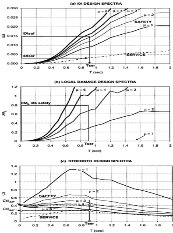
FIGURE 8.3 (a) IDI; (b) local damage; and (c) strength design spectra.
