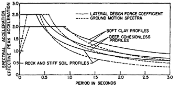
FIGURE 9.2 Comparison of ground motion spectra with design force coefficients (ATC-3-06, 1978).
