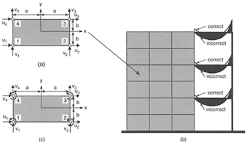
FIGURE 14.27 Use of finite elements in shear wall analysis.
