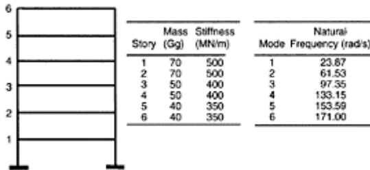
FIGURE 19.11 Properties and natural frequencies of six-story shear building considered in study of interaction and nonclassical damping effects. (Note: 1 Gg=68,525 slugs; 1 MN/m=737.5 kips/ft.)
