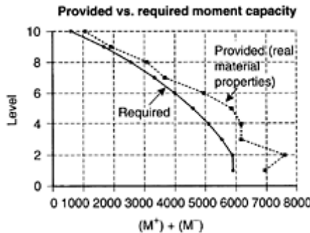
FIGURE 8.26 Required and provided beam moment capacity.
