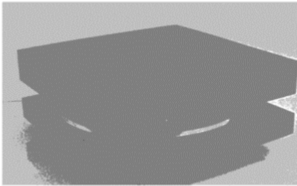
FIGURE 11.10 Example of a friction pendulum bearing (courtesy of Earthquake Protection Systems, Inc.).
