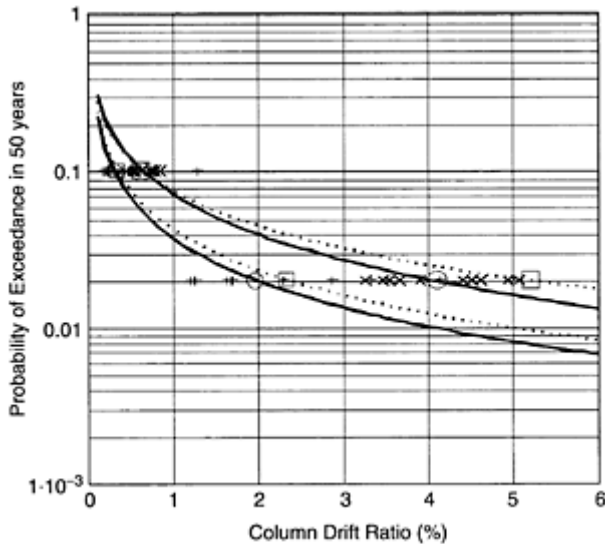
FIGURE 7.5 Probabilistic column drift ratio demand curve of a two-story steel moment frame building at Carbondale, IL before and after retrofit with shear walls (data points before retrofit [ \times ], after retrofit [ + ], median value ( o ) and median including
