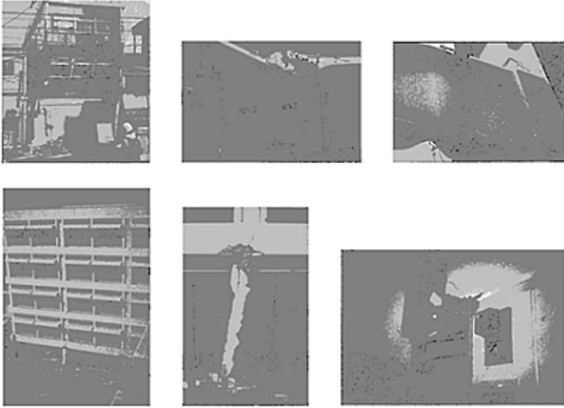
FIGURE 10.2 Photos illustrating significant damage to structures and structural components when they have to develop large ductilities.
