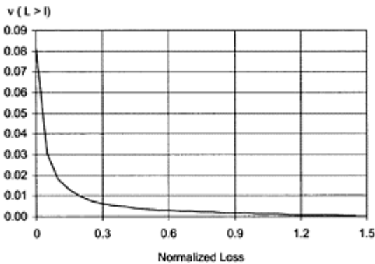
FIGURE 9.46 Normalized loss curve computed for a seven-story reinforced concrete building.
