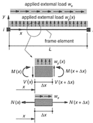
FIGURE 6.18 Equilibrium in undeformed configuration of frame element.
