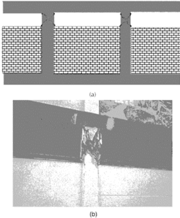
FIGURE 14.20 Captive column effect.
