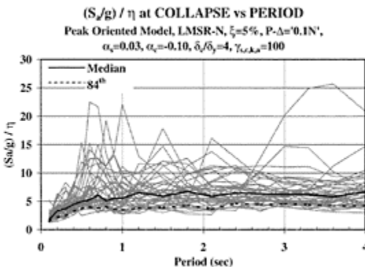
FIGURE 9.26 Variation of collapse capacity with period; base case structural system. (Ibarra, L., Medina, R. and Krawinkler, H. (2002). Collapse assessment of deteriorating SDOF systems. Proc. 12th European Conference on Earthquake Engineering, London, Paper Reference 665. With permission.)
