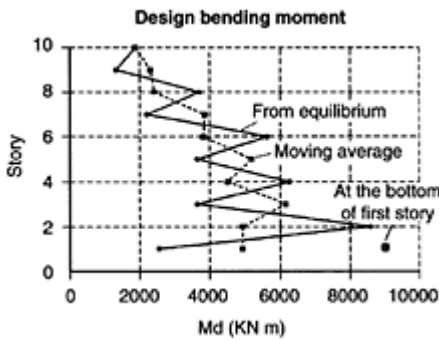
FIGURE 8.32 Design bending moment for interior column.
