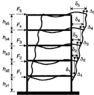
FIGURE 14.16 Story drift computation.
