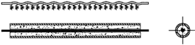
FIGURE 16.23 Core loaded sleeved strut (Kalyanaraman, V., Sridhara, B.N. and Mahadevan, K., (1994). Sleeved column system, Proc. SSRC Task Group Meetings and Task Force Sessions , Lehigh University, Bethlehem, PA.).
