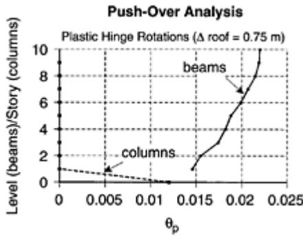
FIGURE 8.47 Plastic hinge rotations for push-over analysis.
