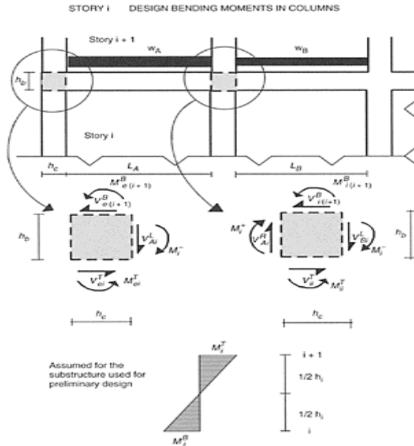
FIGURE 8.11 Design bending moments for columns of a generic story i .
