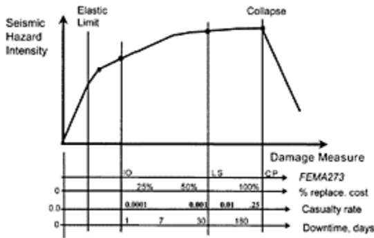
FIGURE 9.7 Conceptual relationship between seismic hazard intensity and structural performance (Courtesy W. Holmes, G.Deierlein).
