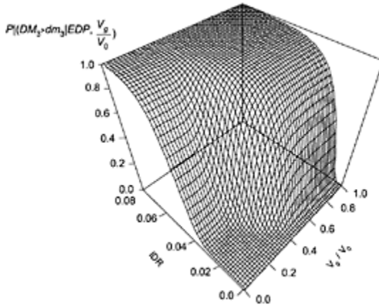
FIGURE 9.35 Probability of experiencing or exceeding a punching shear failure in an interior slab-to-column connection as a function of interstory drift ratio and gravity shear force ratio.
