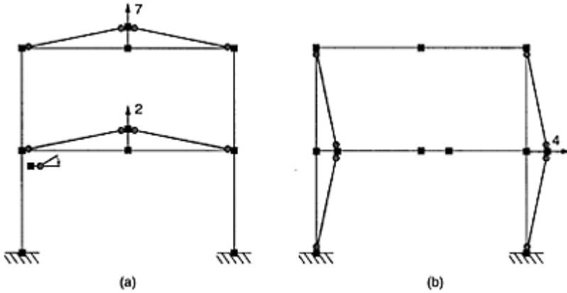
FIGURE 6.12 A few independent collapse mechanisms.
