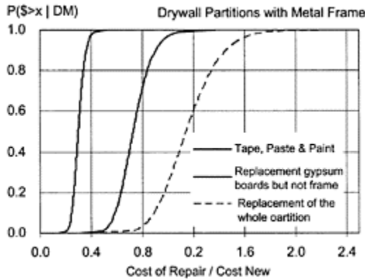
FIGURE 9.43 Loss functions for three damage states in drywall partitions with metal frames.
