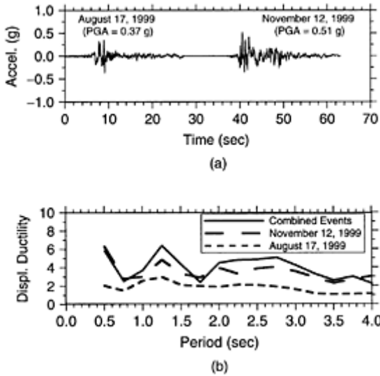
FIGURE 5.16 Ground accelerations (a); and displacement ductility ratio spectra (b); for the Düzce (EW component) recordings of the August 17, 1999 Kocaeli ( M_w=7.4 ) and November 12, 1999 Düzce ( M_w=7.1 ) earthquakes in Turkey.
