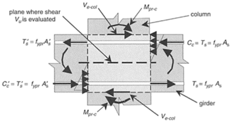
FIGURE 14.35 Joint shear determination.
