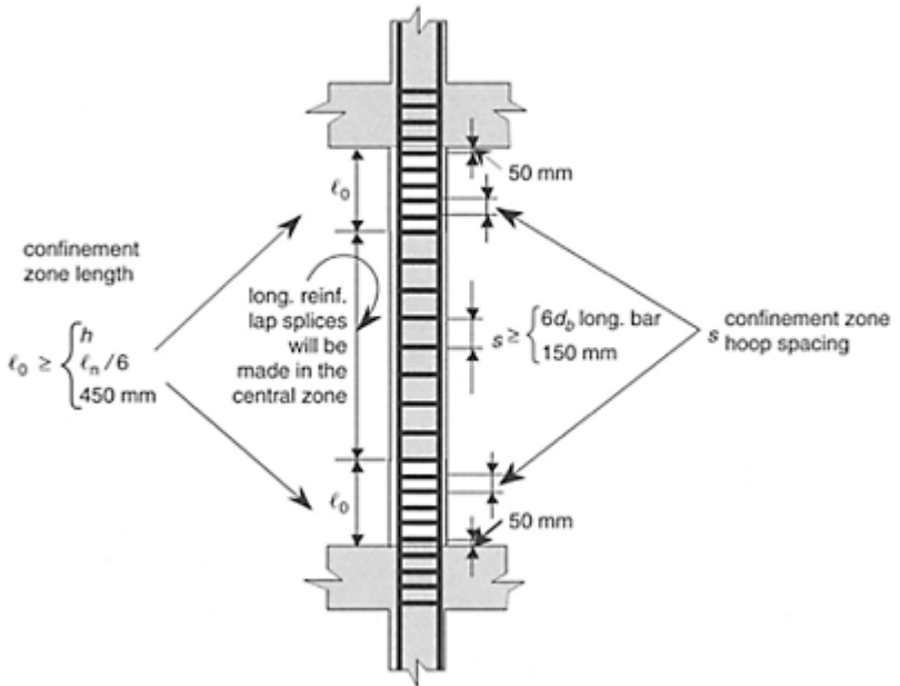
FIGURE 14.31 Confinement hoop spacing in columns.
