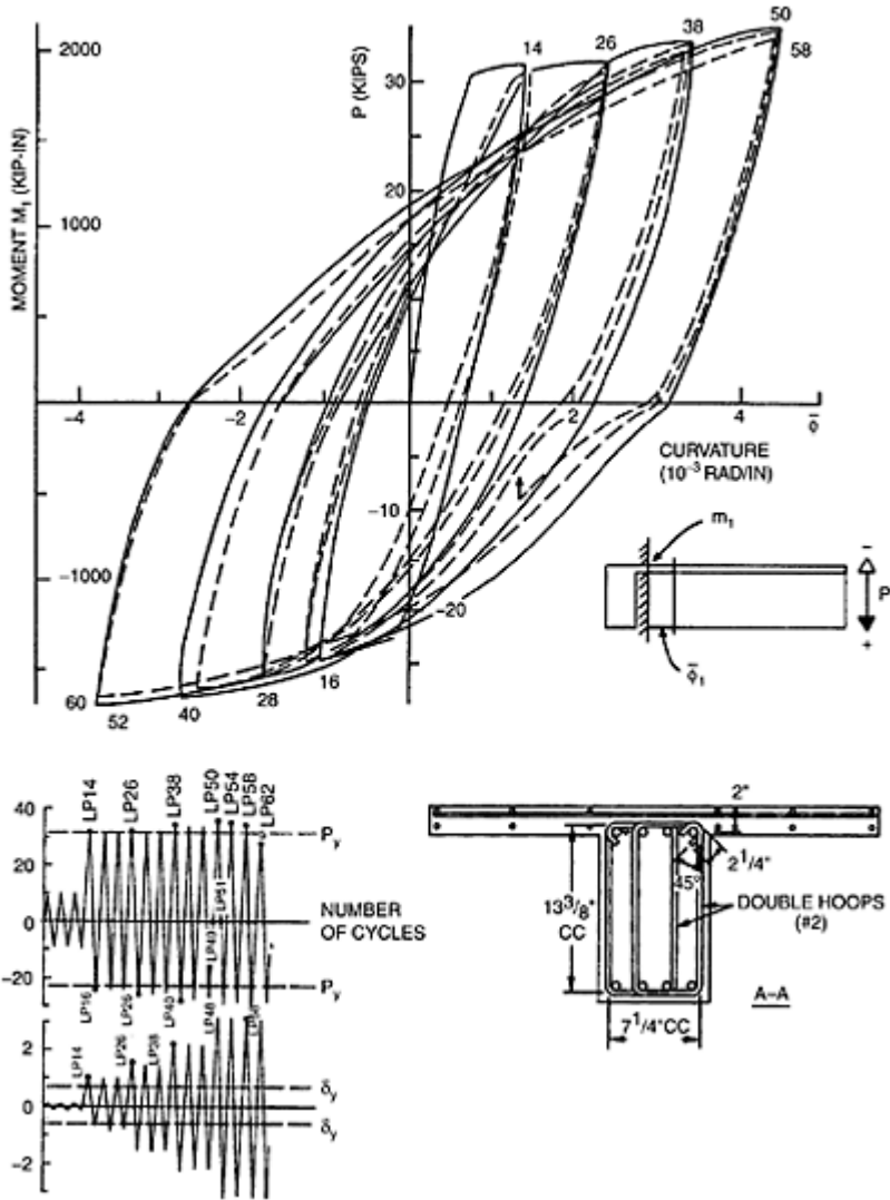
FIGURE 8.64 Test results for a half scale T-beam (Ma et al., 1976).
