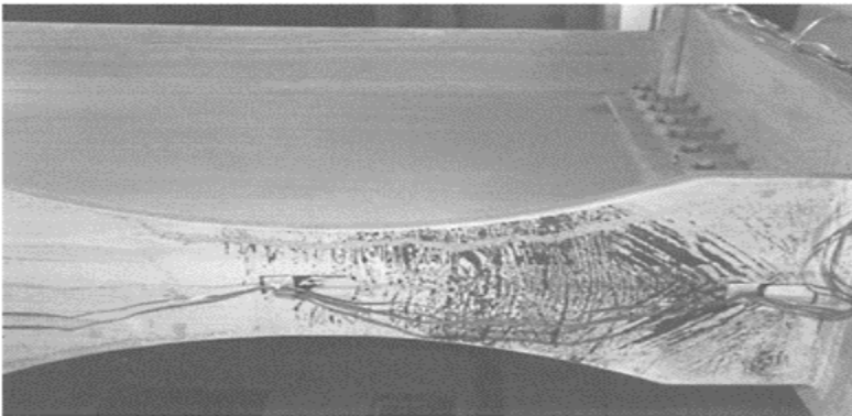
FIGURE 15.13 Moment connection modified with RBS scheme (Yu, Q.-S., Noel, S. and Uang, C.-M.
