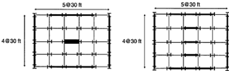
FIGURE 7.11 Plane of five-story one-way dual systems with equal total lateral resistances.
