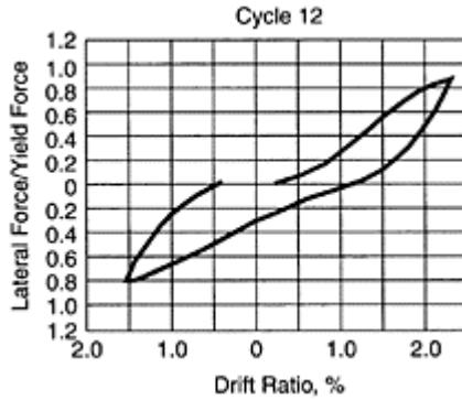
FIGURE 13.19L A force-displacement relationship in a cycle of applied displacement for the test frame in Figure 13.18.
