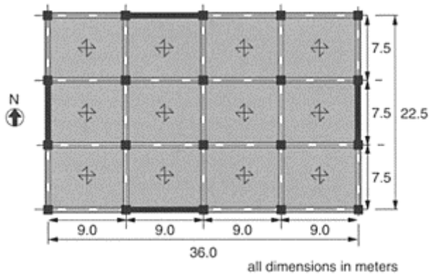
FIGURE 14.46 One-bay wall scheme studied in (Garcia, 1996).
