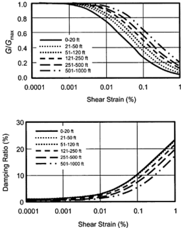
FIGURE 4.6 EPRI model: (a) modulus reduction curves and (b) damping curves.
