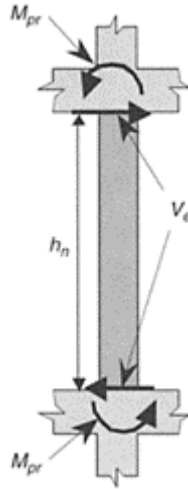
FIGURE 14.33 Calculation of V_e for columns.
