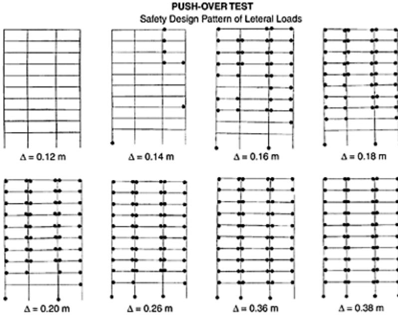
FIGURE 8.43 Sequence of plastic hinge formation for push-over analysis of external frame.
