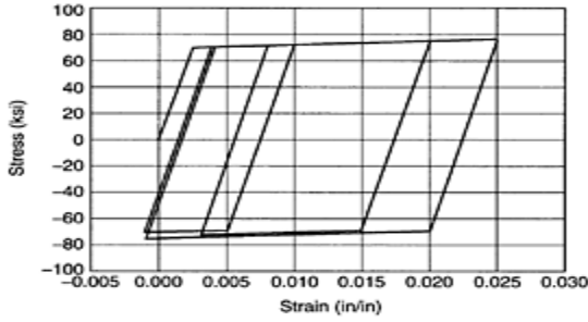
FIGURE 6.15 Hysteretic bilinear stress-strain relationship.
