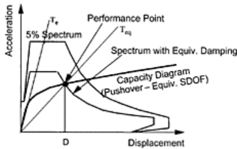
FIGURE 9.6 Illustration of capacity spectrum method.
