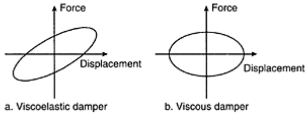
FIGURE 12.2 Force-displacement relations for velocity-dependent dampers.
