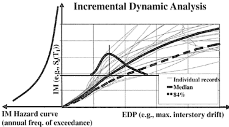
FIGURE 9.19 Incremental dynamic analyses and their use in probabilistic seismic demand analysis.
