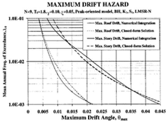
FIGURE 9.20 Examples of hazard curves for engineering demand parameters; nine-story frame structure with T_1=1.8 sec. (Medina, R.A., Ph.D. Dissertation, Stanford University, 2002. With permission.)
