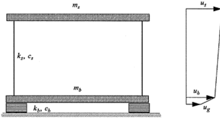
FIGURE 11.6 Parameters of two-degree-of-freedom isolation system model.
