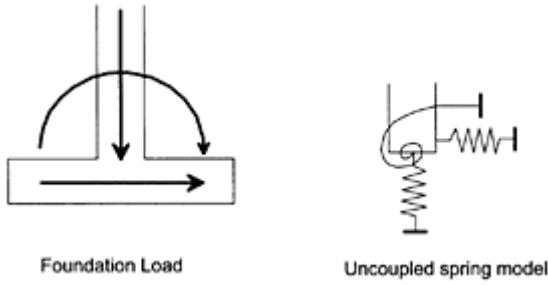
FIGURE 4.17 Uncoupled elastoplastic spring model for rigid footings.
