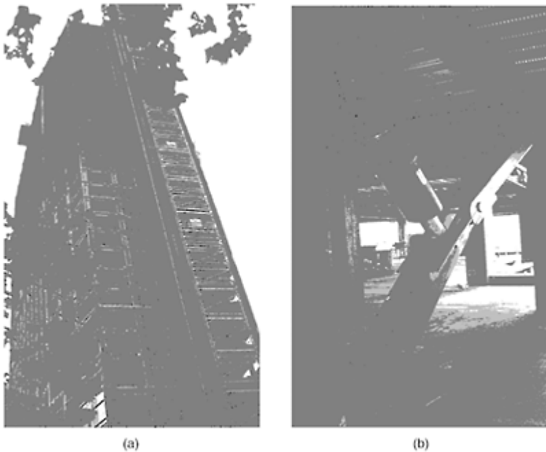
FIGURE 12.16 Toggle-brace assemblies in the Yerba Buena Tower, (a) Elevation of tower; (b) toggle brace assembly.
