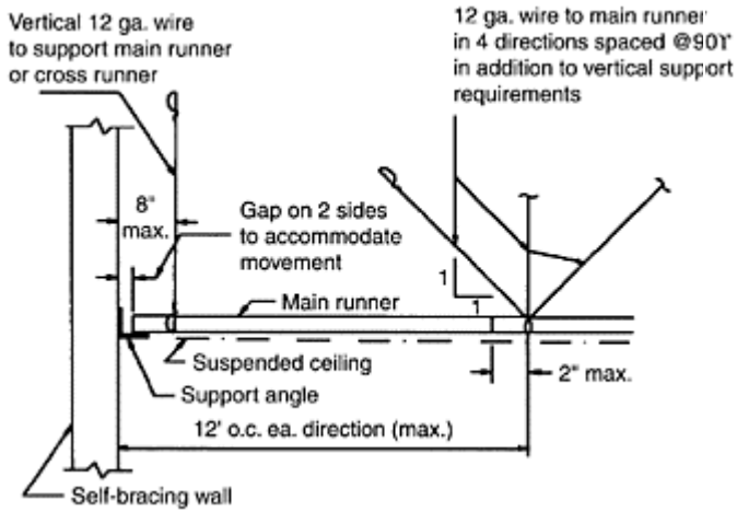
FIGURE 19.24 Bracing detail for suspended ceilings. (Adapted from Sabol, T.A. (1989). Design of nonstructural systems and components, in Seismic Design Handbook , Naeim, F., Ed., Van Nostrand Reinhold, New York, chap. 12. With permission.)
