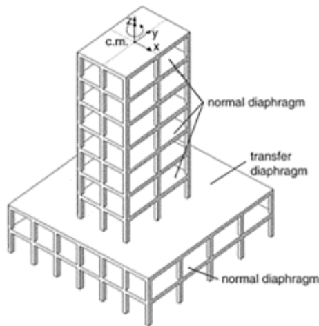
FIGURE 14.26 Example of transfer diaphragm.
