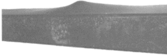
FIGURE 16.13 Bulging of steel casing (courtesy of Star Seismic, LLC).
