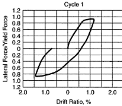
FIGURE 13.19A A force-displacement relationship in a cycle of applied displacement for the test frame in Figure 13.18.
