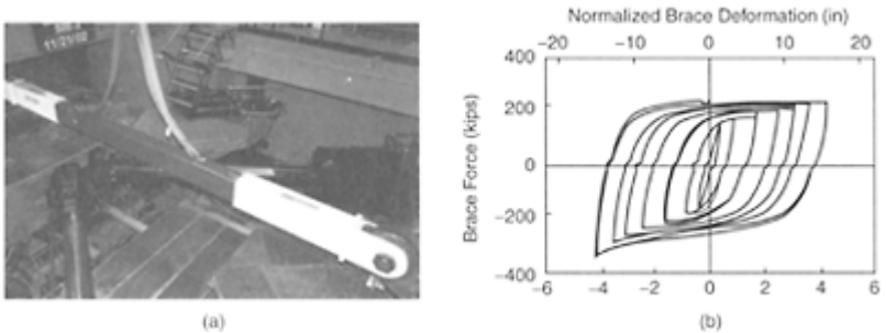
FIGURE 16.47 Test setup and typical response of Star Seismic buckling-restrained braces, (a) Test setup; (b) hysteresis response. (Merritt, S., Uang, C.M. and Benzoni, G. (2003b), Subassemblage testing of Star Seismic buckling-restrained braces, Report
