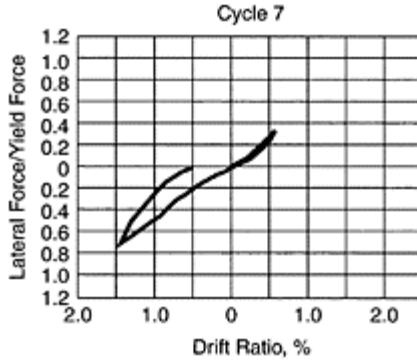
FIGURE 13.19G A force-displacement relationship in a cycle of applied displacement for the test frame in Figure 13.18.
