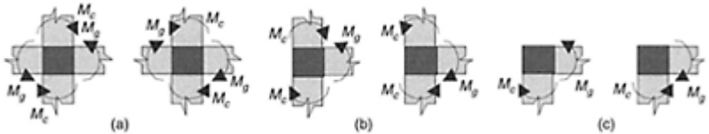
FIGURE 14.30 Minimum flexural strength of columns.
