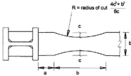
FIGURE 15.8 Reduced beam section dimensions.
