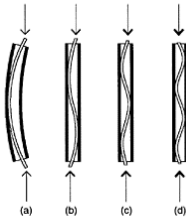
FIGURE 16.21 Concept of sleeved column (Sridhara, B.N. (1990). Sleeved column—as a basic compression member, Proc. 4th International Conference on Steel Structures & Space Frames , Singapore, pp. 181–188.).
