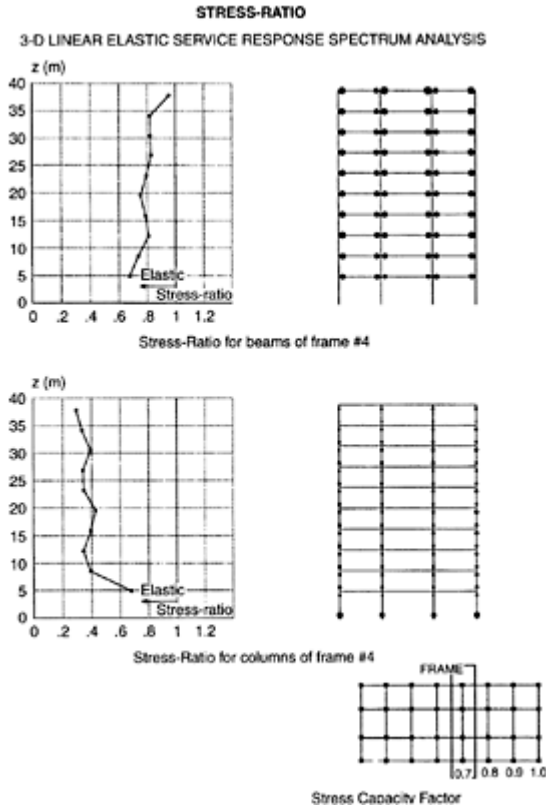
FIGURE 8.41 Stress-ratio for columns and beams.
