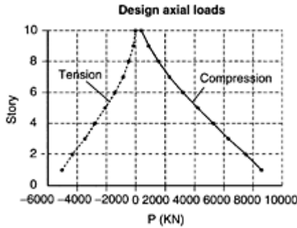
FIGURE 8.29 Design axial load for exterior column.
