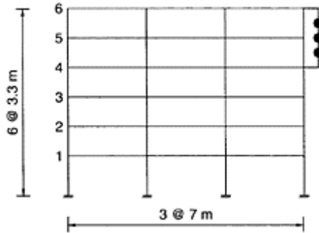
FIGURE 19.16 Building and nonstructural element considered in Example 19.2. (Note 1 m=3.28 ft.)
