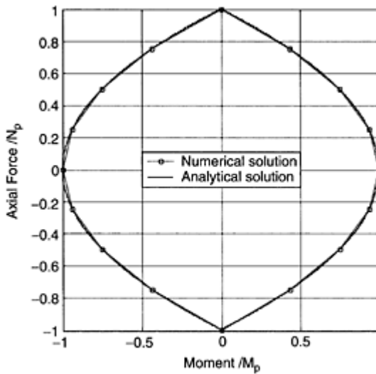
FIGURE 6.21 Axial force-bending moment interaction diagram of rectangular section with elastic-perfectly plastic material; analytical and numerical solution with eight midpoint evaluations.
