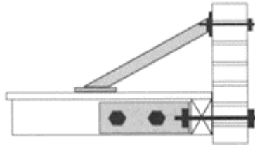
FIGURE 17.18 Schematic of Division 88 masonry retrofitting techniques for unreinforced masonry.
