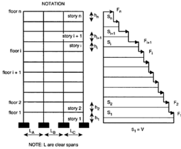
FIGURE 8.8 Generic frame considered for plastic design.
