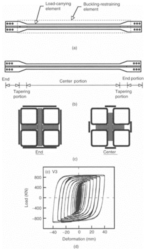
FIGURE 16.32 Steel-only buckling-inhibiting brace, (a) Components; (b) load-carrying core steel; (c) cross sections; (d) hysteresis response. (Chen, C.C., Wang, C.H. and Hwang, T.C. (2001b). Buckling strength of
