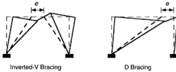
FIGURE 16.5 Yielding mechanism in eccentrically braced frames.
