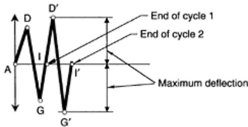
FIGURE 14.2 Vertical deflection program for beam (c) Special in Figure 14.1.
