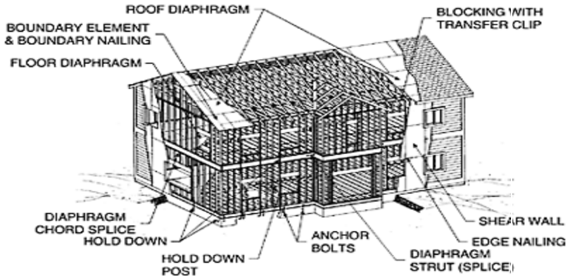
FIGURE 18.1 Typical components of woodframe construction. (From SEAOC, 1997, Guidelines for Wood Diaphragms and Shear Walls . With permission.)
