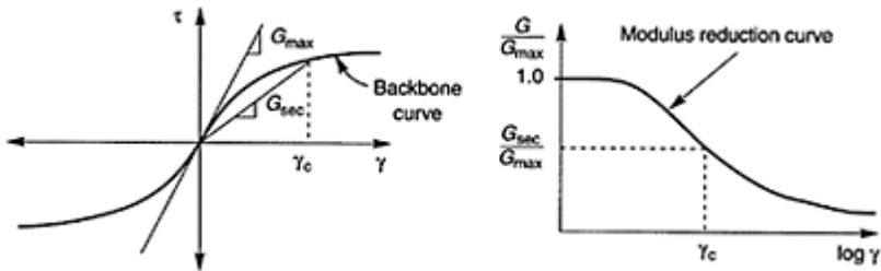
FIGURE 4.4 Relationship between (a) backbone curve and (b) modulus reduction curve.
