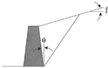
FIGURE 4.47 Schematic illustration of retaining wall.
