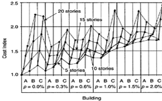
FIGURE 14.42 Cost index (ratio of the cost of the structure for each case to the structure cost for the five-story layout type A building without walls) for the buildings studied in (Garcia and Bonacci, 1996).
