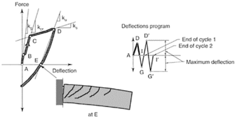
FIGURE 14.4 First one-half cycle for example beam.
