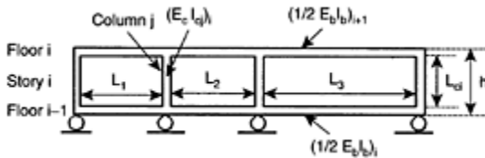
FIGURE 8.6 Substructure to estimate story stiffness for moment resisting frames.
