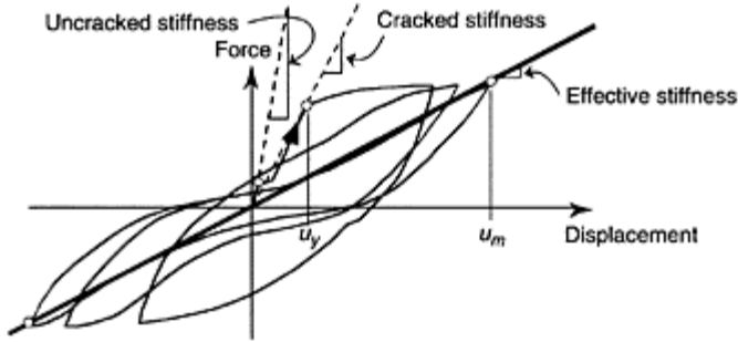
FIGURE 14.23 Stiffness during nonlinear response for a reinforced concrete element.
