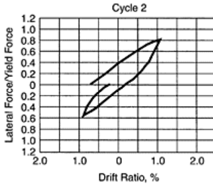
FIGURE 13.19B A force-displacement relationship in a cycle of applied displacement for the test frame in Figure 13.18.
