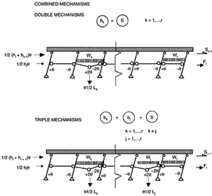
FIGURE 8.10 Combined mechanisms.
