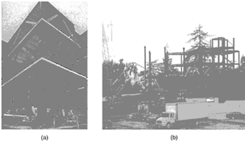
FIGURE 12.6 Unbonded steel brace applications (courtesy of I.Aiken). (a)
