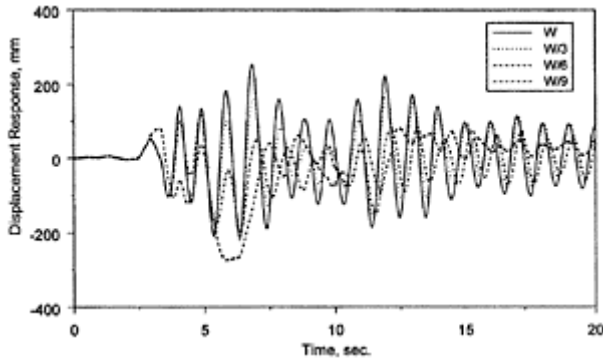
FIGURE 13.16 Calculated displacement responses of oscillators with different strengths to a ground motion with moderate peak velocity (initial period of oscillator=1.0 sec).
