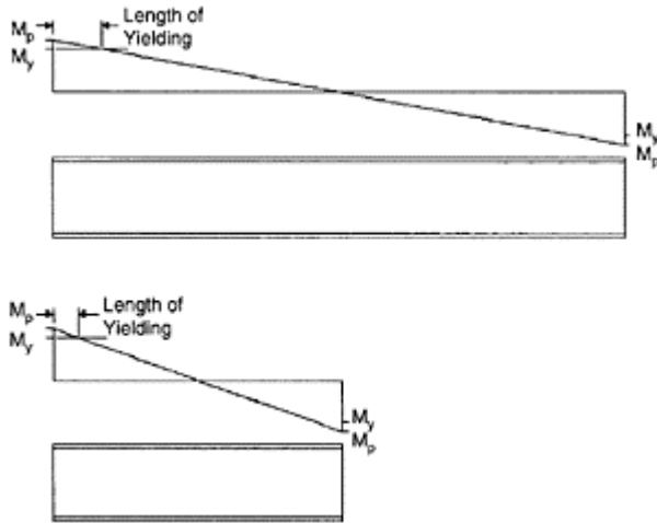
FIGURE 15.4 Span effect on M_p (FEMA 355D).
