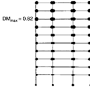
FIGURE 8.61 Damage index obtained from time-history analysis.
