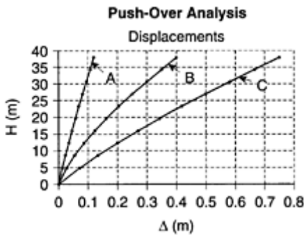
FIGURE 8.45 Displacements for push-over analysis.
