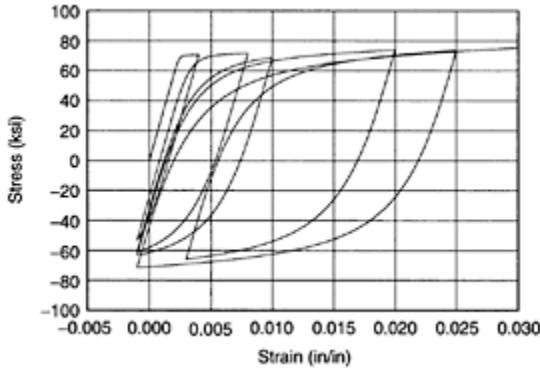
FIGURE 6.16 Hysteretic steel stress-strain relation by Menegotto-Pinto.
