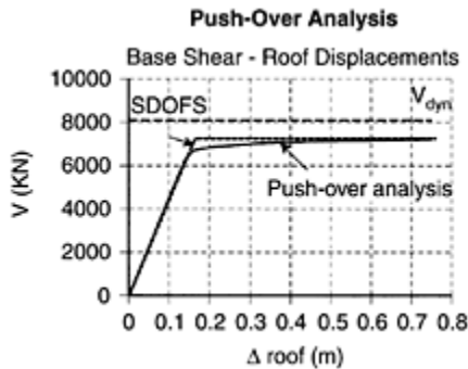
FIGURE 8.49 Dynamic base shear capacity, push-over analysis and equivalent SDOFS.
