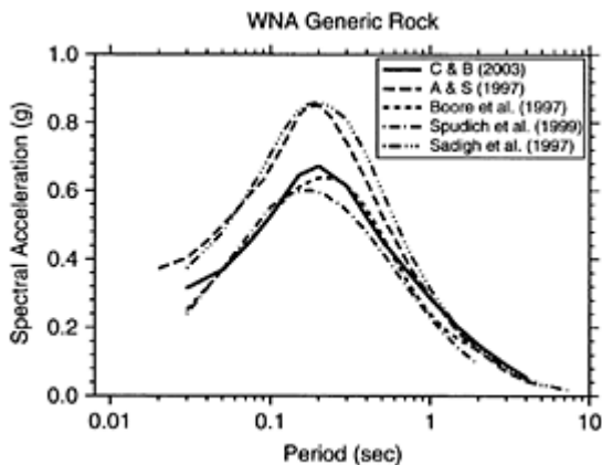
FIGURE 5.26 Comparison of 5%-damped pseudo-acceleration ( S_a ) response spectra predicted by the WNA ground motion relations listed in Table 5.4. The relations are evaluated for M_W=7 , r_{jb}=r_{ru}=10 km, r_{seis}=10.4 km ( d_s=3 km), strike-slip faulting, and generic rock site conditions (see Tables 5.6 and 5.7). PGA is plotted at 0.03-sec period. A & S (1997) refers to Abrahamson and Silva (1997) and C & B (2003) refers to Campbell and Bozorgnia (2003).
