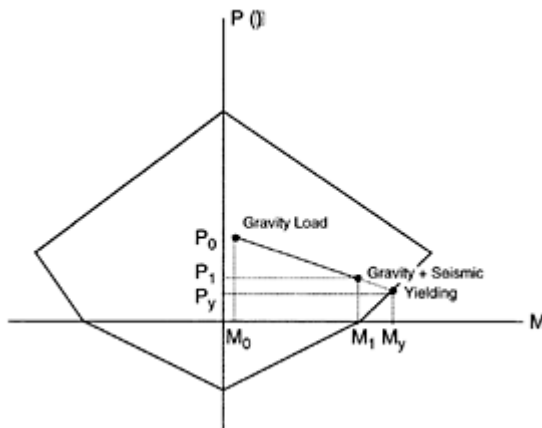
FIGURE 8.40 Determination of stress-ratio for columns.
