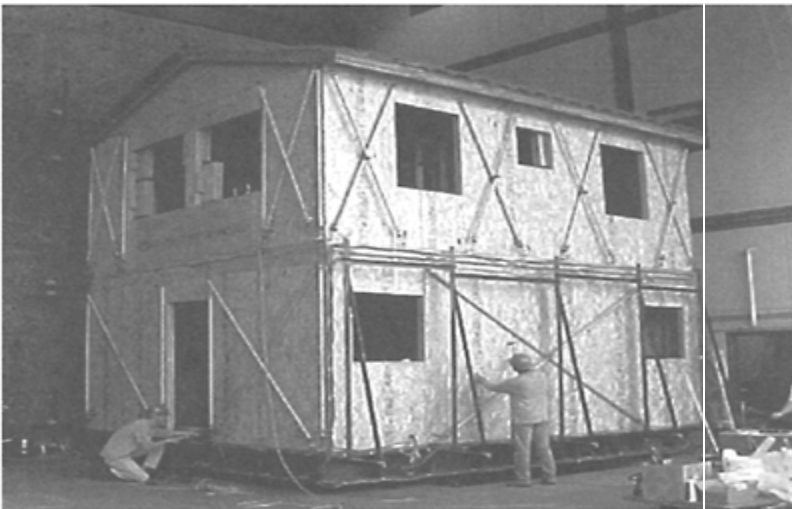
FIGURE 18.15 UC San Diego two-story house, Phase 9, without finishes. (From Fischer et al., 2001, CUREE Publication W-
