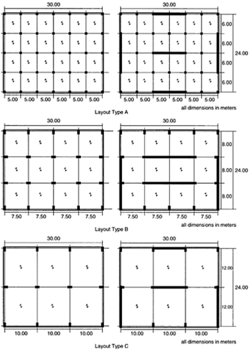
FIGURE 14.41 Plan layout types in buildings studied in (Garcia and Bonacci, 1996).
