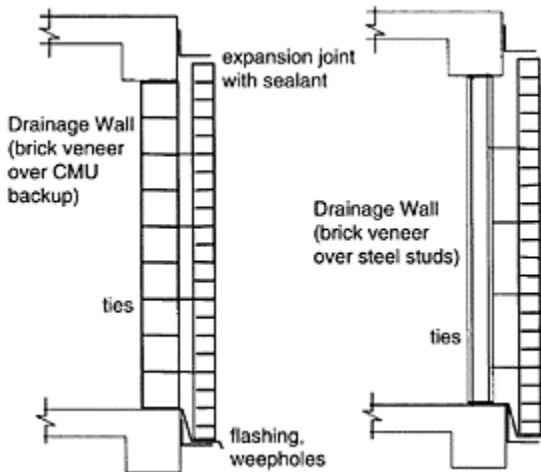
FIGURE 17.2 Examples of drainage walls.
