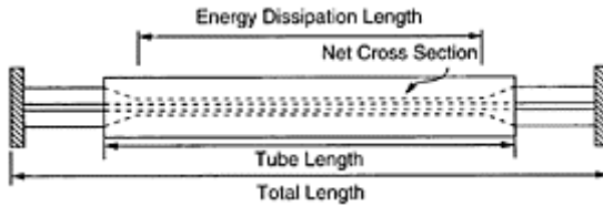
FIGURE 16.33 Geometry of buckling-restrained brace test specimens. (Tsai, K.C. and Lai, J.W. (2002). A study of buckling restrained seismic braced frame, Structural Engineering , 17(2), (in Chinese).)
