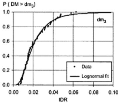
FIGURE 9.33 Fragility function for damage measure dm_3 in interior reinforced concrete slab-column connections of flat plates.
