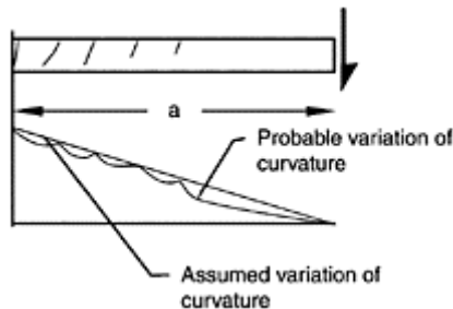
FIGURE 13.22 Distribution of curvature
