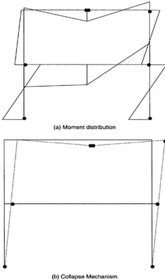
FIGURE 6.13 Moment distribution and mechanism at incipient collapse.
