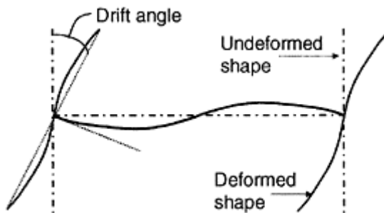
FIGURE 15.7 Interstory drift angle (FEMA 350).
