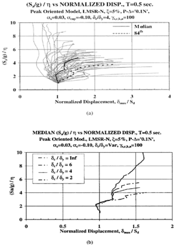
FIGURE 9.25 (S_a/g)/\eta -EDP graphs, (a) for a specific system and individual records, (b) median results for four different systems. (Ibarra L. et al., Proc. 12th European Conference on
