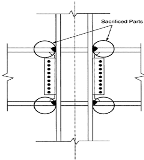
FIGURE 10.4 Typical beam-column connection in the United States before Northridge earthquake.
