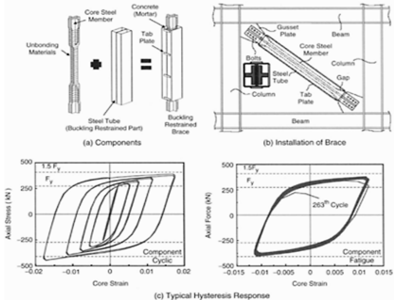
FIGURE 16.35 Double-tube budding-restrained brace. (Tsai, K.C. and Lai, J.W. (2002). A study of buckling restrained seismic braced frame, Structural Engineering , 17(2), (in Chinese).)
