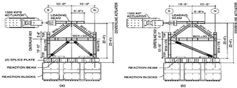
FIGURE 16.44 Subassembly test setup,
