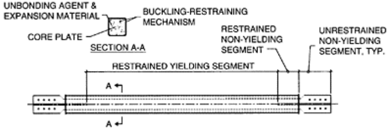
FIGURE 16.11 Components of budding-restrained brace. (Adapted from Wada et al. (1998) by López 2001.)
