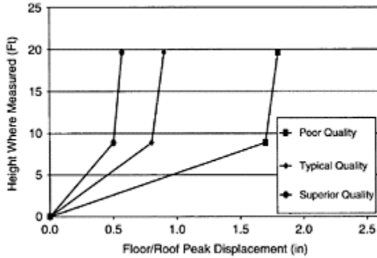
FIGURE 18.22 Vertical distribution of deformation demand in Large House Index Building considering three levels of construction quality. (From Cobeen et al., 2003, CUREE Publication W-30, CUREE, Richmond, CA. With permission.)
