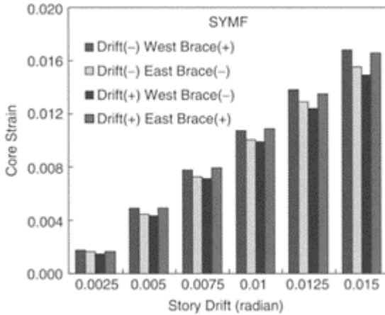
FIGURE 16.43 Axial strains in tension and compression braces (Tsai, K.C., Hwang, Y.C. and Weng, C.S. (2004). Subassembly testing and analysis of buckling restrained brace for seismic resistance, Structural Engineering , 18 (in Chinese).)
