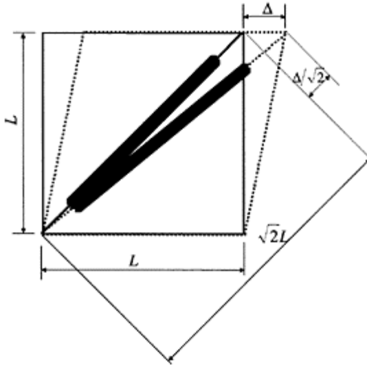
FIGURE 10.6 Axial deformations of brace and shear deformation of frame.
