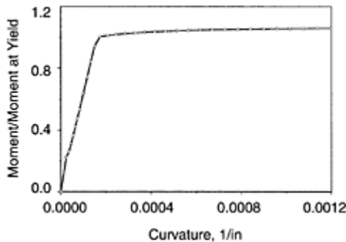
FIGURE 13.7 Calculated relationship between bending moment and unit curvature.
