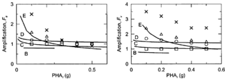
FIGURE 4.11 Spectral amplification factors as a function of NEHRP Categories B-E, as evaluated by Stewart et al. (2003c) (lines). NEHRP factors from Figure 4.8 are shown for comparison (symbols).
