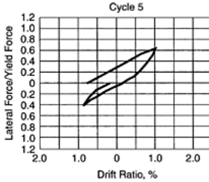
FIGURE 13.19E A force-displacement relationship in a cycle of applied displacement for the test frame in Figure 13.18.
