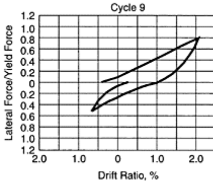
FIGURE 13.19I A force-displacement relationship in a cycle of applied displacement for the test frame in Figure 13.18.
