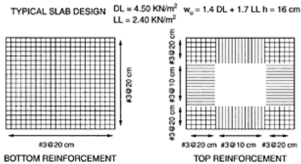
FIGURE 8.17 Design of a typical building slab.
