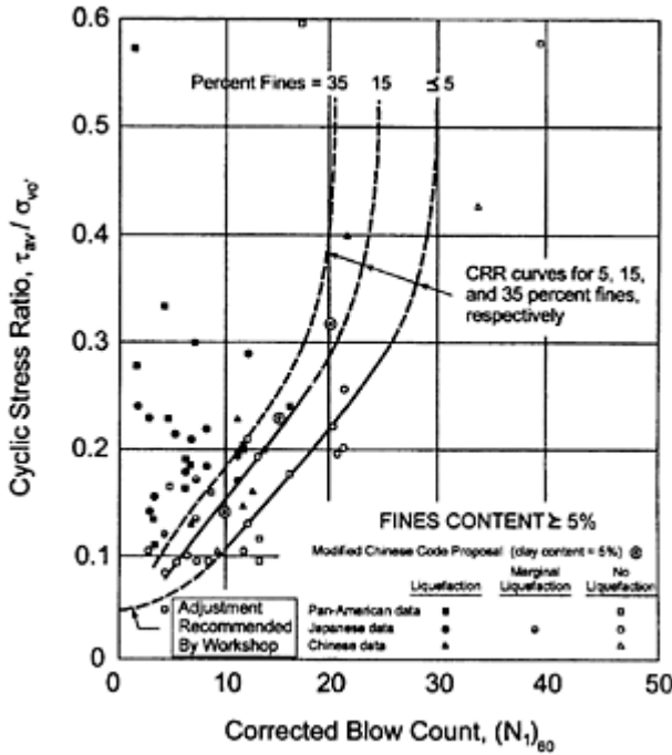
FIGURE 4.29 Variation of CRR with corrected standard penetration resistance, (N_1)_{60} . (From Youd, T.L. et al., J. Geotech. Geoenviron. Eng. , ASCE, 127, 817–833, 2001. With permission.)
