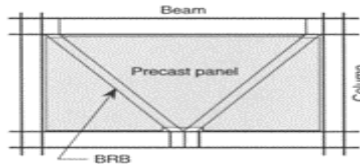
FIGURE 16.14 Buckling restrained braces sandwiched between precast concrete panels.
