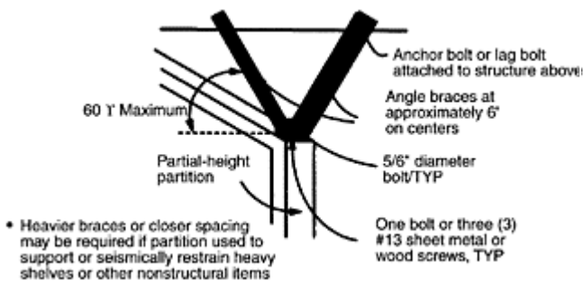
FIGURE 19.22 Seismic bracing of partial lightweight partitions. (From Federal Emergency Management Agency,
