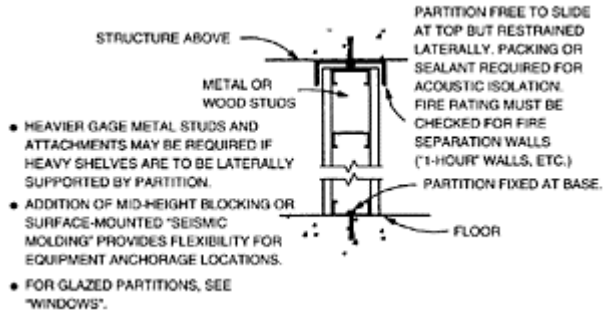
FIGURE 19.21 Seismic bracing of full lightweight partitions. (From Federal Emergency Management Agency, Reducing the Risks of Nonstructural Earthquake Damage, A Practical Guide, FEMA, Washington, D.C., 1994.)
