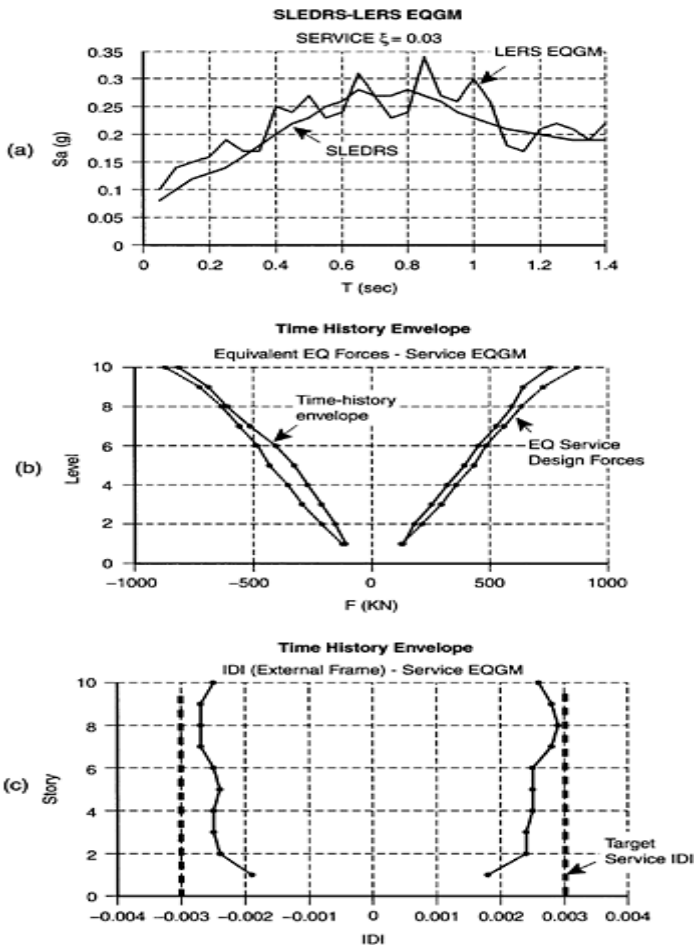
FIGURE 8.42 (a) SLEDRS and LERS of the factored service EQGM used for time-history analysis, (b) Design and
