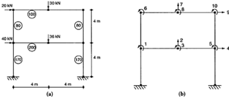
FIGURE 6.10 (a) Two-story frame, (b) Free global DOFs without axial deformations.
