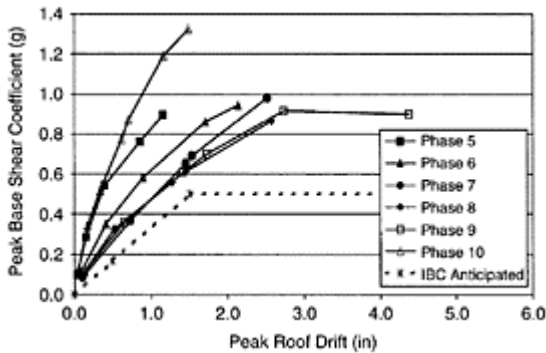
FIGURE 18.19 Load-deflection behavior for UC San Diego house. Phase 9 is final configuration without finish materials. Phase 10 is final configuration with finish materials. No failures were observed. Curves end at stop of testing. (From Cobeen et al., 2003, CUREE Publication W-30, CUREE, Richmond, CA. With permission.)
