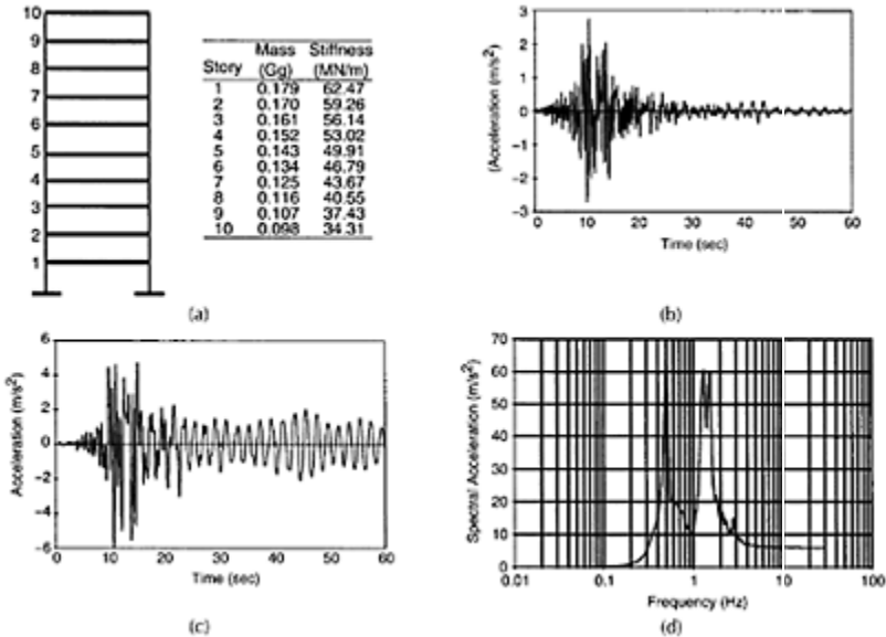
FIGURE 19.9 (a) Ten-story building considered in Example 19.1. (Note: Gg=68 , 525 slugs; 1\text{ MN/m}=737.5\text{ kips/ft} ); (b) E-W component of ground acceleration recorded at the Foster City station during the 1989
