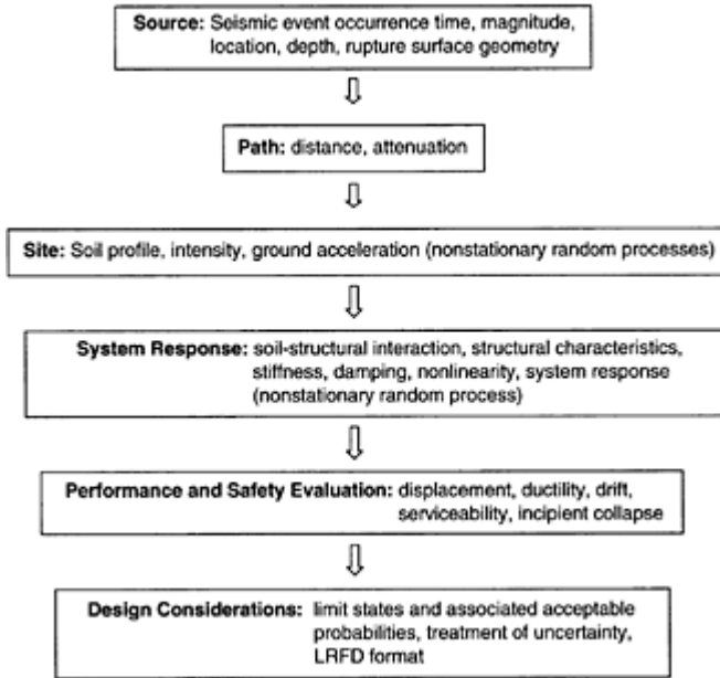
FIGURE 7.1 Probabilistic performance evaluation and design for earthquakes.
