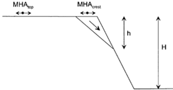
FIGURE 4.40 Schematic illustration of slope geometry considered by Ashford and Sitar (2002) for steep slopes of weakly cemented rock/soil.
