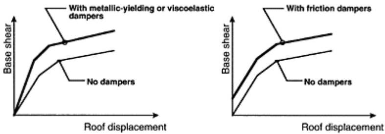
FIGURE 12.3 Influence of dampers on building response.
