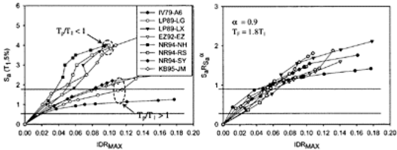
FIGURE 9.18 IDAs with two different intensity measures; (a) IM=S_a(T_1) , (b) IM=S_a R_{sa}^\alpha . (Cordova, P.P., et al., Proc. 2nd U.S.-Japan Workshop on Performance-Based Earthquake Engineering for Reinforced Concrete Building Structures , 2000. With permission.)
