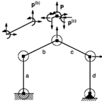
FIGURE 6.3 Node and element free body equilibrium.
