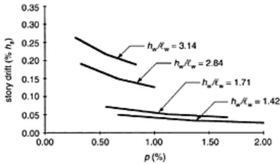
FIGURE 14.48 Story drift as a percentage of story height obtained for different values of the wall area ratio, p , for eight-story building having the plan layouts shown in Figures 14.46 and 14.47 and located in a moderate seismic zone studied in (Garcia, 1996).
