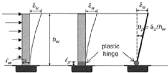
FIGURE 14.38 Wall responding in the nonlinear range.
