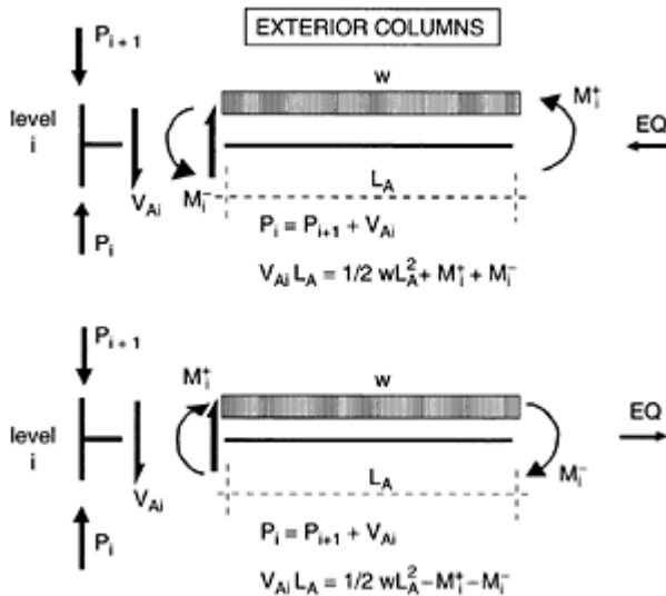
FIGURE 8.12 Equilibrium equations for determining axial forces in external columns.
