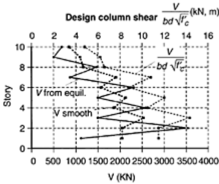
FIGURE 8.35 Shear and normalized shear stress for interior columns.
