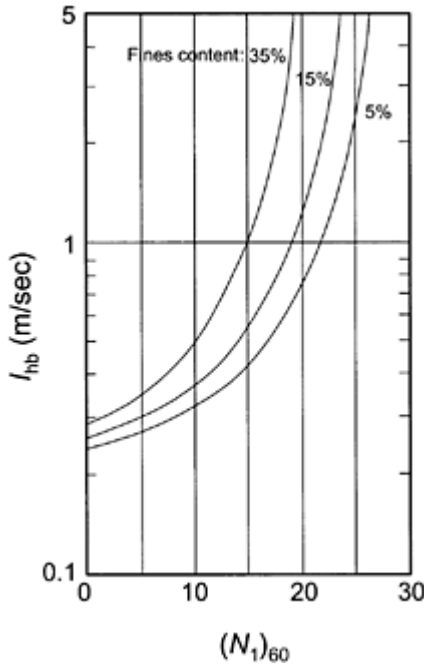
FIGURE 4.31 Variation of Arias intensity required to trigger liquefaction with corrected standard penetration resistance, (N_1) (Modified from Kayen, R.E. and Mitchell, J.K., J. Geotech. Geoenviron. Eng. , ASCE, 123, 1162–1174, 1997. With permission.)
