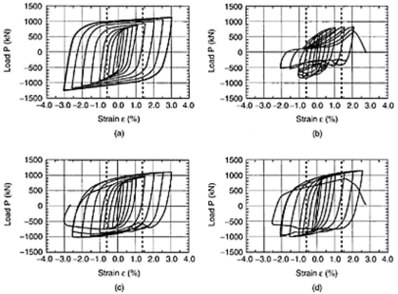
FIGURE 16.20 Cyclic response of four test specimens. (a) Type 1; (b) type 2; (c) type 3; (d) type 4. (Iwata, M., Kato, T. and Wada, A. (2000).
