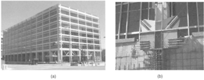
FIGURE 16.9 Buckling-restrained brace frames for seismic rehabilitation of reinforced concrete building, (a) Global view (courtesy of SIE, Inc.); (b) connection details (courtesy of Reaveley Engineers & Associates, Inc.).
