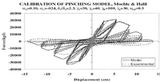
FIGURE 9.23 Comparison between experimental results and analytical predictions for a deteriorating system.
