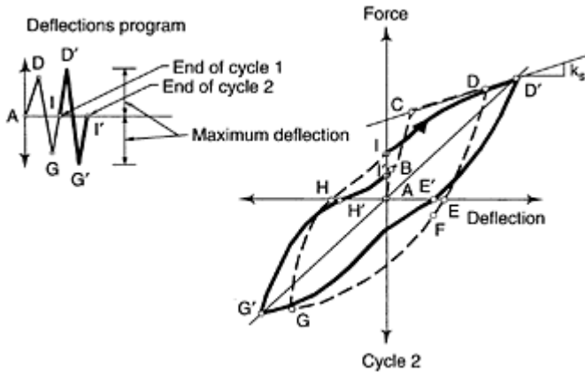
FIGURE 14.6 Second cycle for example beam.
