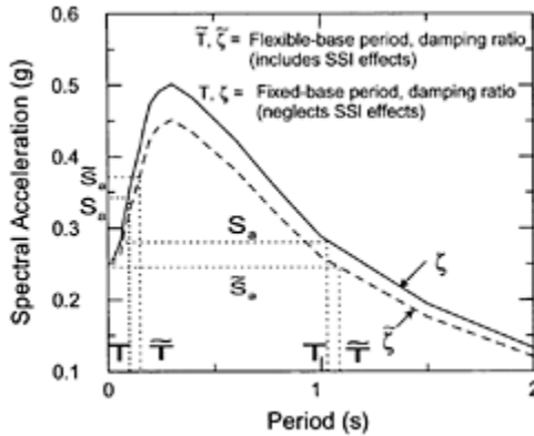
FIGURE 4.20 Schematic showing effects of period lengthening and foundation damping on design spectral accelerations for realistic spectral shape. (From Stewart, J.P. et al.,
