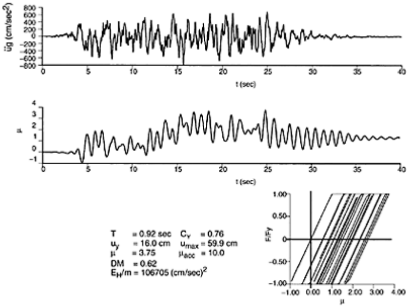
FIGURE 8.48 Equivalent SDOFS response for critical EQGM.
