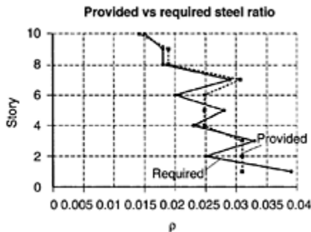
FIGURE 8.34 Provided and required steel ratio for interior column.
