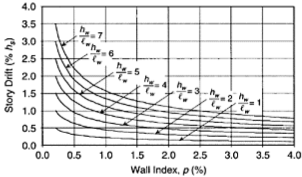
FIGURE 14.22 Relationship between wall index p and story drift index for a spectral acceleration S_{DI} of 100% of g .
