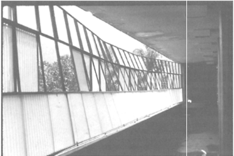
FIGURE 19.4 Failure of window frame in school building during the 1973 Orizaba, Mexico, earthquake.
