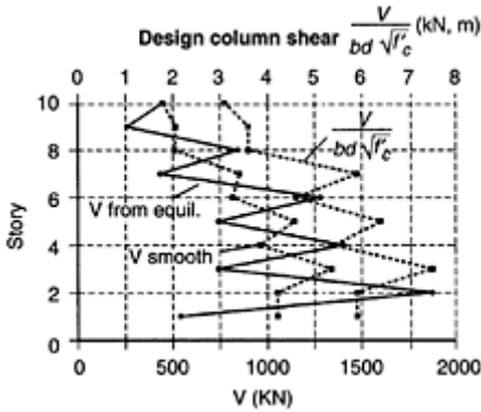
FIGURE 8.31 Shear and normalized shear stress for exterior columns.
