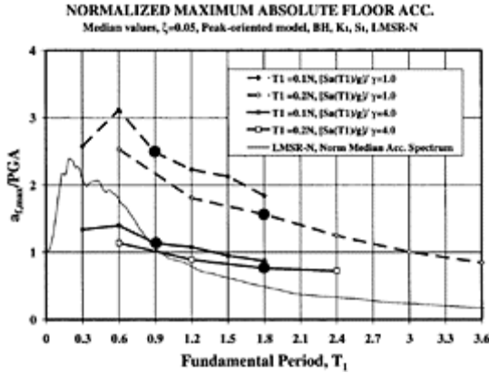
FIGURE 9.49 Median values of normalized maximum floor acceleration for frame structures with T_1=0.1N and T_1=0.2N . (Medina, R.A., Ph.D. Dissertation, Stanford University, 2002. With permission.)
