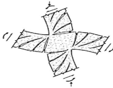
FIGURE 13.21 Deformation of frame joint.
