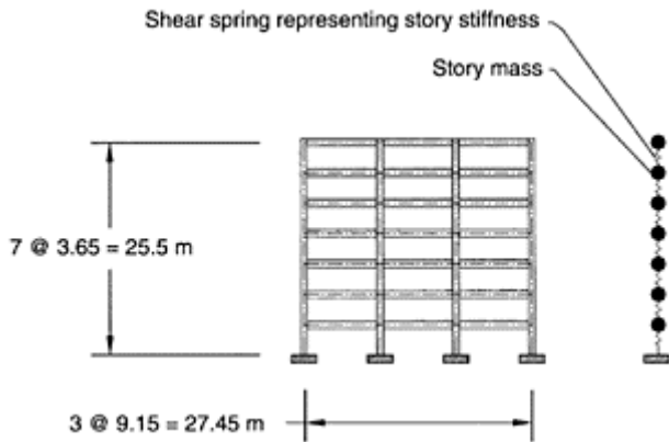
FIGURE 13.2 Seven-story frame and its “shear beam” representation.
