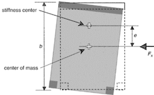
FIGURE 14.11 Torsional moment, M_b , from location of story mass and stiffness.
