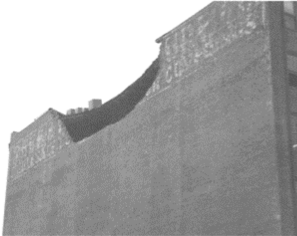
FIGURE 17.12 Partial collapse of an unreinforced masonry bearing wall near Pioneer Square in Seattle. (Photo by The Masonry Society.)
