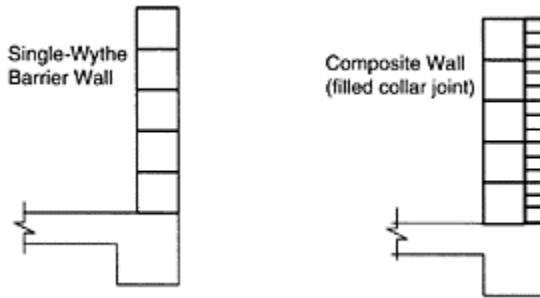
FIGURE 17.1 Examples of barrier walls.
