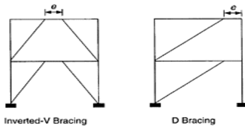
FIGURE 16.4 Examples of eccentric bracing configurations.
