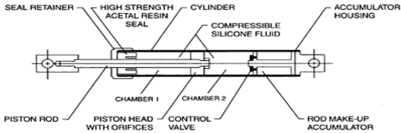
FIGURE 12.9 Schematic section through a fluid viscous damper (courtesy of Taylor Devices).
