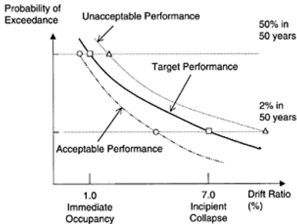
FIGURE 7.8 Bi-level acceptance criteria in terms of 50-year limit state probability in log scale.
