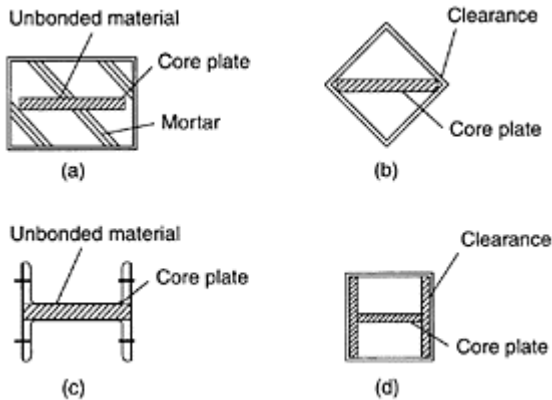
FIGURE 16.19 Section of four test specimens, (a) Type 1; (b) type 2; (c) type 3; (d) type 4. (Iwata, M., Kato, T. and Wada, A. (2000). Buckling-restrained braces as hysteretic dampers, Proc. STESSA , Quebec, PQ, pp. 33–38).
