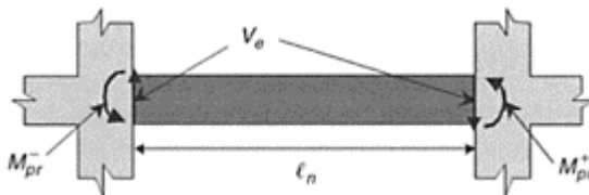
FIGURE 14.29 Calculation of V_e .
