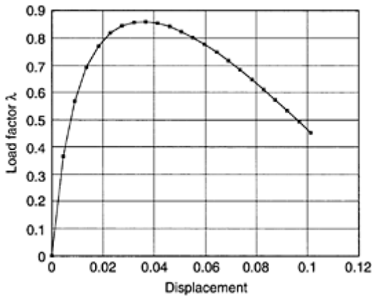
FIGURE 6.20 Load-displacement response with load factor control during iteration.
