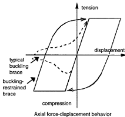
FIGURE 16.7 Behavior of conventional brace versus buckling-restrained brace. (Adapted from Clark, P., et al. (1999). Proc. 69th Annual SEAOC Convention , Sacramento, CA. With permission.)
