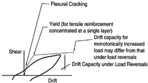
FIGURE 13.20 Drift capacity.
