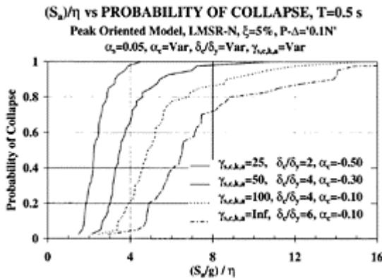
FIGURE 9.30 Collapse fragility curves for systems with various deterioration properties; T=0.5 sec. (Ibarra, L., Medina, R. and Krawinkler, H. (2002). Collapse assessment of deteriorating SDOF systems. Proc. 12th European Conference on Earthquake Engineering , London, Paper Reference 665. With permission.)
