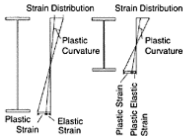
FIGURE 15.3 Elastic and plastic strain distribution (FEMA 355D).
