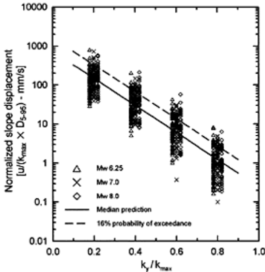
FIGURE 4.46 Normalized sliding displacement (Modified from Bray, J.D. and Rathje, E.M. (1998). J.
