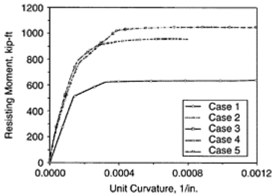
FIGURE 13.12 Calculated moment-curvature relationships.
