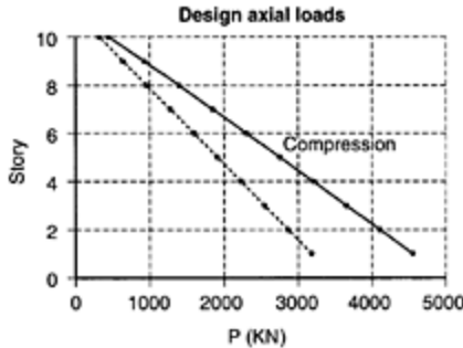
FIGURE 8.33 Design axial load for interior column.
