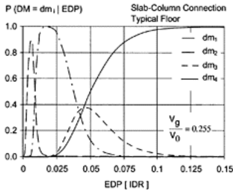
FIGURE 9.37 Probabilities of being in various damage states for an interior slab-to-column connection.
