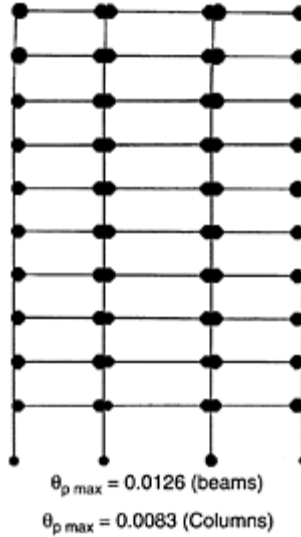
FIGURE 8.55 Time-history analysis: maximum plastic hinge rotations.
