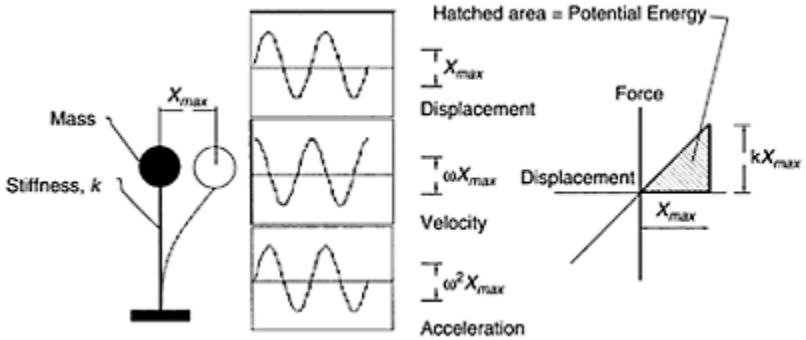
FIGURE 13.1 Response of an SDOF oscillator in harmonic motion.
