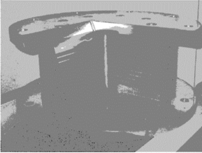
FIGURE 11.8 Cut-away model of a lead-plug isolation bearing (courtesy of DIS, Inc.).
