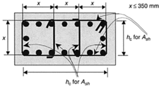
FIGURE 14.32 Separation between legs of hoop and crossties.
