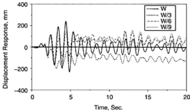
FIGURE 13.15 Calculated displacement responses of oscillators with different strengths to a ground motion with high peak velocity (initial period of oscillator=1.0 sec).
