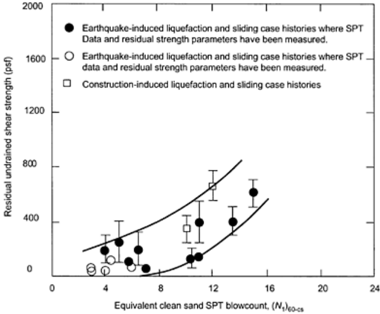
FIGURE 4.35 Estimation of residual strength of liquefied soil from SPT resistance. (From Seed, R.B. and Harder, L.F., Proceedings, H. Bolton Seed Memorial Symposium, Vol. 2 , 351–376, 1990. With permission.)
