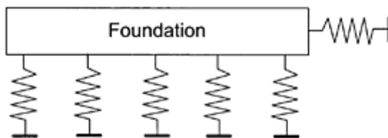
FIGURE 4.16 Uncoupled Winkler spring model.
