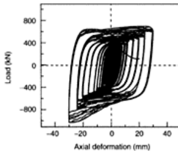
FIGURE 16.31 Typical response of buckling-inhibiting brace (Chen, C.C., Chen, S.Y. and Liaw, J.J. (2001a).
