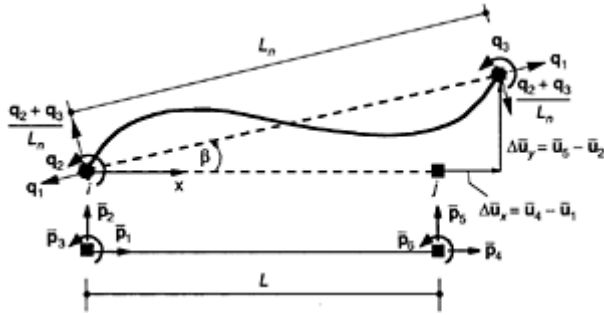
FIGURE 6.9 Equilibrium of frame element in deformed configuration.
