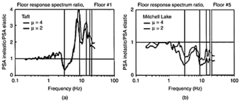
FIGURE 19.12 Floor response spectrum ratios (inelastic structure/elastic structure) corresponding to floor accelerations of five-story shear building with first-floor interstory ductilities of 2 and 4: (a) ratios for first floor when building is subjected to 1952 Taft acceleration record; (b) ratios for fifth floor when building is subjected to 1982 Mitchell Lake acceleration record. Vertical lines identify the natural frequencies of the structure. (Adapted from Sewell, R. T., Damage Effectiveness of Earthquake Ground Motion: Characterizations Based on the Performance of Structures and
