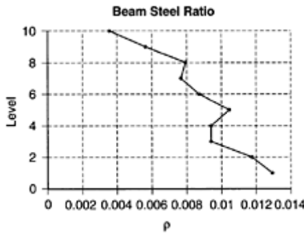
FIGURE 8.25 Provided beam steel ratio.
