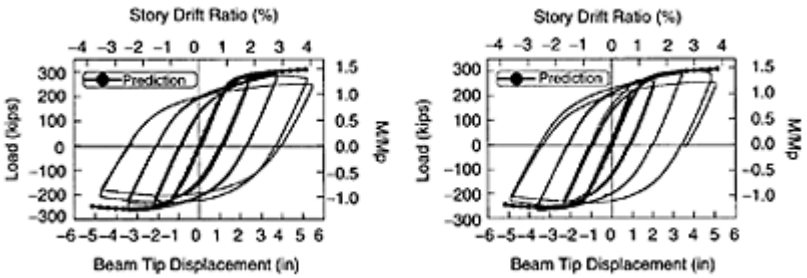
FIGURE 15.16 Load versus beam tip deflection relationships of the composite specimen (Yu, Q.-S., Noel, S. and Uang, C.-M. (1997).
