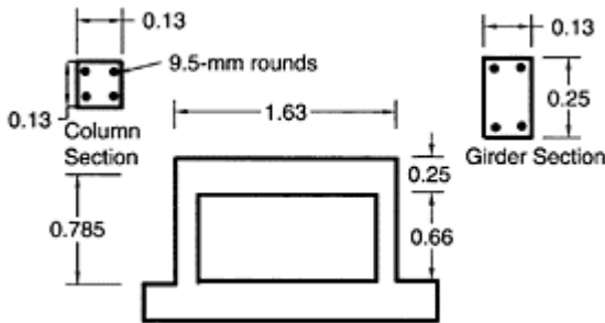
FIGURE 13.18 Test frame.
