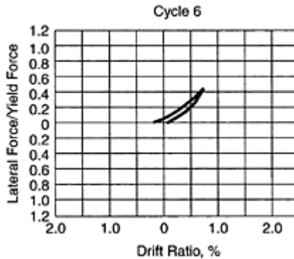
FIGURE 13.19F A force-displacement relationship in a cycle of applied displacement for the test frame in Figure 13.18.
