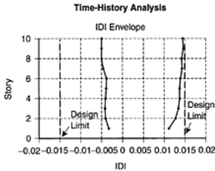
FIGURE 8.52 IDI envelopes for time-history analysis.
