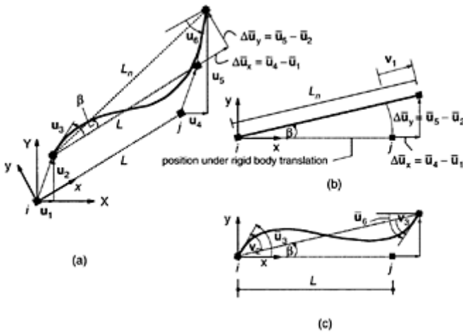
FIGURE 6.7 Deformed configuration of two-node one-dimensional element under large displacements.
