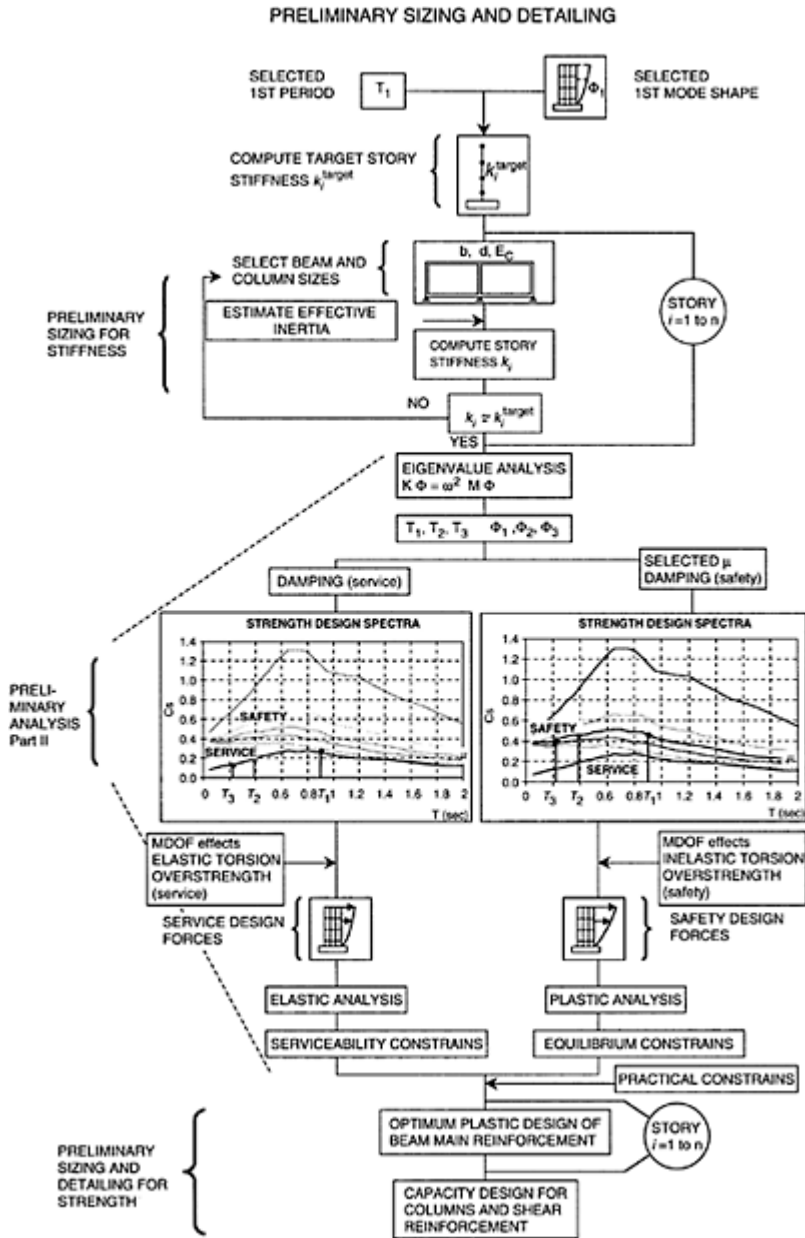
FIGURE 8.4 Flowchart of preliminary sizing and detailing.
