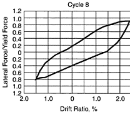
FIGURE 13.19H A force-displacement relationship in a cycle of applied displacement for the test frame in Figure 13.18.
