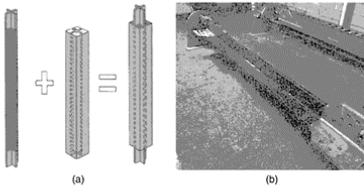
FIGURE 12.5 Unbonded steel brace (courtesy of Nippon Steel), (a) Conceptual details; (b) cruciform configuration of steel
