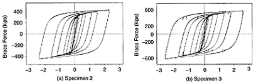
FIGURE 16.24 Cyclic response of Unbonded Braces, (a) Specimen 2; (b) specimen 3. (Clark, P., Aiken, I., Kasai, K., Ko, E. and Kimura, I. (1999). Design procedures for buildings incorporating hysteretic damping devices, Proc. 69th Annual Convention of SEAOC , Sacramento, CA.)
