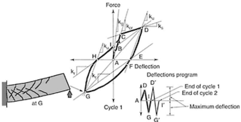
FIGURE 14.5 First cycle for example beam.
