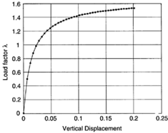
FIGURE 6.19 Load-displacement response with load factor control during incrementation.
