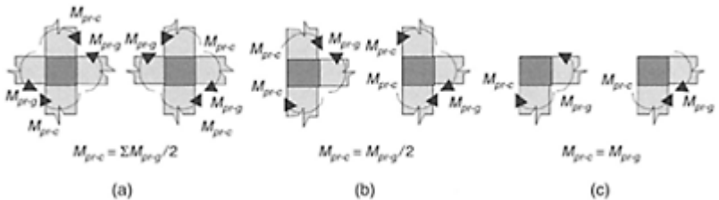
FIGURE 14.34 Maximum M_{pr} for the columns needed to obtain column shear V_e .
