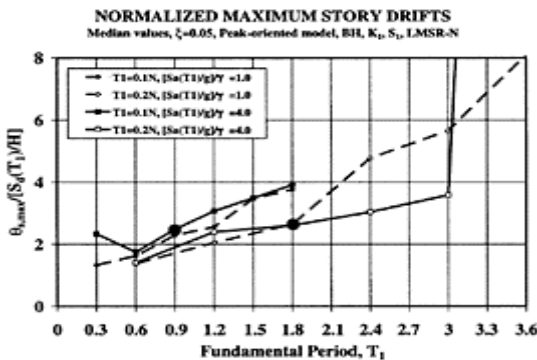
FIGURE 9.48 Median values of normalized maximum story drift for frame structures with T_1=0.1N and T_1=
