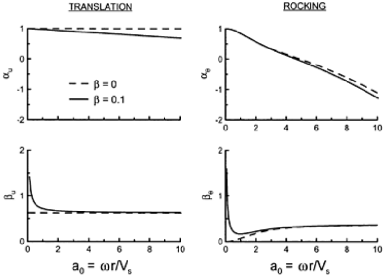
FIGURE 4.21 Foundation stiffness and damping factors for elastic and viscoelastic halfspaces ( \nu=0.4 ). (Adapted from Veletsos, A.S. and Verbic, B., J. Earthquake Eng. Struct. Dyn. , 2, 87–102, 1973.)
