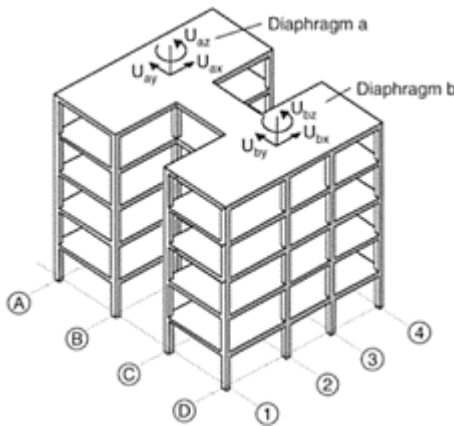
FIGURE 14.25 Independent rigid diaphragms linked by flexible elements.
