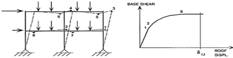
FIGURE 9.8 Illustration of a pushover analysis. (Seneviratna, G.D.R.K. and Krawinkler, H. (1997). Evaluation of inelastic MDOF effects for seismic design. John A.Blume Earthquake Engineering Center Report No. 120, Department of Civil Engineering, Stanford University.)
