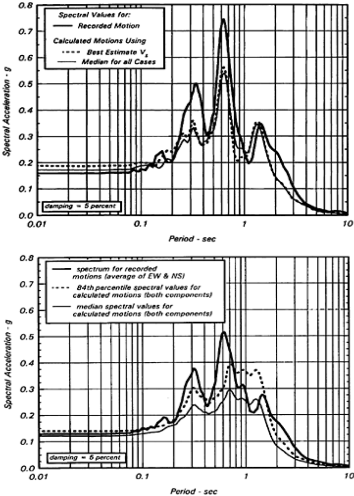
FIGURE 4.12 Comparison of acceleration response spectrum of recorded motion at Treasure Island strong motion site (1989 Loma Prieta earthquake) with calculated spectra from ground response analyses. Calculations in upper frame utilized nearby rock recording (Yerba Buena Island) as control motion; lower frame presents statistical variation in
