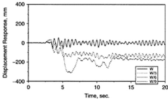
FIGURE 13.17 Calculated displacement responses of oscillators with different strengths to a ground motion with moderate peak velocity (initial period of oscillator=0.5. sec).
