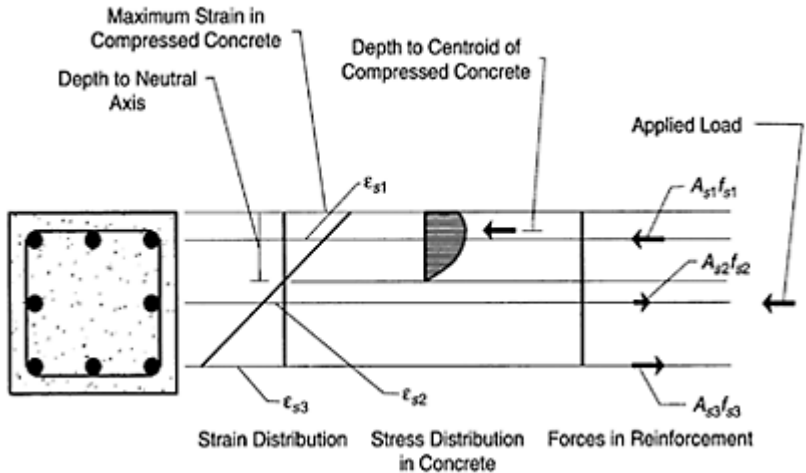
FIGURE 13.11 Assumed strain, stress and force distributions.
