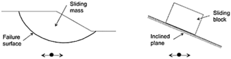
FIGURE 4.43 Analogy between (a) potential seismically induced landslide and (b) rigid block resting on inclined plane.
