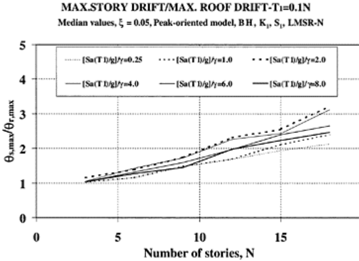
FIGURE 9.13 Median ratio of maximum story drift angle to maximum roof drift angle. (Medina, R.A. (2002). Seismic demands of nondeteriorating frame structures and their dependence on ground motions. Ph.D. Dissertation, Dept. of Civil Engineering, Stanford University. With permission.)
