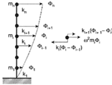
FIGURE 8.5 Mathematical model of the building.
