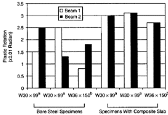
FIGURE 15.17 Plastic rotation capacities of NIST/AISC two-sided beam-to-column subassemblies (a: from Civjan and Engelhardt, 1998; b: from Uang et al., 2000).
