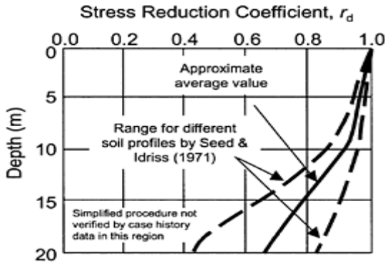
FIGURE 4.27 Variation of depth reduction factor, r_d , for simplified cyclic stress method. (Modified from Youd, T.L. et al. J. Geotech. Geoenviron. Eng. , ASCE, 127, 817–833, 2001. With permission.)
