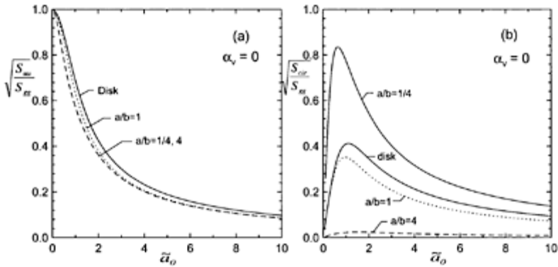
FIGURE 4.22 Amplitude of transfer function between free-field motion and FIM for vertically incident incoherent waves (Veletsos and Prasad, 1989; Veletsos et al, 1997).
