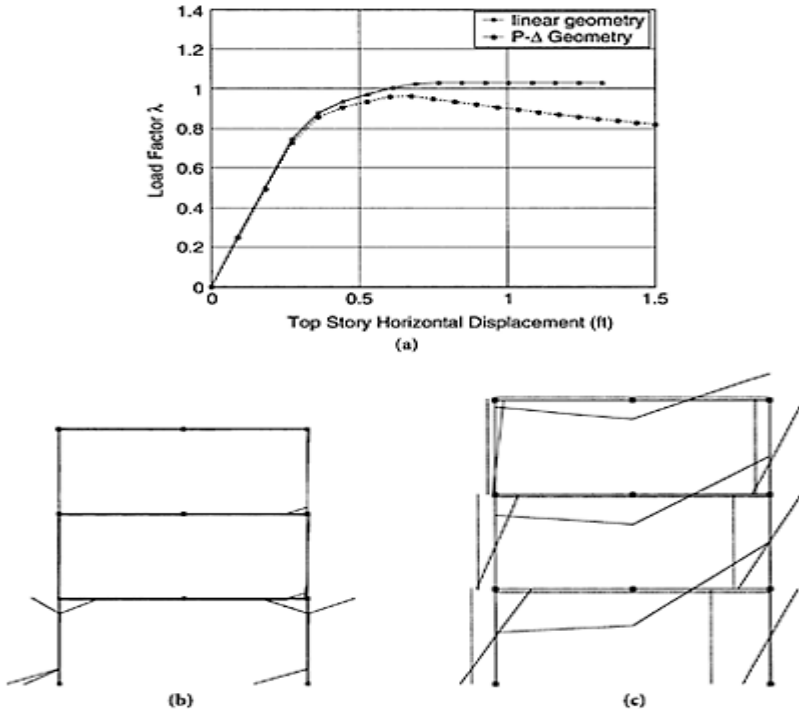
FIGURE 6.25 (a) Load factor-top story displacement relation for three-story steel frame; distributed inelasticity element with force formulation and five control sections; layer section with 20 layers, (b)
