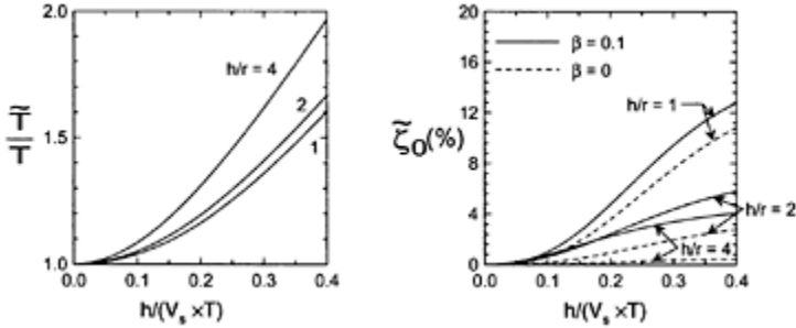
FIGURE 4.19 Period lengthening ratio and foundation damping factor for single degree-of-freedom structure with rigid circular foundation on viscoelastic halfspace ( \nu=0.4 , \gamma_m=0.15 ).
