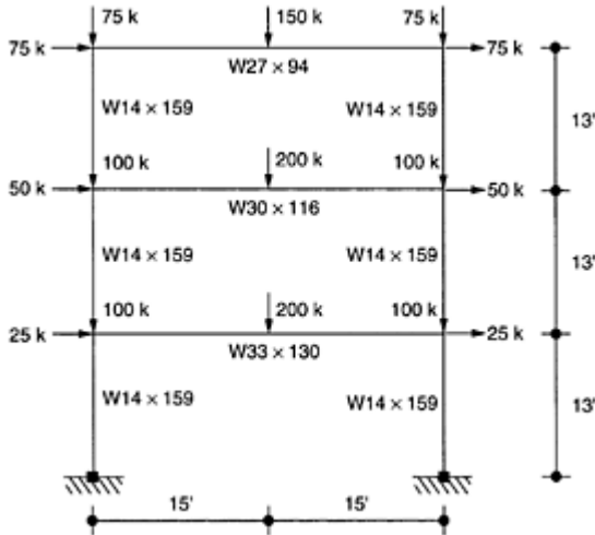
FIGURE 6.23 Geometry, member sizes and reference loading for three-story, one-bay steel frame.
