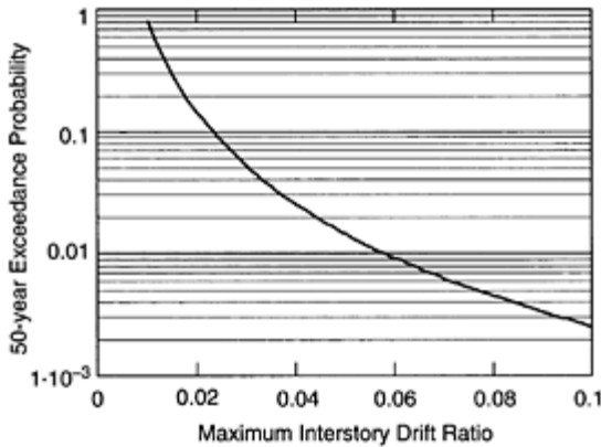
FIGURE 7.3 Fifty-year maximum interstory drift ratio demand curve.
