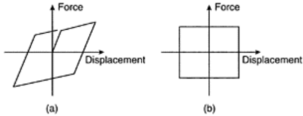
FIGURE 12.1 Force-displacement relations for hysteretic dampers.
