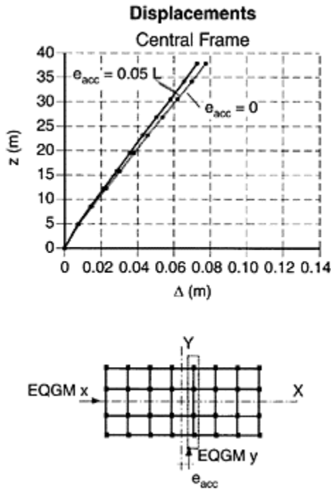
FIGURE 8.37 3D linear elastic response spectrum analysis of central frame (Y displacements).
