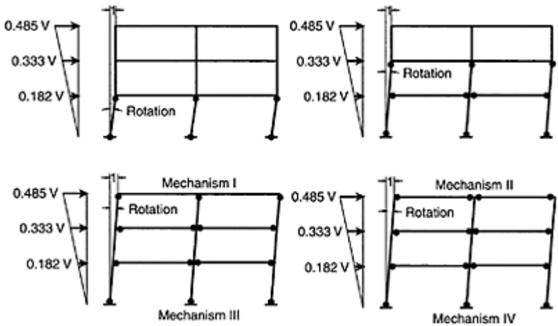
FIGURE 13.14 Mechanisms assumed to determine base shear strength.
