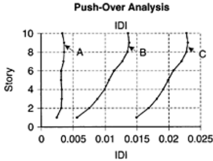
FIGURE 8.46 IDI for push-over analysis.
