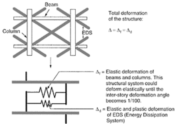
FIGURE 10.9 Structure with energy dissipating system.
