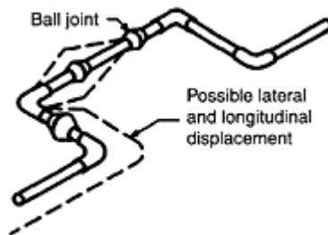
FIGURE 19.25 Possible arrangement to allow for relative deflections in
