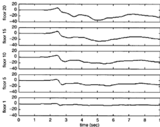
FIGURE 6.29 Displacement history (in inches) at five floor levels in 20-story building due to horizontal ground acceleration.
