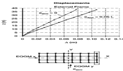
FIGURE 8.38 3D linear elastic response spectrum analysis external frame (Y displacements).
