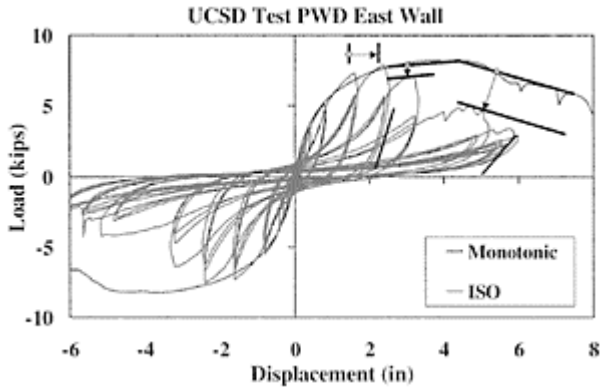
FIGURE 9.21 Experimental results from plywood shear wall tests; modes of deterioration (ISO=loading protocol of International Standards Organization).
