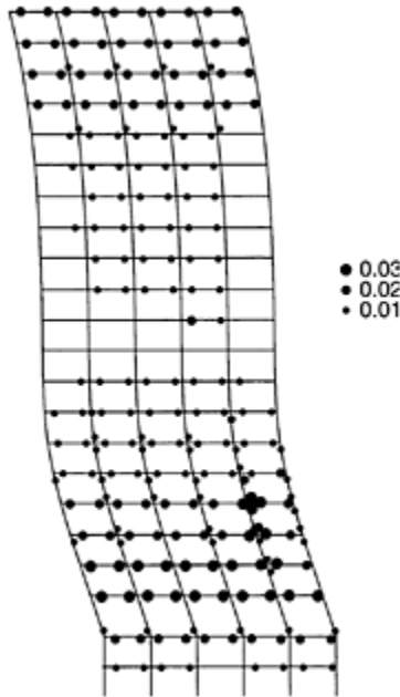
FIGURE 6.31 Maximum plastic hinge rotations in 20-story building due to horizontal ground motion. Deformed shape is the residual deformation after the earthquake (magnified by 20).
