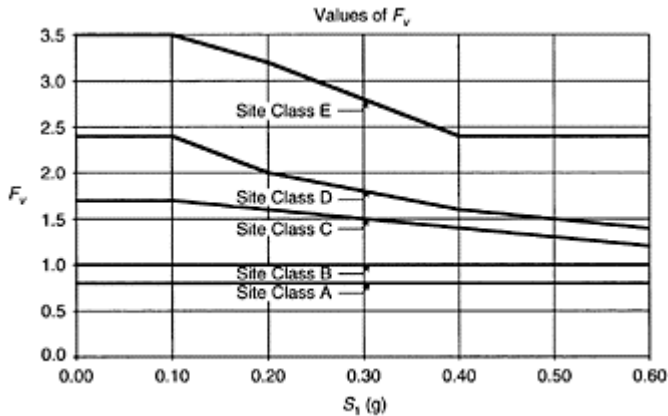
FIGURE 14.8 Values of F_v as a function of site class and S_1 .
