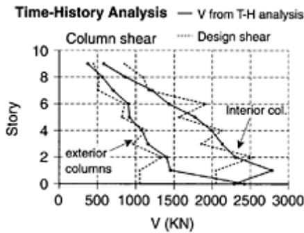
FIGURE 8.59 Time-history and design column shear.
