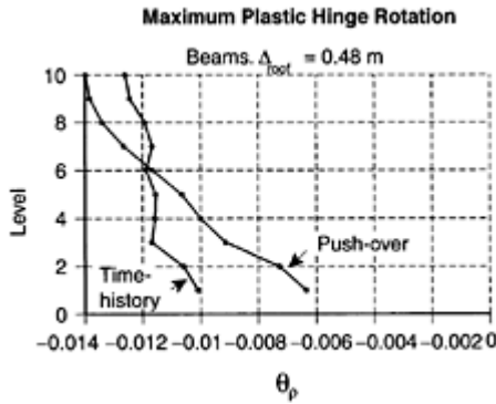
FIGURE 8.57 Comparison of maximum plastic hinge rotation from time-history and push-over analysis (equal \Delta_{roof} ).
