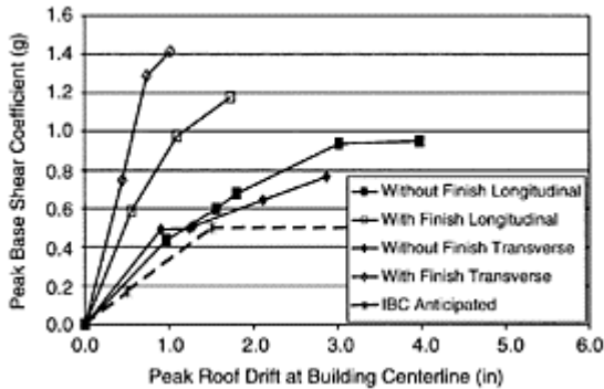
FIGURE 18.20 Load-deflection behavior for UC Berkeley apartment building. Phase I is configuration with no finish materials, Phase III is configuration with finish materials. No failures were observed. Curves end at stop of testing. (From Cobeen et al, 2003, CUREE Publication W-30, CUREE, Richmond, CA. With permission.)
