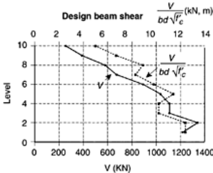
FIGURE 8.27 Shear and normalized shear stress for beams.
