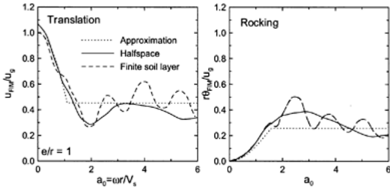
FIGURE 4.24 Transfer function amplitudes for embedded cylinders. (Day, 1978; Elsabee and Morray, 1977).
