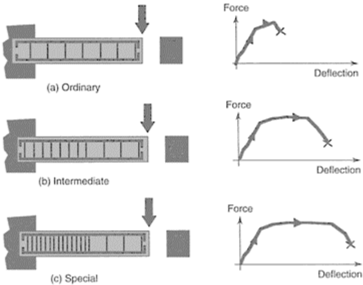
FIGURE 14.1 Force-deflection behavior of a reinforced concrete member having varying degrees of toughness.
