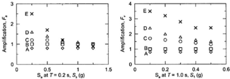
FIGURE 4.8 Site factors F_a and F_v given in NEHRP provisions (BSSC, 2001).
