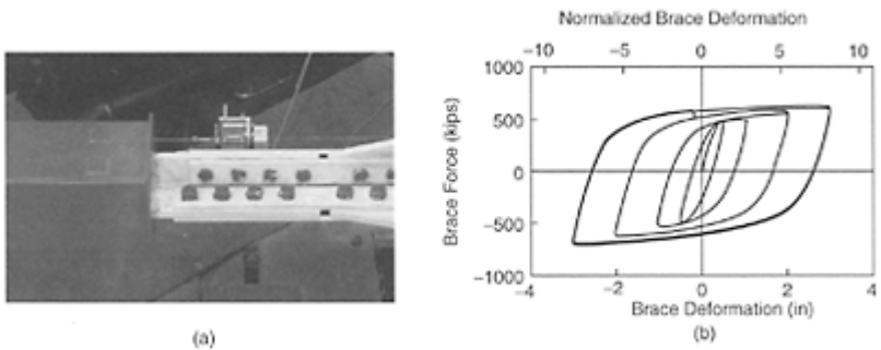
FIGURE 16.29 End details and typical hysteresis response, (a) End details; (b) hysteresis response. (Courtesy of Associated Bracing, Inc.)
