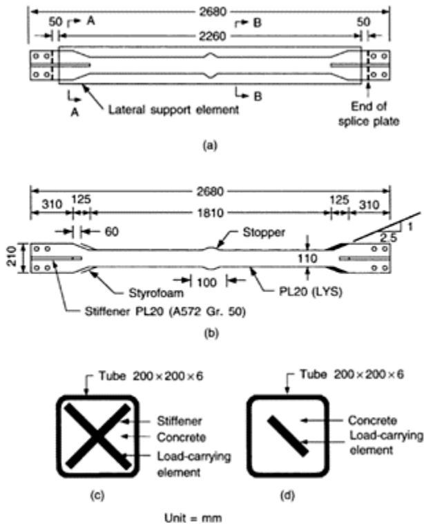
FIGURE 16.30 Details of buckling-inhibiting brace, (a) Overall view; (b) load-carrying element; (c) A-A section; (d) B-B section. (Chen, C.C., Chen, S.Y. and Liaw, J.J. (2001a). Application of low yield strength steel on controlled plastification ductile concentrically braced frames, Canadian Journal of Civil Engineering , 28, 823–836.)
