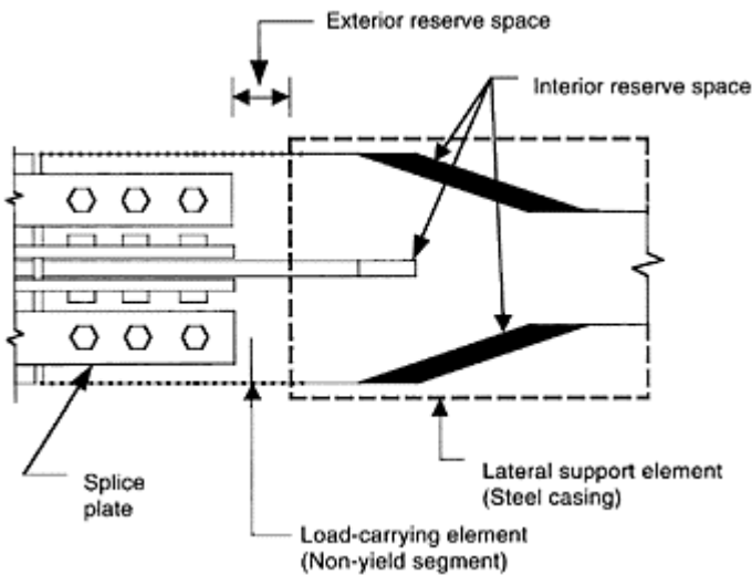
FIGURE 16.12 Gap between mortar and restrained yielding
