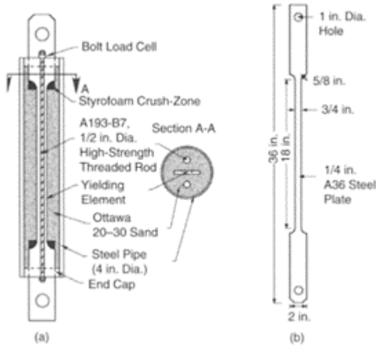
FIGURE 16.25 Composite confined hysteretic damper, (a) Test specimen; (b) steel core. (Higgins, C. and Newell, J. (2002).
