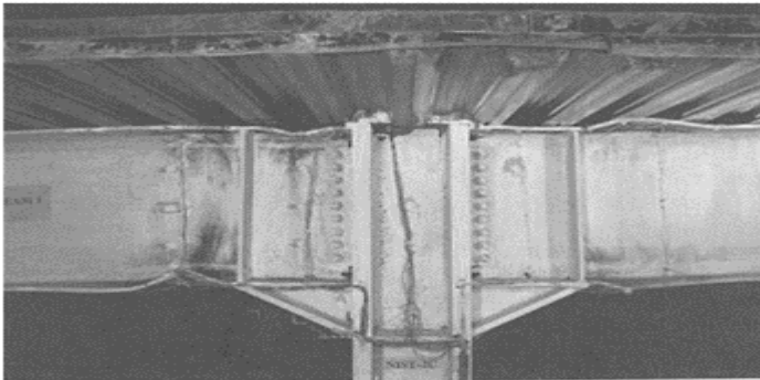
FIGURE 15.15 Buckling and yielding modes of composite welded haunch specimen (Yu, Q.-S.,
