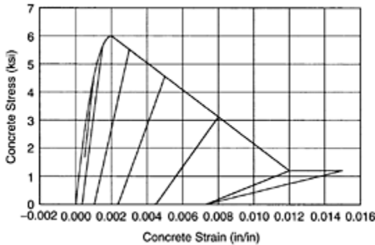
FIGURE 6.17 Hysteretic concrete stress-strain relation.
