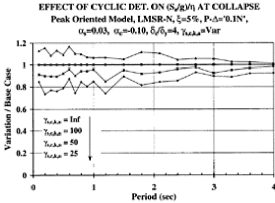
FIGURE 9.28 Effect of variation in cyclic deterioration on collapse capacity of base case. (Ibarra, L., Medina, R. and Krawinkler, H. (2002). Collapse assessment of deteriorating SDOF systems. Proc. 12th European Conference on Earthquake Engineering , London, Paper Reference 665. With permission.)
