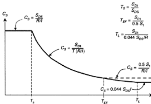
FIGURE 14.10 Seismic response coefficient, C_s , in the equivalent lateral force procedure.
