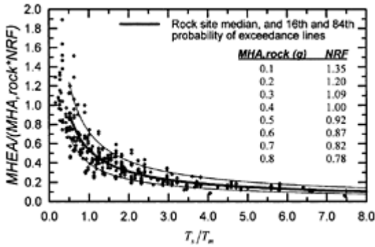
FIGURE 4.45 Normalized MHEA for deep-seated slide surface versus normalized fundamental period of slide mass (From Bray, J.D. and Rathje, E.M., J. Geotech. Geoenviron. Eng. , ASCE, 124. 242–253. 1998. With permission.)
