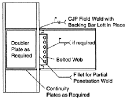
FIGURE 15.6 Pre-Northridge moment connection (FEMA 355D).
