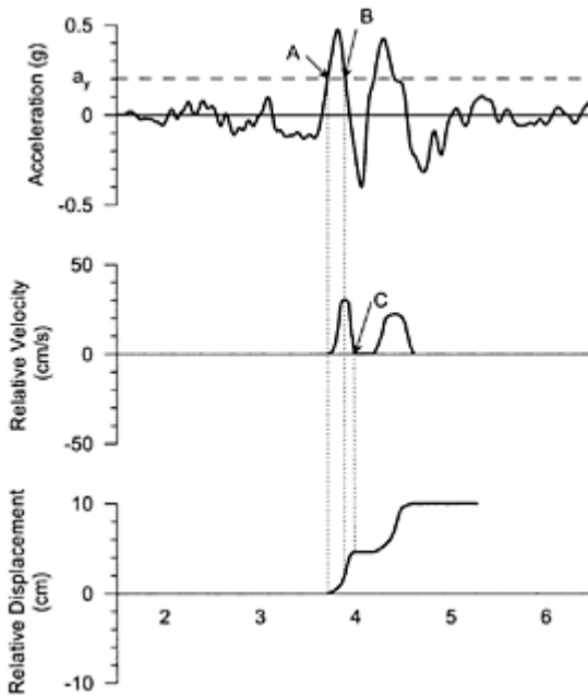
FIGURE 4.44 Development of permanent slope displacement for earthquake ground motion. (From Wilson, R.C. and Keefer, D.K., U.S. Geological Survey Professional Paper 1360, 317–345, 1985. With permission.)
