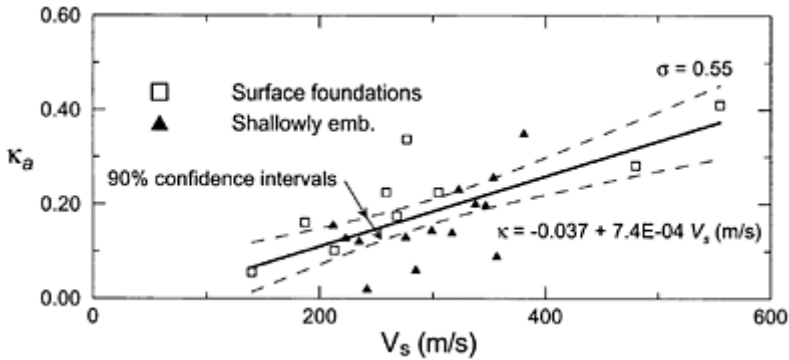
FIGURE 4.23 \kappa_a versus V_s results of linear regression. (From Kim, S. and Stewart, J.P., J. Geotech. Geoenviron. Eng. , ASCE, 129, 323–335, 2003. With permission.)
