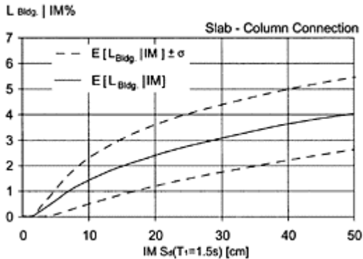
FIGURE 9.40 Variation of normalized losses in the building due to damage to slab-to-column connections as a function of the ground motion intensity.
