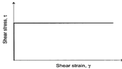
FIGURE 4.38 Stress-strain curve for rigid-perfectly plastic material, which is the assumed condition in limit equilibrium slope stability analyses.
