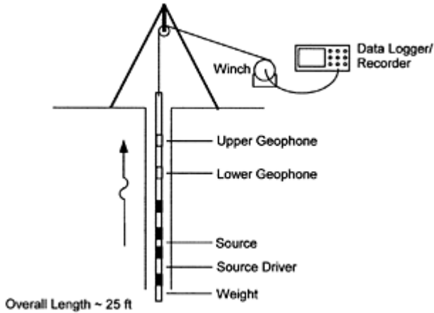
FIGURE 4.3 Schematic illustration of the suspension logger test.
