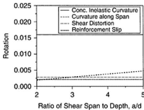
FIGURE 13.23 Relative contributions of rotation components.
