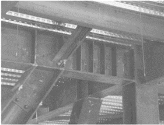
FIGURE 16.6 Typical link detail (courtesy of Structural Engineers, Inc.).
