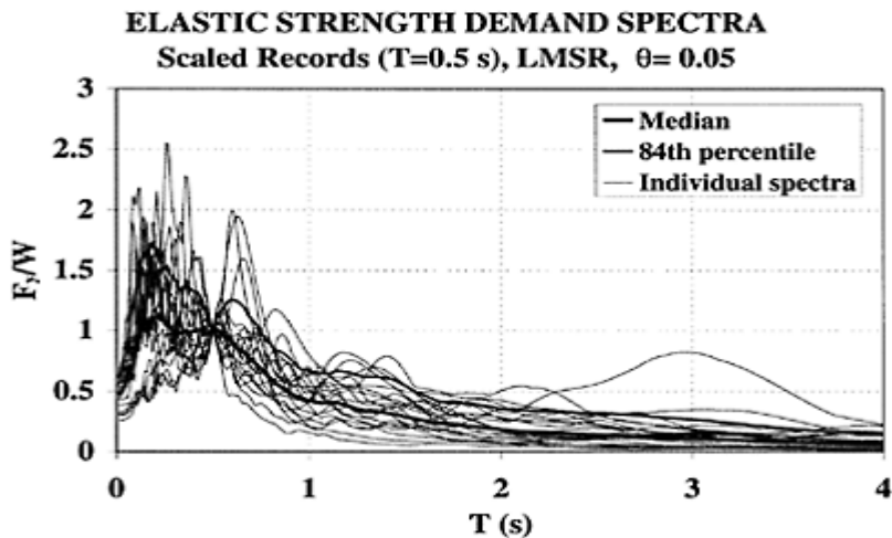
FIGURE 9.17 Set of ground motion spectra scaled to common S_a at T=0.5
