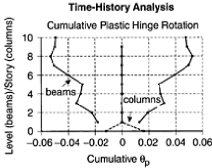
FIGURE 8.54 Cumulative plastic hinge rotation for time-history analysis.
