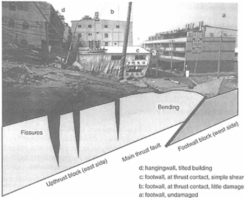
FIGURE 2.1 Damage effects of thrust faulting of the Chelungpu fault in the 1999 Chi-Chi, Taiwan, earthquake at Fengyuan. Damage was usually smaller on the footwall (western) side. (Courtesy National Center for Research on Earthquake Engineering, Taiwan.)
