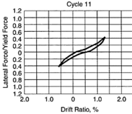
FIGURE 13.19K A force-displacement relationship in a cycle of applied displacement for the test frame in Figure 13.18.
