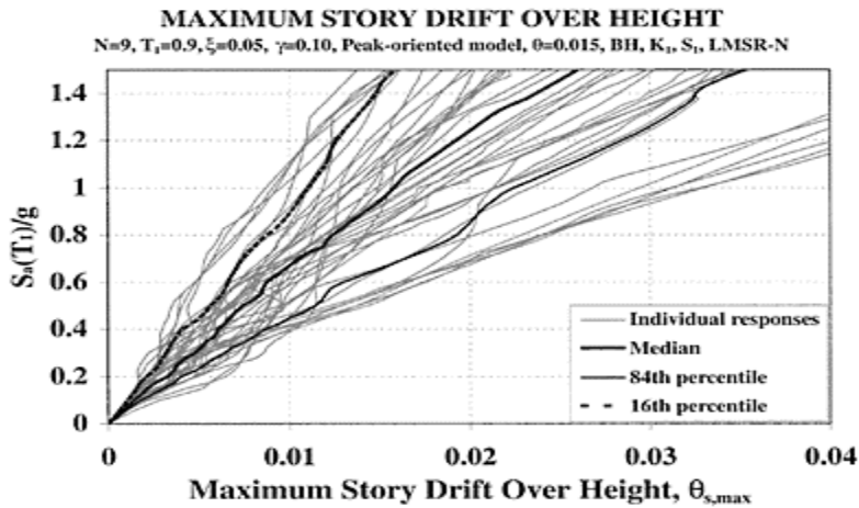
FIGURE 9.16 Record-to-record variability reflected in IDA curves for a nine-story frame structure with T_1=0.9 sec. (Medina, R.A. (2002). Seismic demands of nondeteriorating frame structures and their dependence on ground motions. Ph.D. Dissertation, Dept. of Civil Engineering, Stanford University. With permission.)
