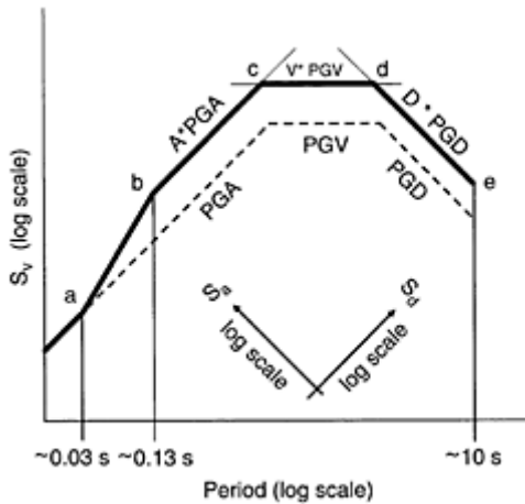
FIGURE 5.9 Elastic horizontal design spectrum according to Newmark and Hall. (Adapted from Chopra and Goel (2001). Direct displacement-based design: use of inelastic vs. elastic
