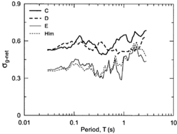
FIGURE 4.14 Variation with period of dispersion in ground response predictions associated with factors other than the ground response model estimation error for NEHRP Categories C-E and Holocene lacustrine/marine sediments (Him). (From Baturay, M.B. and Stewart, J.P. Bull Seism. Soc. Am. , 93, 2025–2042, 2003. With permission.)
