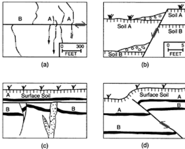
FIGURE 3.2 Geological evidence for paleo-earthquakes. (a) Map of intermittent streams (dot-line pattern) crossing San Andreas fault in Carrizo Plain, California. Streams labeled A
