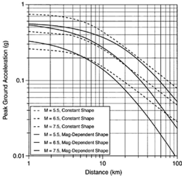
FIGURE 2.14 Comparison of constant and magnitude dependent shapes of attenuation relations.
