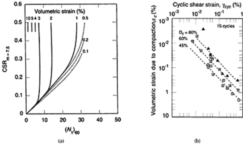
FIGURE 4.34 (a) Estimation of volumetric strain from liquefaction from CSR_m=7.5 and SPT penetration resistance and (b) volumetric strain from seismic compression as function of shear strain amplitude and relative density. (From Tokimatsu, K. and Seed, H.B., J. Geotech. Engrg. , ASCE, 113, 861–878, 1987. With permission).
