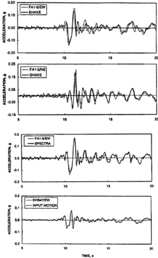
FIGURE 4.13 Comparison of recorded ground surface accelerations and predictions by SHAKE (top two frames) and SPECTRA (third frame from top). Bottom frame shows recording at base of array (47-m
