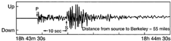
FIGURE 2.6 Seismogram at Berkeley, California, from a magnitude 5.3 earthquake located 90 km away, northeast of Santa Cruz on 27 June 1988. This recording of the vertical component of ground motion clearly shows the separate onsets of the P and S waves. Time increases on the trace from left to right.
