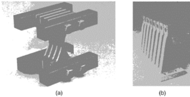
FIGURE 12.4 Examples of metallic yielding dampers, (a) Added damping and stiffness (ADAS) element; (b) triangular ADAS element (TADAS).
