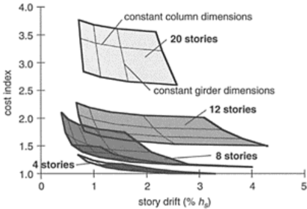
FIGURE 14.45 Relationship of cost of columns and girders against story drift for moment-resisting frame buildings studied in (Garcia, 1996).
