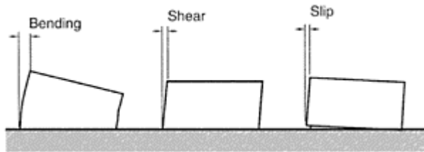
FIGURE 13.26 Idealized sources of deformation for a reinforced concrete wall.
