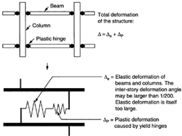
FIGURE 10.5 Strong column-weak beam model.
