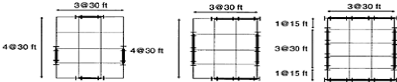
FIGURE 7.10 Plane of three-story, 1×1 bay, and 2×2 bay, and 3×3 bay moment frame systems with equal total lateral resistances.
