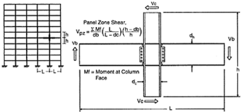
FIGURE 15.5 Calculation of panel zone shear (FEMA 355D).
