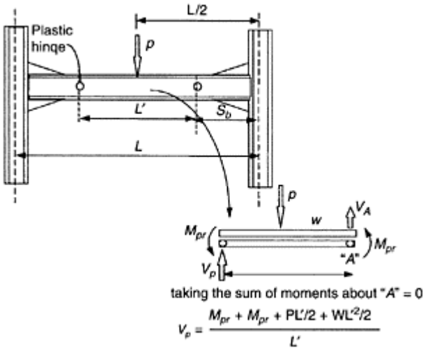
FIGURE 15.9 Sample calculation of shear at plastic hinge (FEMA 350).
