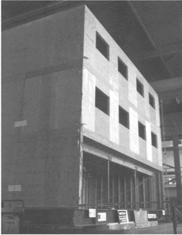
FIGURE 18.17 UC Berkeley apartment, Phase I without finishes. (From Mosalam, 2003, CUREE Publication W-19, CUREE, Richmond, CA. With permission.)
