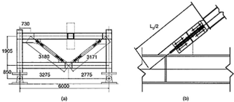
FIGURE 16.40 Geometry of subassembly test, (a) Geometry; (b) connection details. (Tsai, K.C., Hwang, Y.C., Weng, C.S., Shirai, T. and Nakamura, H. (2002), Experimental tests of large scale buckling restrained braces and frames, Proceedings, Passive Control Symposium , December 2002, Tokyo Institute of Technology, Tokyo, Japan.)
