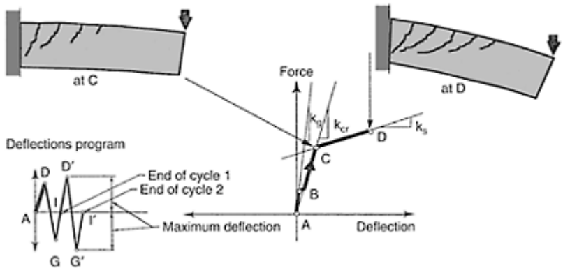
FIGURE 14.3 First quarter-cycle for example beam.
