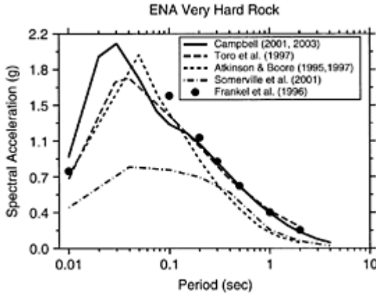
FIGURE 5.27 Comparison of 5%-damped pseudo-acceleration ( S_a ) response spectra predicted by the ENA ground motion relations listed in Table 5.4. The relations are evaluated for M_W=7 , r_{jb}=r_{rup}=10 km, r_{hypo}=14.1 km ( h_{hypo}=10 km), and very hard rock site conditions (see Tables 5.6 and 5.7). PGA is plotted at 0.01 sec period. The values of PGA and spectral acceleration predicted by the Frankel et al. (1996) relation are divided by the factors given in Table 5.5 to adjust them from firm rock to very hard rock site conditions. The Frankel et al. relation is plotted as single spectral ordinates to emphasize the lack of spectral ordinates below 0.1 sec.
