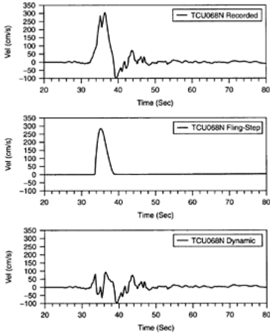
FIGURE 2.12 Velocity time histories for the north-south component of station TCU068 in the 1999 Chi-Chi earthquake (see Figure 2.9) separated into dynamic shaking and fling-step components.
