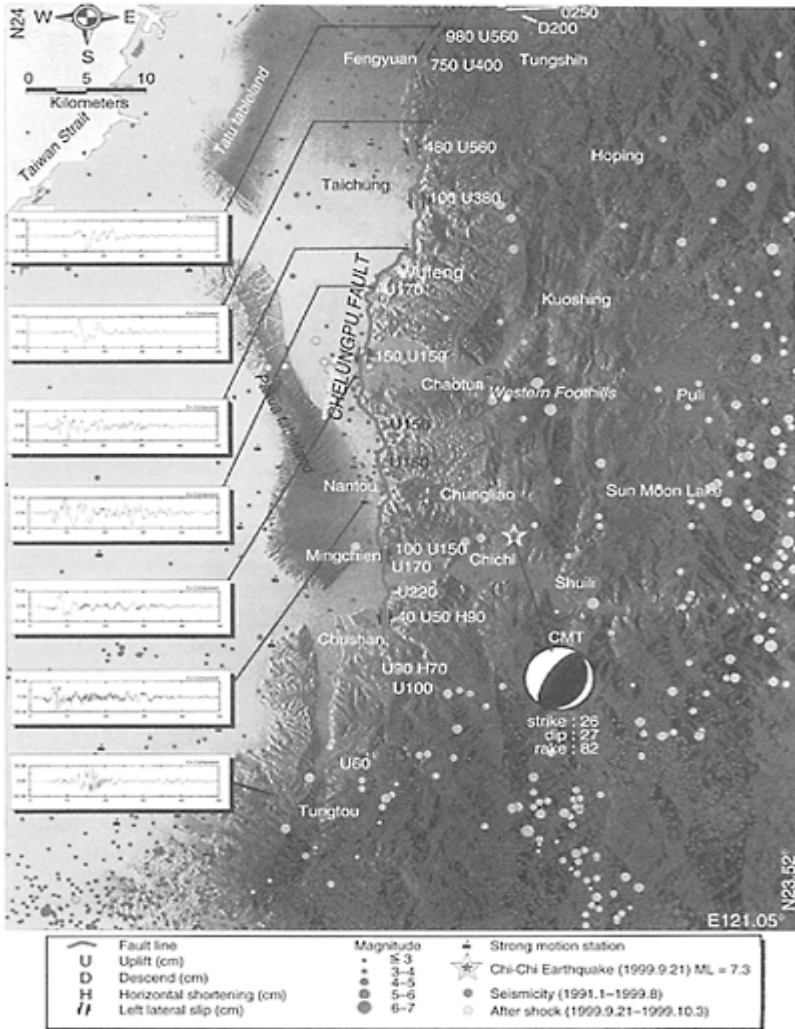
FIGURE 2.9 Relief map showing ruptured Chelengpu fault trace (red line), epicenter of aftershocks, ground displacement in centimeters and sample horizontal ground accelerations. Star is epicenter, circle is thrust mechanism (after Y.-B.Tsai). See also color insert following page 2–30.
