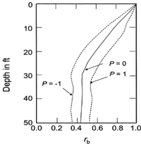
FIGURE 4.28 Variation of depth reduction factor, r_b , for Arias intensity method. Variable P represents number of standard deviations above mean value. (Modified from Kayen, R.E. and
