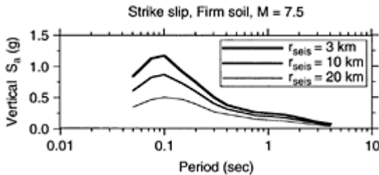
FIGURE 5.34 Median vertical acceleration response spectra for 5%
