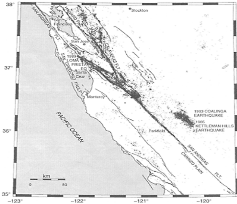
FIGURE 3.1 Seismicity of central California, 1980–1986, to compare the seismicity of that part of the San Andreas fault that ruptured in 1857 (Carrizo Plain, lower right corner), which is not imaged by earthquakes at all, to the seismicity of that part of the fault that ruptures frequently, as at Parkfield, or creeps accompanied by very small earthquakes (between Parkfield and Loma Prieta), which images the fault very well. That part of the fault crossing the San Francisco Peninsula ruptured in 1906, but is not
