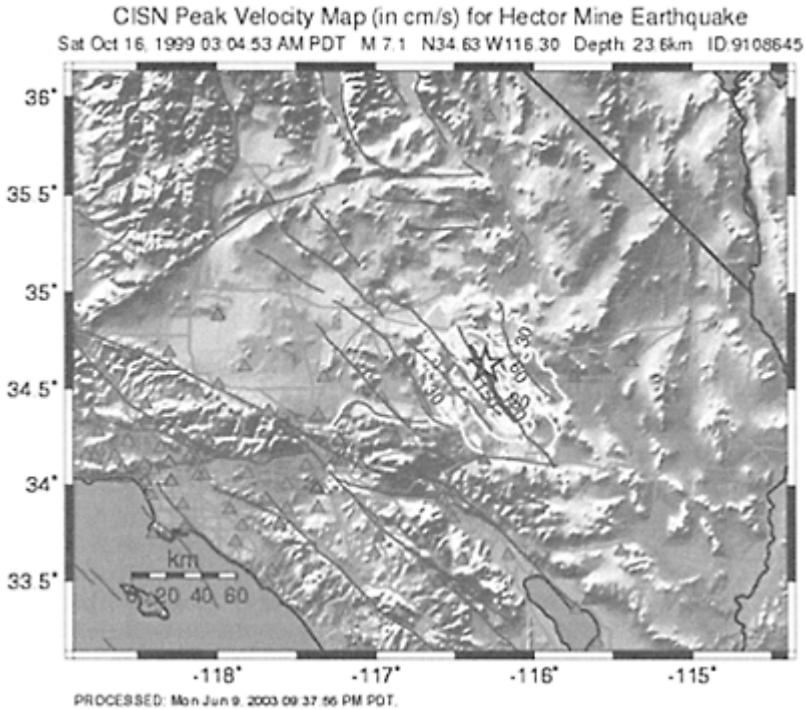
FIGURE 2.15 TriNet peak velocity map. See also color insert following page 2–30.
