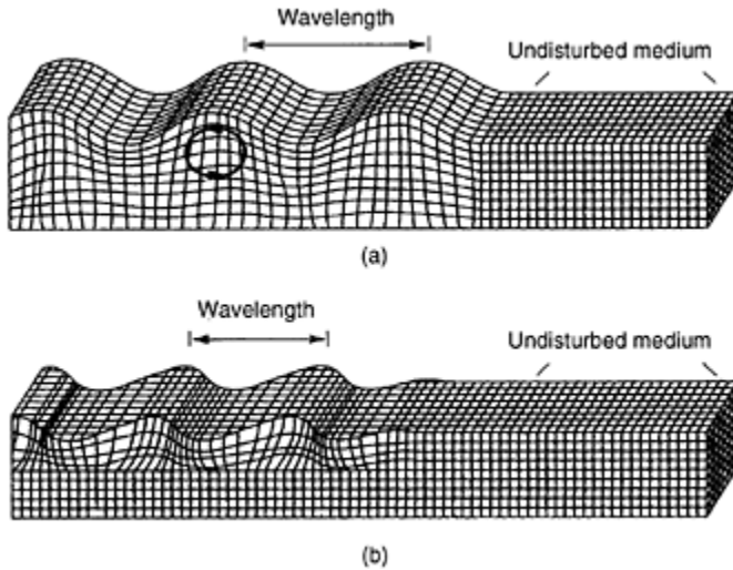
FIGURE 2.5 Deformations produced by surface waves: (a) Rayleigh wave (vertical motion); (b) Love wave (horizontal motion). (Bolt, B.A., 2003. Earthquakes . 5th ed., W.H. Freeman, New York. With permission).
