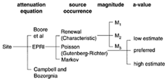
FIGURE 7.2 Logic tree in seismic hazard analysis.
