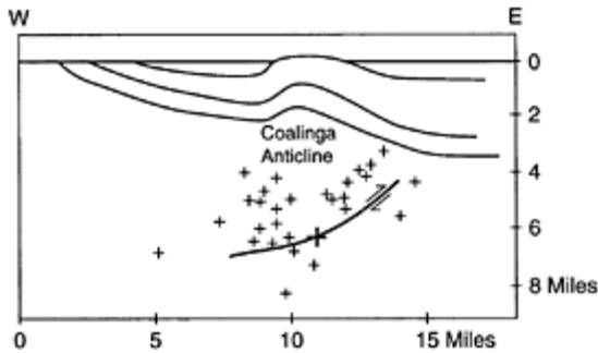
FIGURE 3.4 Cross section of the Coalinga, California, blind-thrust earthquake of May 2, 1983. Large plus symbol marks main shock; smaller plus symbols are aftershocks. Curved line is the fault plane based on modeling of surface deformation and on seismic-reflection profile. Layers above the main shock are bowed upward into an anticline. Based on work by R.S.Stein of the U.S. Geological Survey and G.C.P. King of the Institut de Physique du Globe de Paris.
