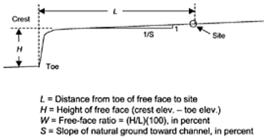
FIGURE 4.36 Illustration of variables used in Youd et al. (2002) lateral spreading model.
