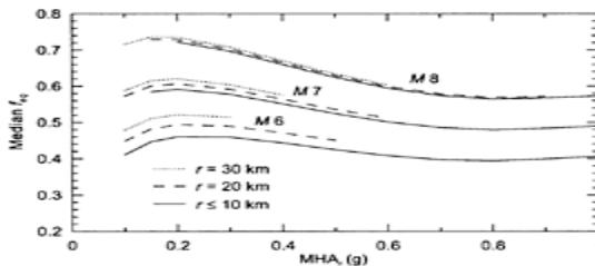
FIGURE 4.42 Relationship between f_{eq} ( = k/MHA_r ) as a function of MHA_r and seismological condition for slope displacement level of 5 cm. (From
