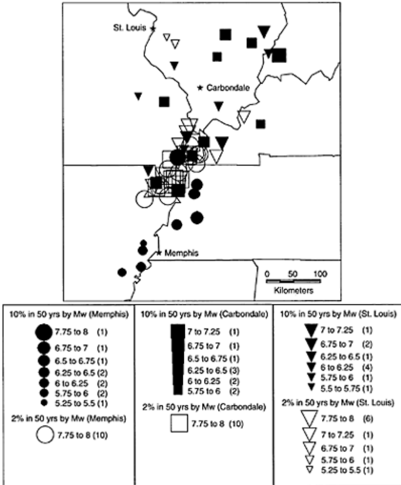
FIGURE 7.4 Epicenters and magnitudes of events contributing to uniform hazard ground motions for Memphis, Carbondale and St. Louis (number of events in the magnitude range is shown in the parentheses)
