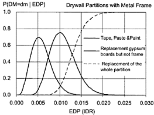
FIGURE 9.42 Probabilities of being in one of the three defined damage states in drywall partitions with metal frames.
