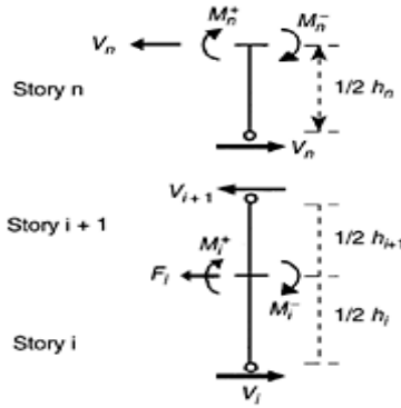
FIGURE 8.13 Approximated shear forces in columns (without considering the size of the joints).
