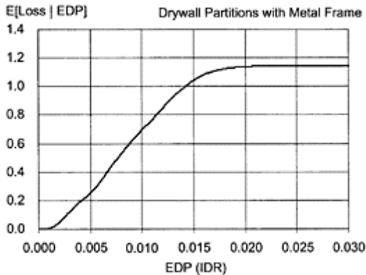
FIGURE 9.44 Variation of expected loss in partition walls as the interstory drift ratio increases.
