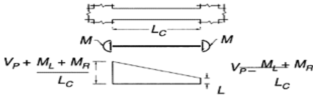
FIGURE 13.24 Shear force in a girder related to development of yield moments at column faces.
