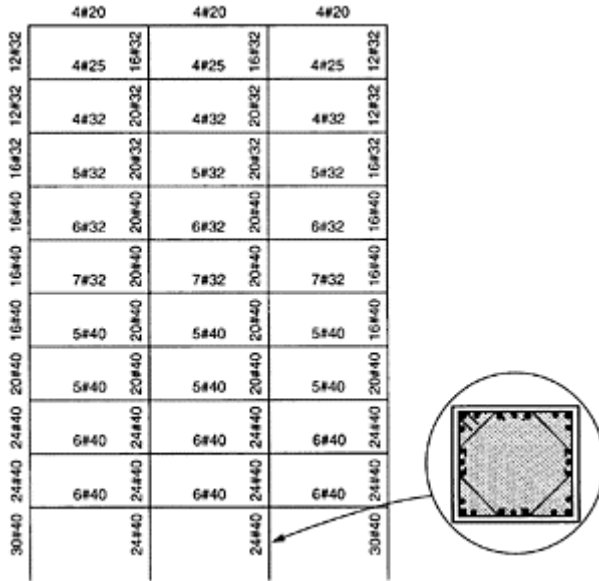
FIGURE 8.36 Preliminary design of main reinforcement for beams and columns (mm).
