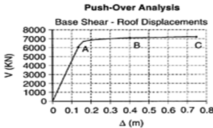
FIGURE 8.44 Base shear-roof displacement for push-over analysis of the external frame.
