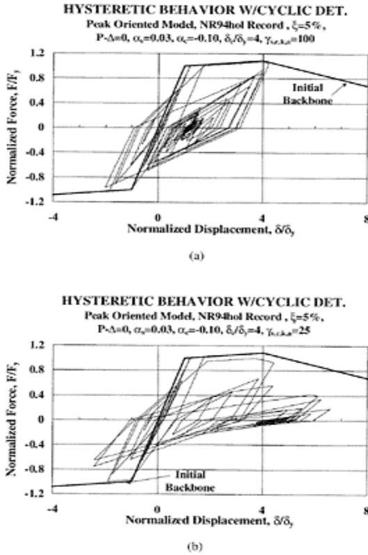
FIGURE 9.24 Effect of cyclic deterioration in time history analysis (a) \gamma_{s,c,k,a}=100 , (b) \gamma_{s,c,k,a}=25 . (Ibarra L. et al, Proc. 12th European Conference on Earthquake Engineering , London, 2002. With permission.)
