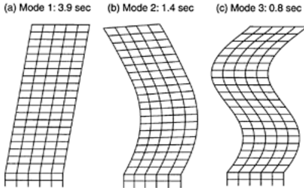
FIGURE 6.28 Lower three vibration modes and periods of 20-story building.
