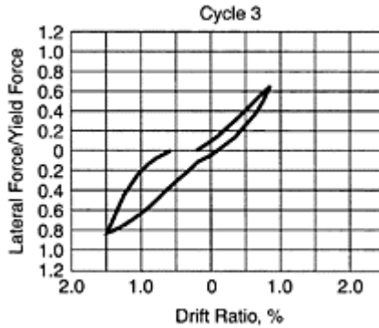
FIGURE 13.19C A force-displacement relationship in a cycle of applied displacement for the test frame in Figure 13.18.
