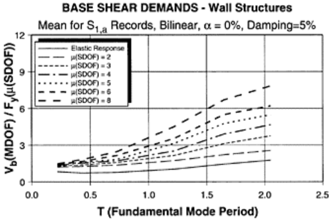
FIGURE 9.14 Amplification of base shear demand for wall structures. (Seneviratna, G.D.RK. and Krawinkler, H. (1997). Evaluation of inelastic MDOF effects for seismic design. John A.Blume Earthquake Engineering Center Report No. 120, Department of Civil Engineering, Stanford University. With permission.)
