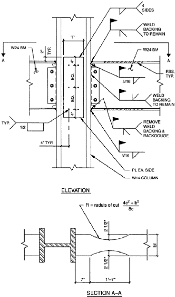
FIGURE 15.11 Example of RBS connection detail.
