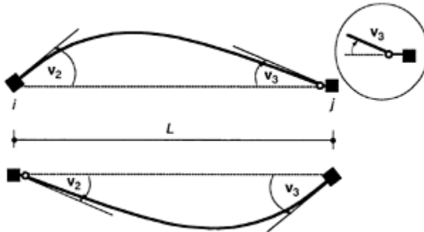
FIGURE 6.8 Flexural deformations for element with moment release.
