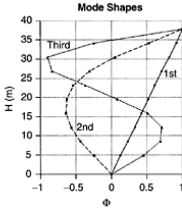
FIGURE 8.21 First three modes.
