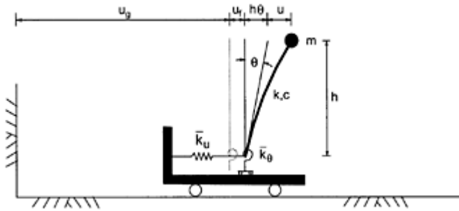
FIGURE 4.18 Simplified oscillator model for analysis of inertial interaction under lateral excitation.
