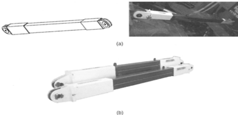
FIGURE 16.28 Star Seismic buckling-restrained brace . (a) Single-tube configuration; (b) multitube
