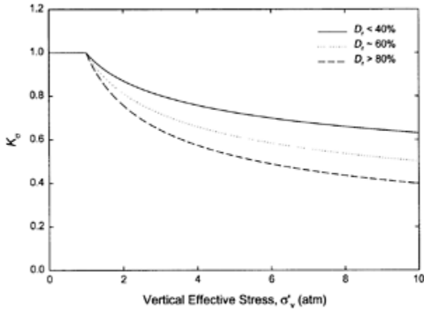
FIGURE 4.30 Variation of overburden correction factor, K_{\sigma} , with overburden pressure. (From Harder, L.F. and Boulanger, R.W., Proceedings, NCEER Workshop on Evaluation of Liquefaction Resistance of Soils , 167–190, 1997. With permission.)
