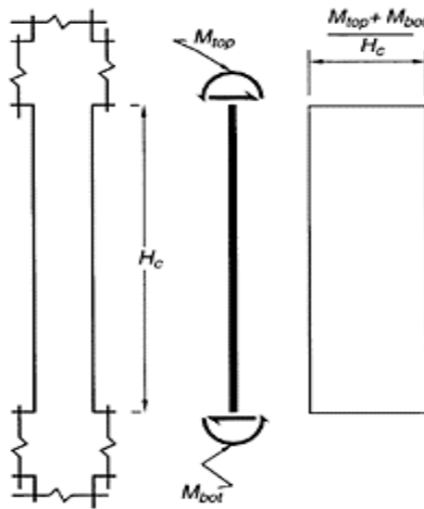
FIGURE 13.25 Shear force in a column related to development of yield moments at joints.
