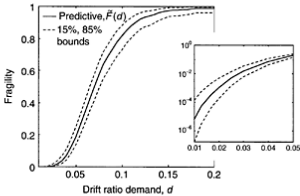
FIGURE 7.6 Conditional probabilistic of failure (fragility) of RC column against drift demand ( d ) shown in linear scale and log scale for d < 0.05 in small figure (Gardoni et al, J. Eng. Mech. , ASCE, 128, 1024–1038, 2002.).
