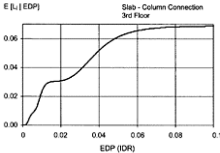
FIGURE 9.39 Variation of expected normalized building loss due to damage in slab-to-column connections as the interstory drift ratio increases.
