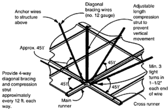
FIGURE 19.23 Seismic bracing system for suspended T-bar ceiling systems. (From Federal Emergency Management Agency, Reducing the Risks of Nonstructural Earthquake Damage, A Practical Guide , FEMA, Washington, D.C., 1994.)
