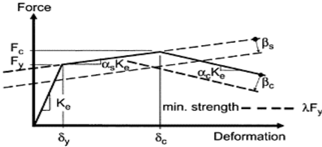
FIGURE 9.22 Backbone curve and its movement with deterioration.
