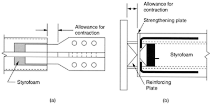
FIGURE 16.18 Buckling-restrained braces end details, (a) Fujimoto, M., Wada, A., Saeki, E., Watanabe, A. and Hitomi, Y. (1988). A study on the unbonded brace encased in buckling-restraining concrete and steel tube, Journal of Structural Engineering , 034B, 249–258 (in Japanese); (b) Nagao, N. and Takahashi, S. (1990). A study on the elastoplastic behavior of unbonded composite bracing (Part 1: experiments on isolated members under cyclic loading), Journal of Structural Engineering , 415, 105–115 (in Japanese).
