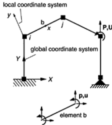
FIGURE 6.1 Local and global reference systems and notation.
