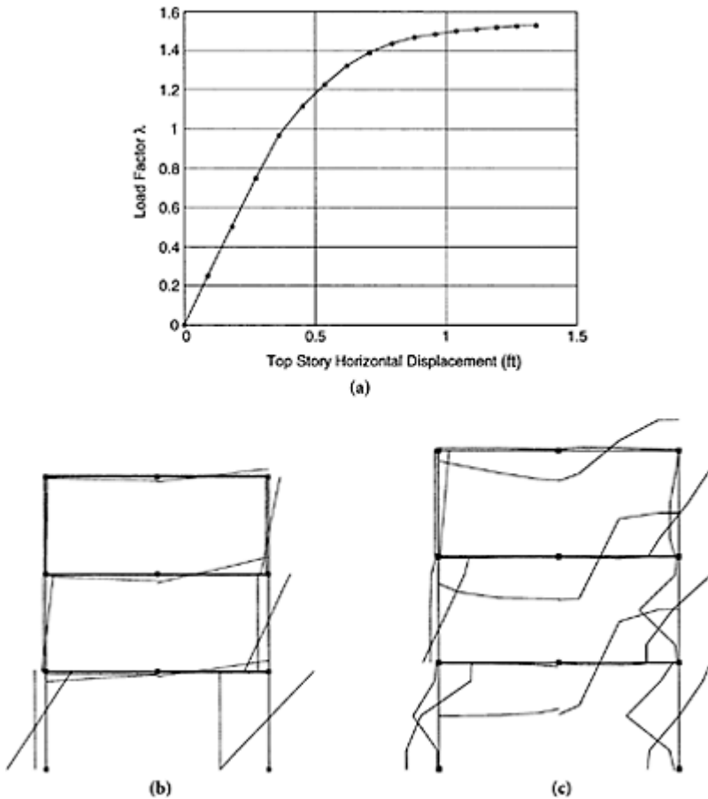
FIGURE 6.26 (a) Load factor-top story displacement relation for three-story steel frame under linear geometry; distributed inelasticity element with displacement formulation and five integration points; layer section with 20 layers, (b) Curvature (solid line) and axial strain (dashed line) distribution for three-story steel frame at maximum displacement;
