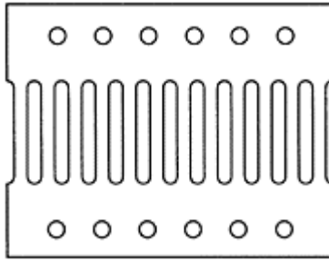
FIGURE 10.15 Details of the steel slit damper (SSD).
