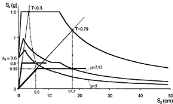
FIGURE 9.12 Two examples of direct use of inelastic spectra for estimating target displacement. (Fajfar, P., Earthquake Eng. Struct. Dyn. , 28, 979–993, 1999. With permission.)
