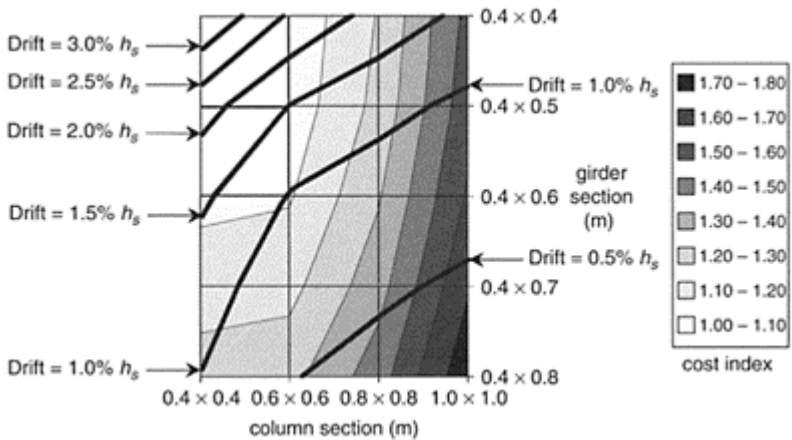
FIGURE 14.44 Maximum story drift and beam and column cost index for an eight-story moment-resistant frame building having the plan
