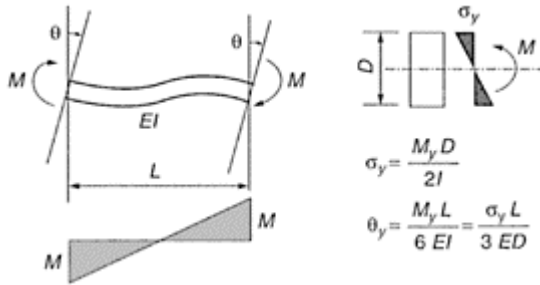
FIGURE 10.7 Deformation angle at beam ends of a rigid frame.
