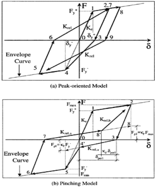
FIGURE 9.10 General load-deformation behavior of peak-oriented and pinching hysteretic models. (Medina, R.A. (2002). Seismic demands of nondeteriorating frame structures and their dependence on ground motions. Ph.D. Dissertation, Dept. of Civil Engineering, Stanford University. With permission.)
