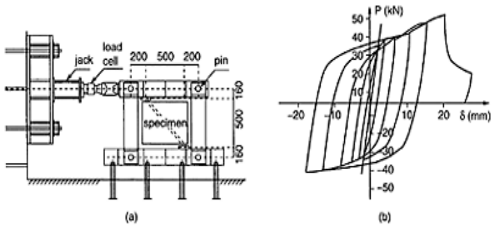
FIGURE 16.15 Subassemblage test of budding-restrained braces sandwiched between precast concrete panels (a) Test setup; (b) hysteresis behavior. (Wakabayashi,
