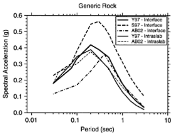
FIGURE 5.28 Comparison of 5%-damped pseudo-acceleration ( S_a ) response spectra predicted by the subduction-zone ground motion relations listed in Table 5.4. The
