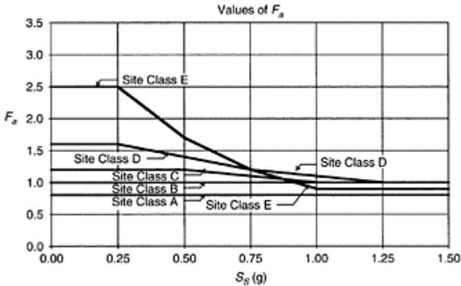
FIGURE 14.7 Values of F_a as a function of site class and S_s .
