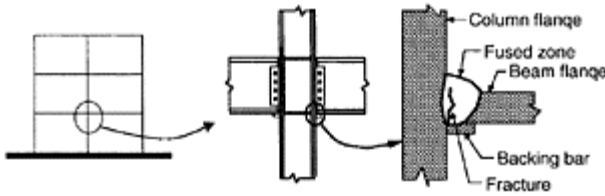
FIGURE 15.1 Common zone of fracture initiation in a typical beam-column connection.
