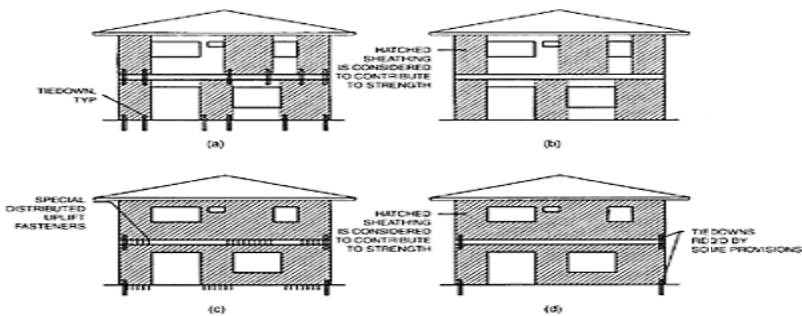
FIGURE 18.14 Diagram of shear wall types, (a)
