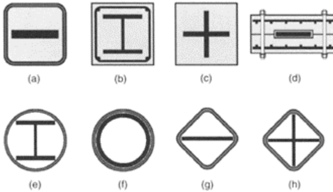
FIGURE 16.17 Cross sections of various budding-restrained braces developed in Japan.
