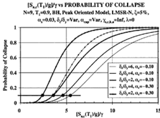
FIGURE 9.50 Collapse fragility curves for nine-story frames with T_1=0.9 sec; beams with various deterioration properties.
