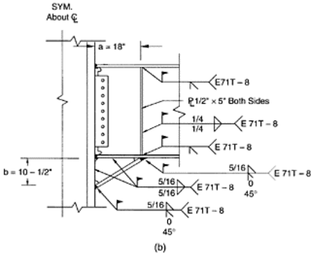
FIGURE 15.18 Haunch retrofit details.
