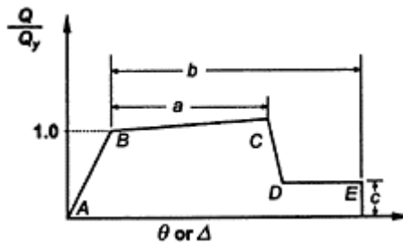
FIGURE 9.5 General force-deformation behavior of structural components. (FEMA 356 (2000). Prestandard and commentary for the seismic rehabilitation of buildings. U.S. Federal Emergency Management Agency.)
