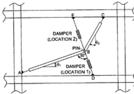
FIGURE 12.13 Toggle-brace assembly.
