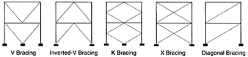
FIGURE 16.1 Examples of concentric bracing configurations (AISC (2002). Seismic Provisions for Structural Steel Buildings , American Institute of Steel Construction, Chicago, IL).
