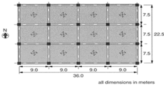
FIGURE 14.43 Plan layout for building studied in (Garcia, 1996).
