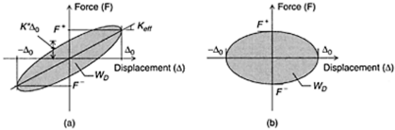
FIGURE 12.7 Parameter definition for velocity-dependent dampers, (a) Viscoelastic damper; (b) viscous damper.
