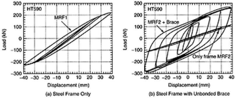
FIGURE 10.12 Hysteretic behavior of steel frames without and with unbonded brace, (a) Steel frame only; (b) steel frame with unbonded brace.
